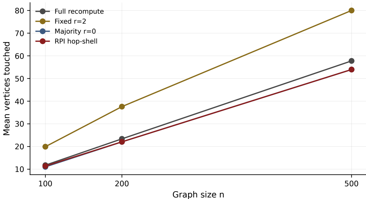
Holdout locality vs n (RPI \approx majority at n=200 and 500)
