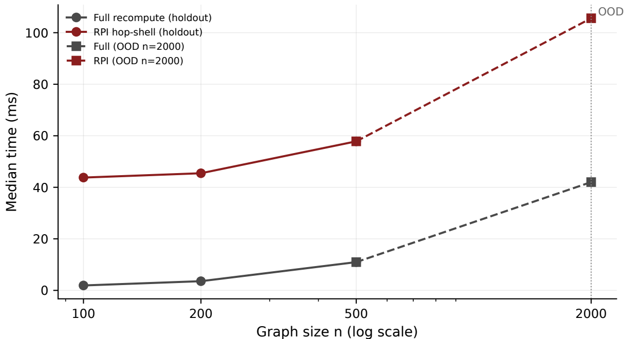
Median time vs n: OOD n=2000 is still slower for RPI
