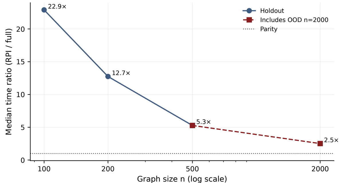
RPI/full median-time ratio shrinks with n but stays >1
