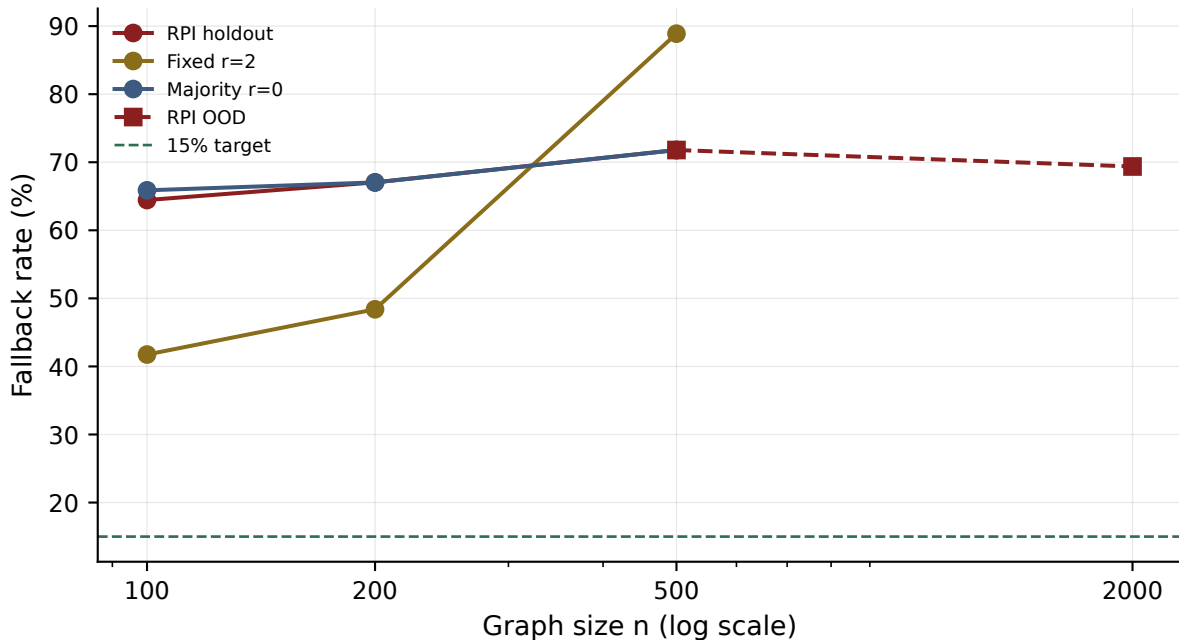
Fallback vs n (fixed/majority not run at n=2000)
