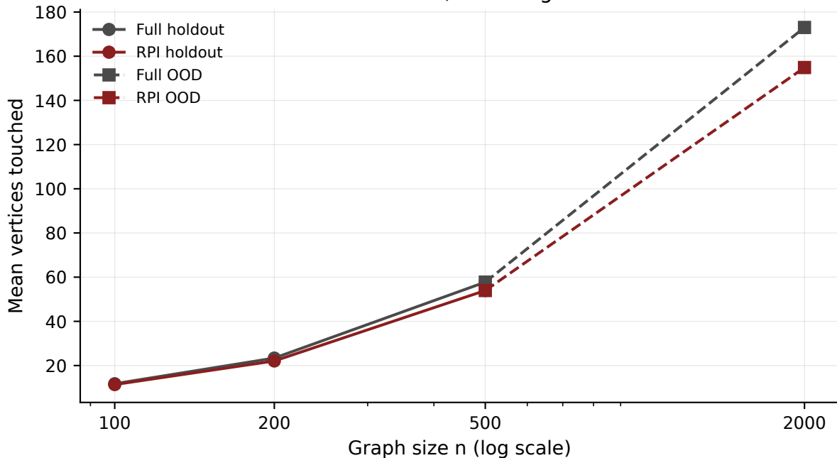
Vertices touched vs n, including OOD n=2000
