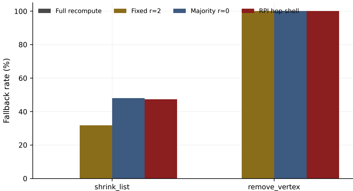
Fallback by edit type (holdout)
