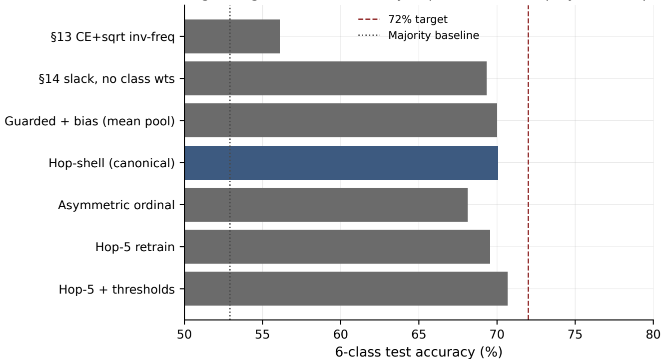
Training lineage (Context.md; only hop-shell is the deployed checkpoint)
