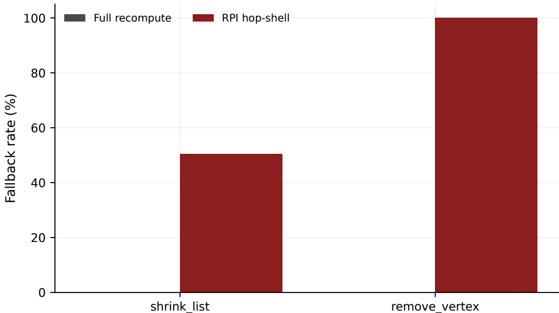
OOD n=2000 fallback by edit type (RPI vs full only)
