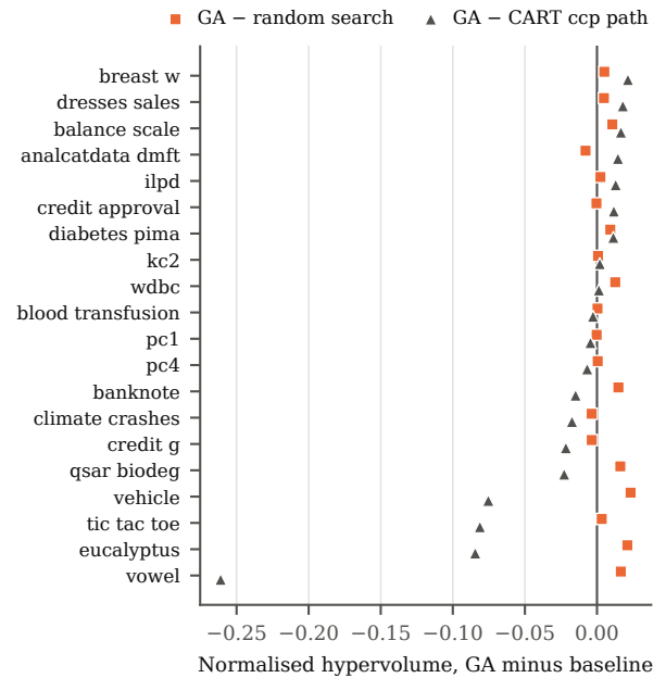
Figure 1: Per-dataset difference in normalised hypervolume between the GA and each baseline (mean over 30 outer folds). Right of zero favours the GA. Datasets sorted by the CART difference.
