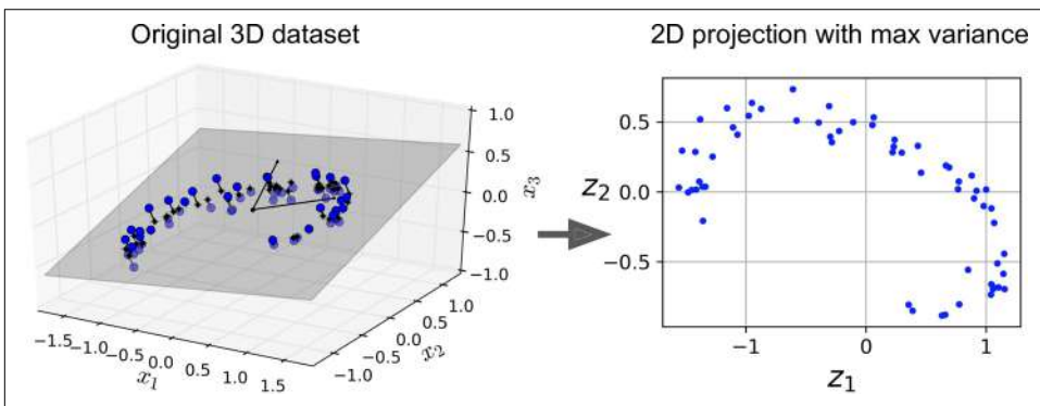
Figure 17-2. PCA performed by an undercomplete linear autoencoder
