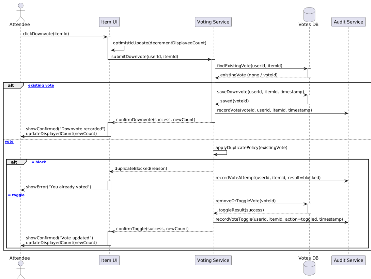
Figure 4.100 downvote sequence diagram
