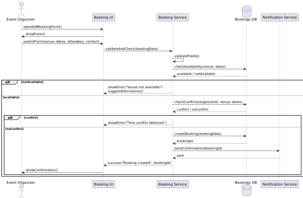
Figure 4.127 add booking (organizer) sequence diagram
