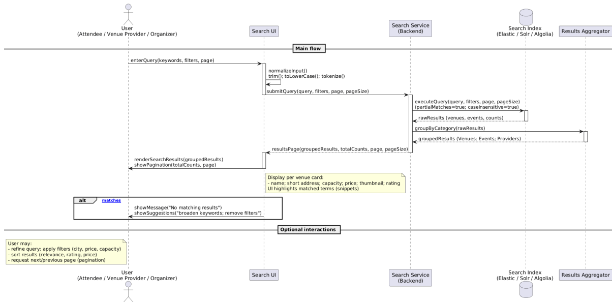
Figure 4.79 unified search for venues sequence diagram
