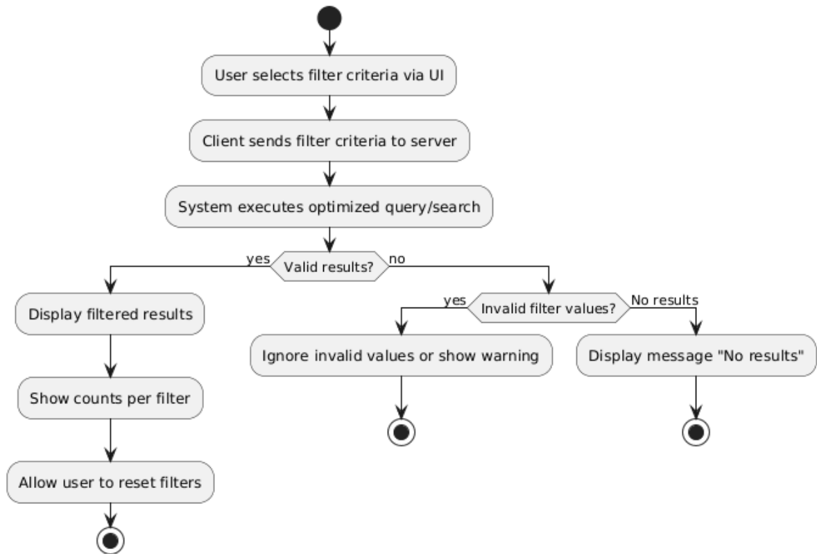
Figure 4.14 filter venues by specific criteria activity diagram
