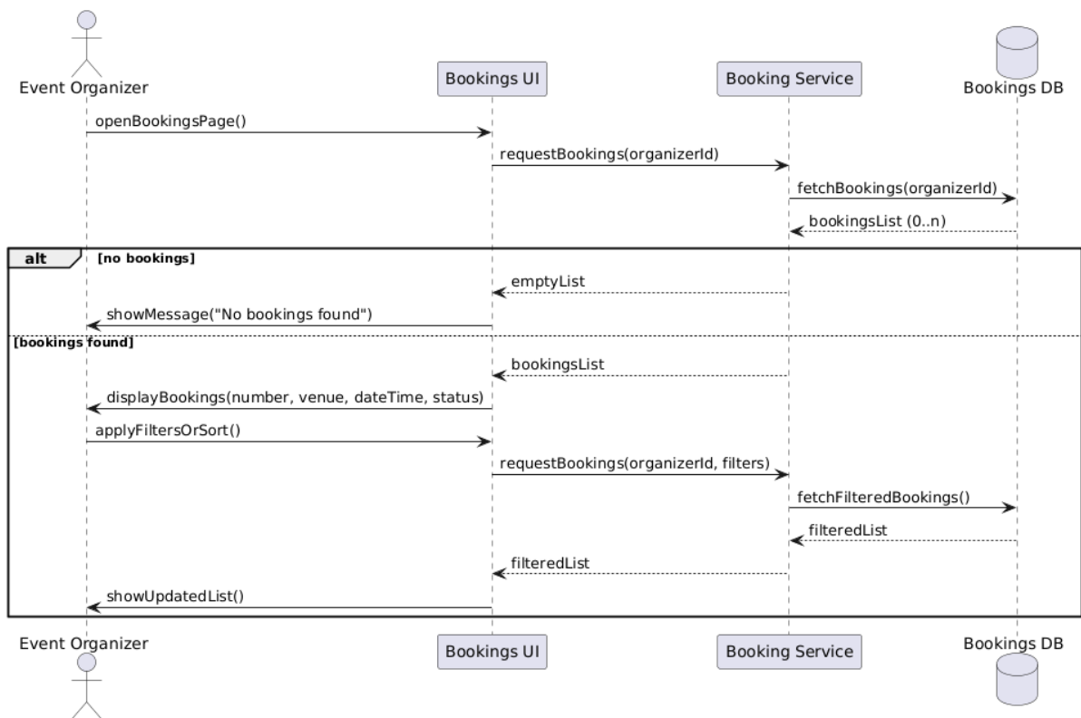
Figure 4.126 view booking (organizer) sequence diagram
