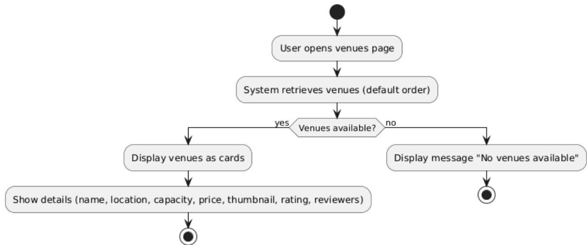
Figure 4.4 view venues activity diagram
