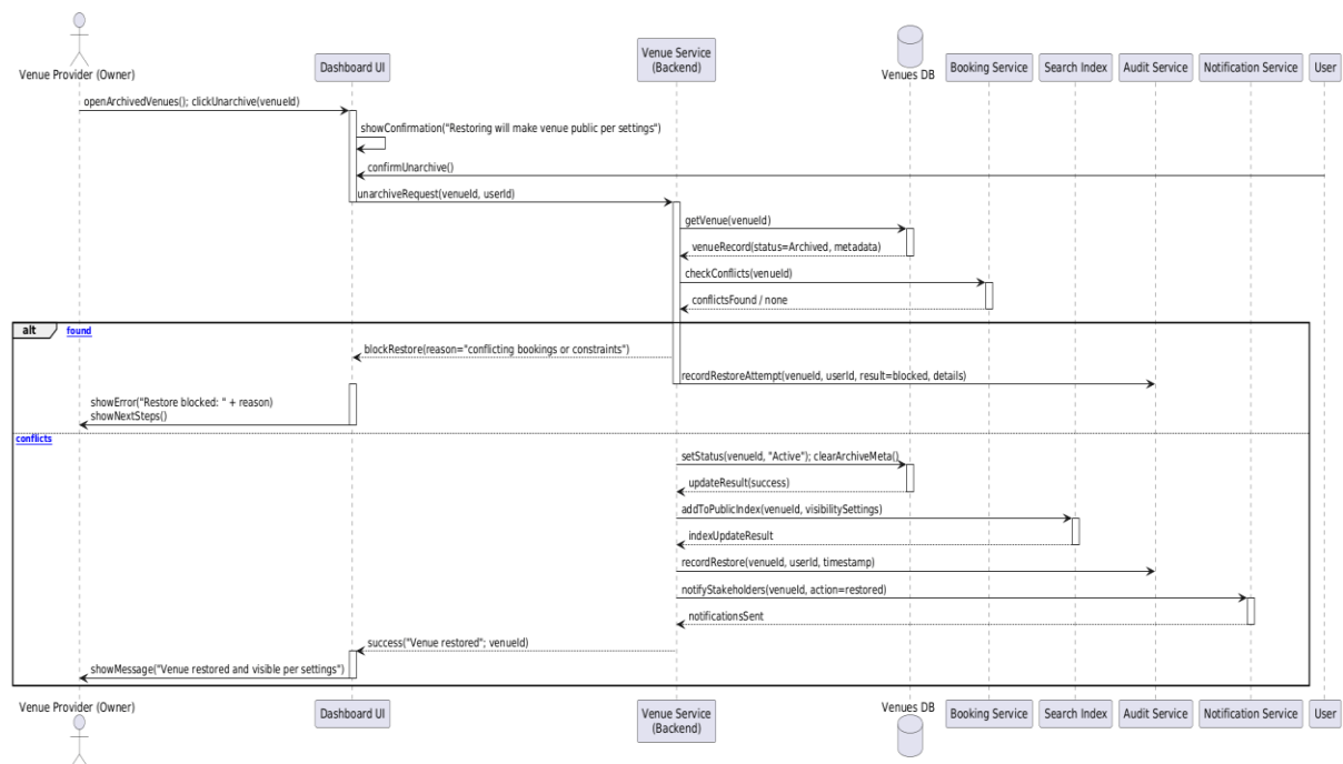
Figure 4.109 unarchive venue sequence diagram
