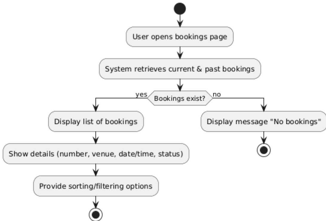
Figure 4.6 view bookings activity diagram
