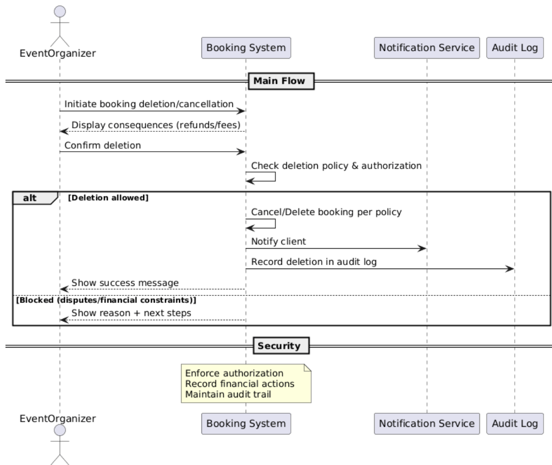
Figure 4.129 delete booking (organizer) sequence diagram
