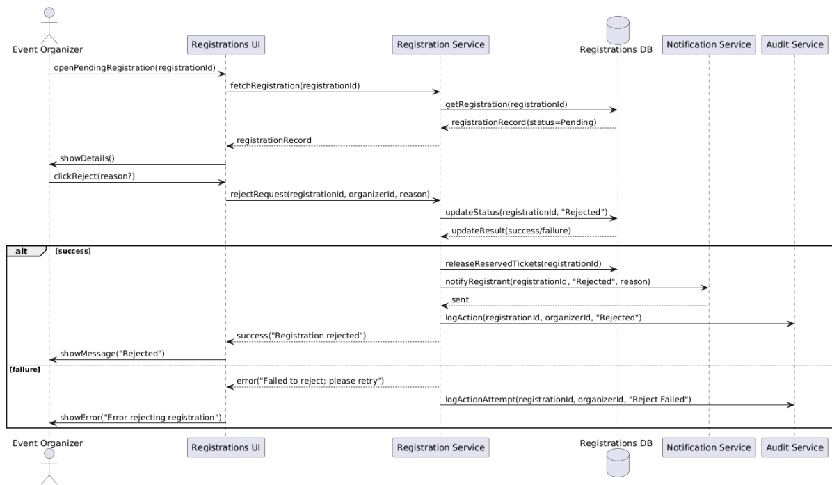
Figure 4.123 reject registration sequence diagram
