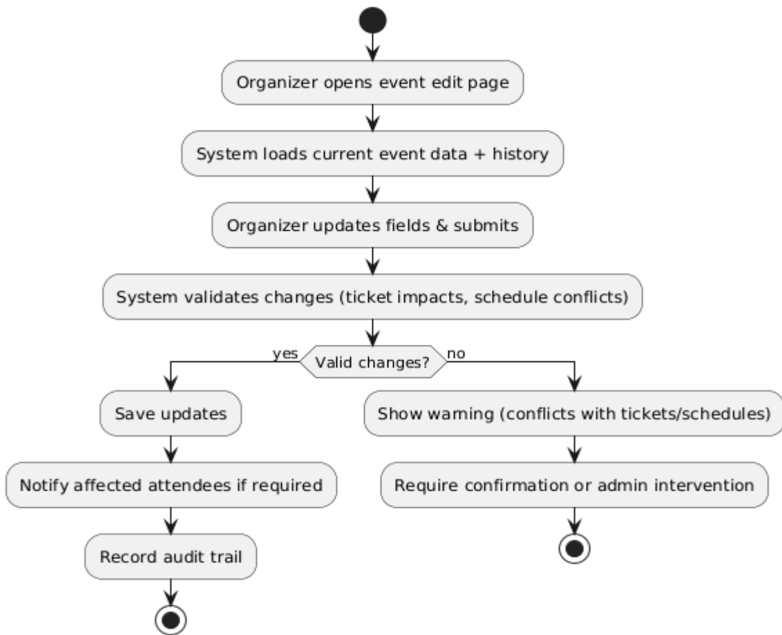
Figure 4.50 edit event activity diagram
