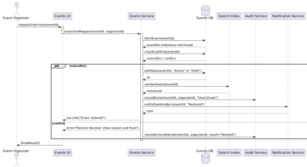
Figure 4.120 unarchive event sequence diagram
