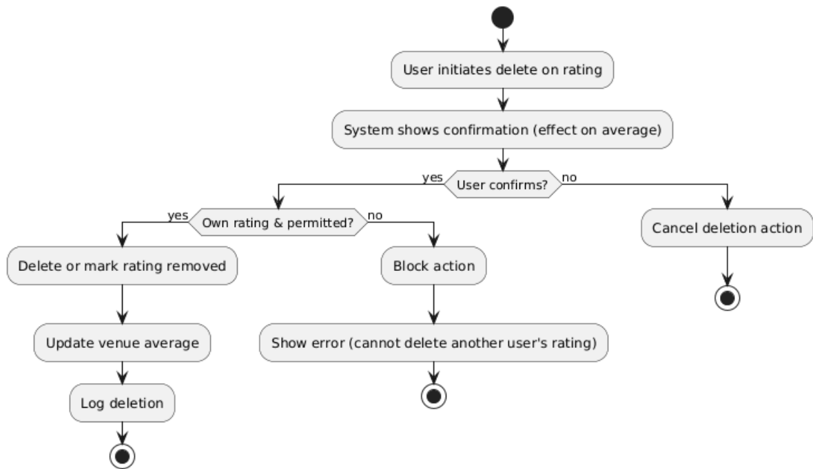
Figure 4.23 delete venue rating activity diagram
