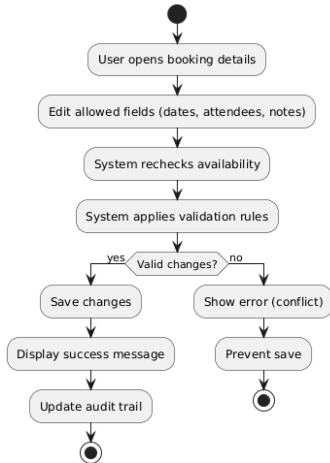
Figure 4.8 edit booking activity diagram
