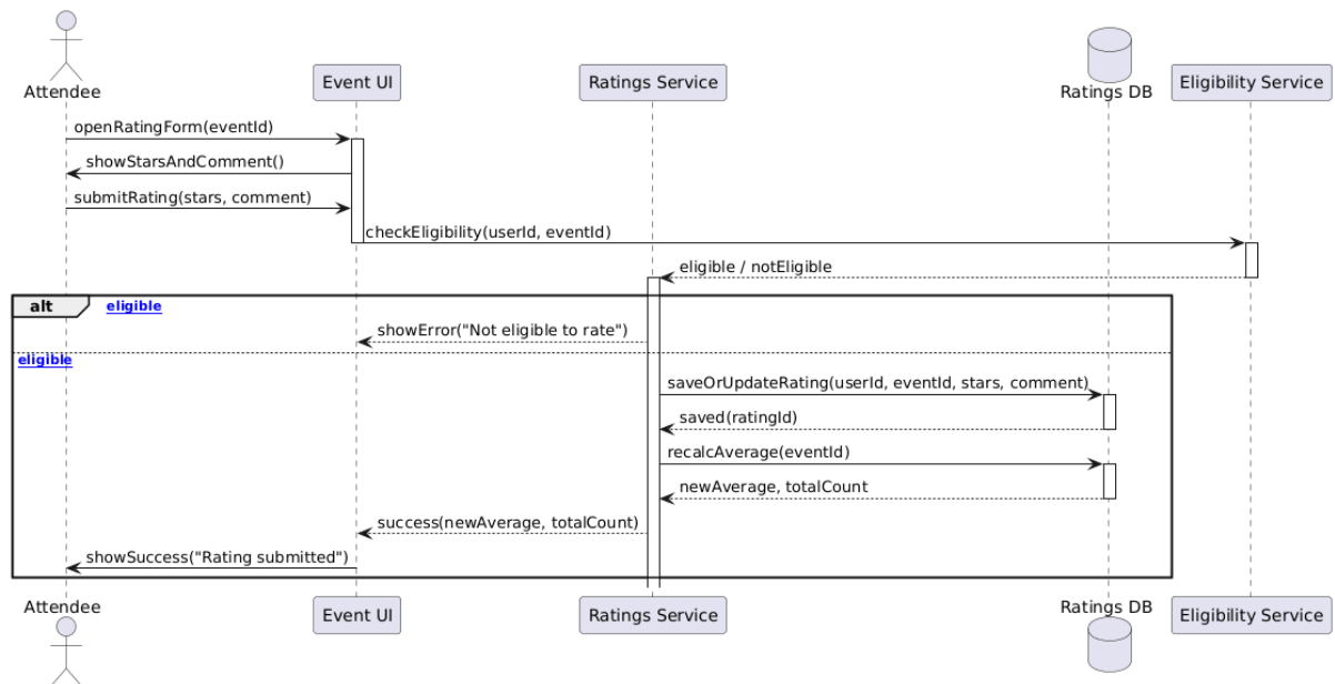
Figure 4.92 add event rating sequence diagram
