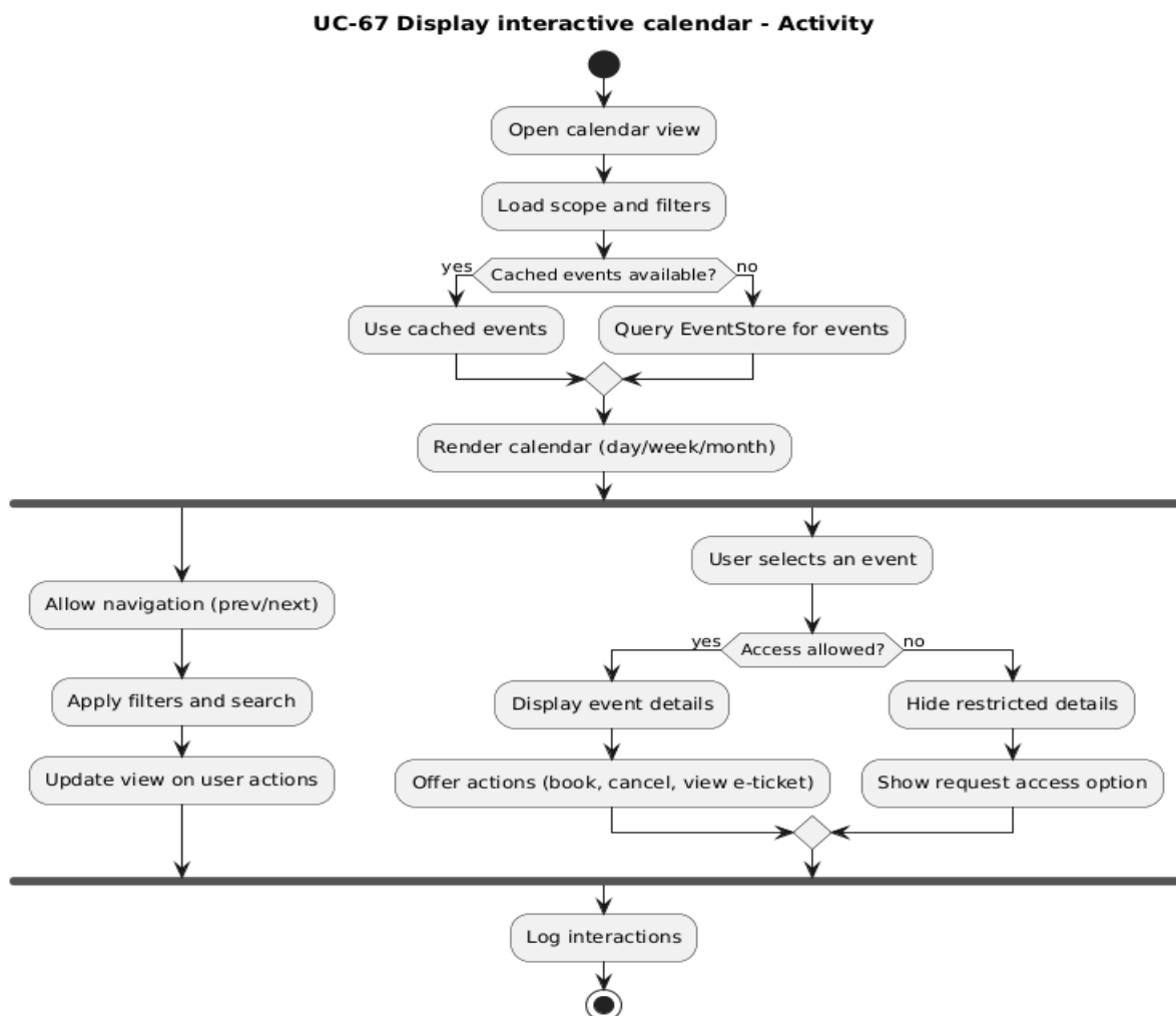
Figure 4.67 display interactive calendar activity diagram
