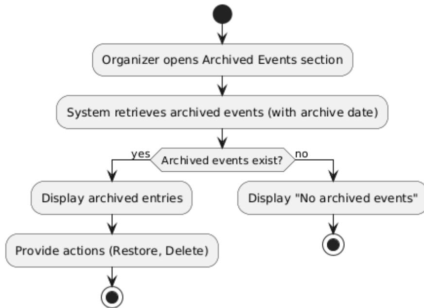
Figure 4.48 browse archived events activity diagram
