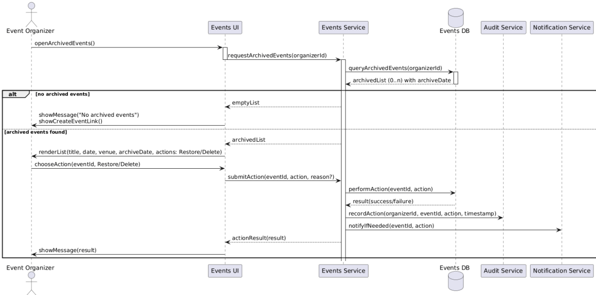
Figure 4.115 browse archived events sequence diagram
