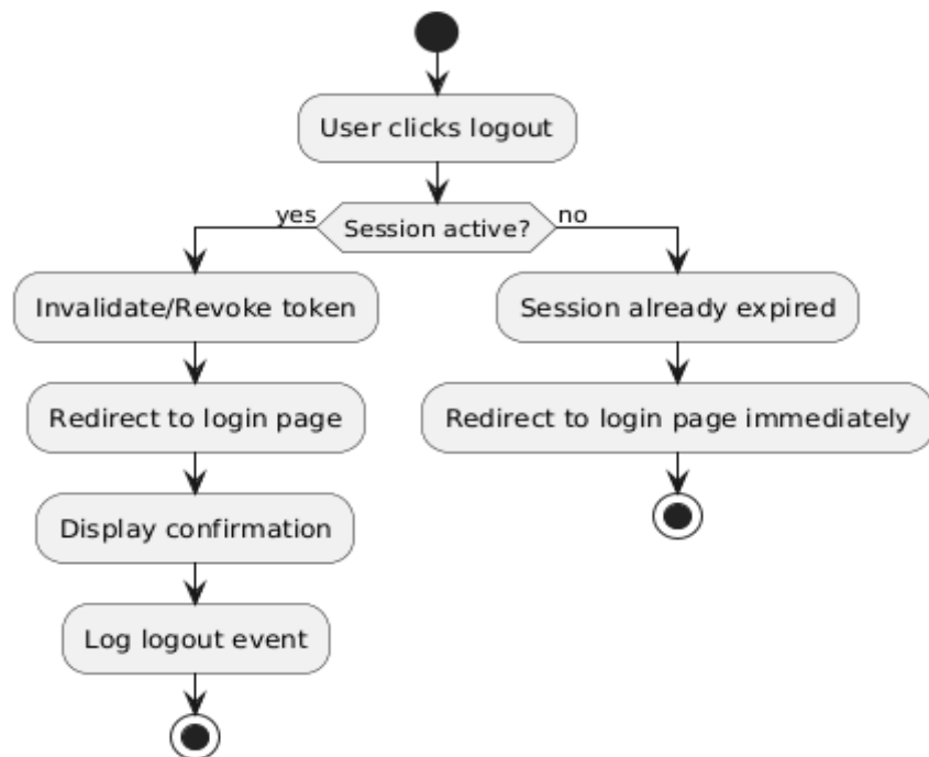
Figure 4.3 Register Logout activity diagram
