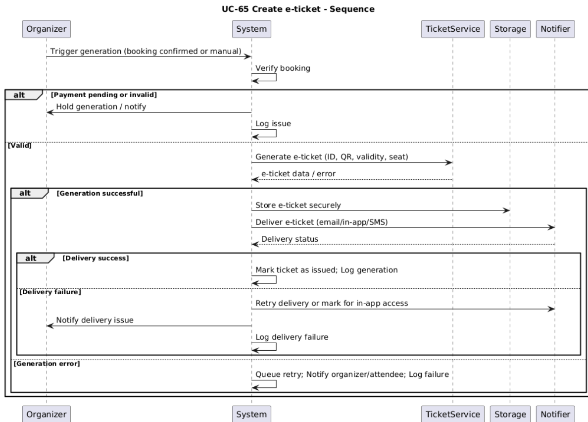
Figure 4.132 create e-ticket sequence diagram
