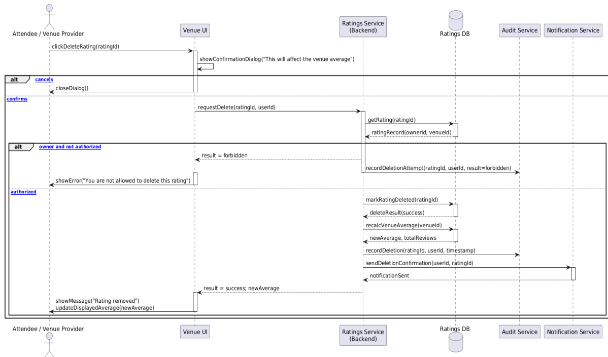
Figure 4.90 delete venue rating sequence diagram
