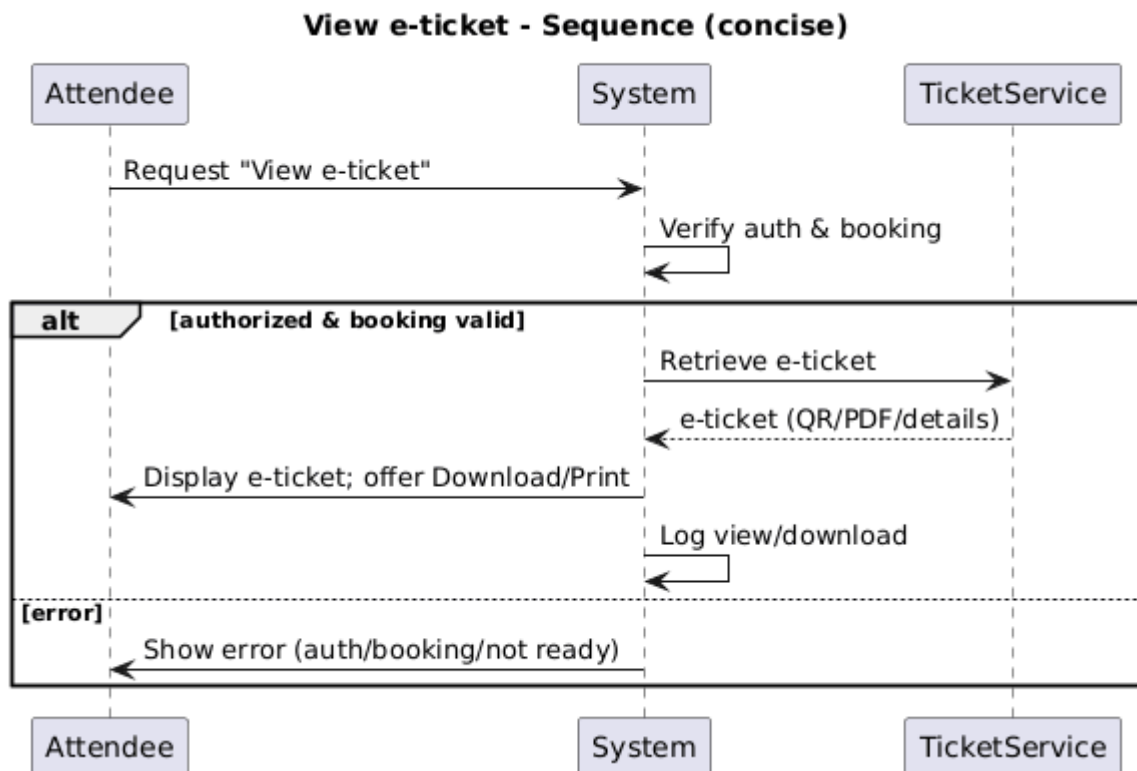
Figure 4.131 view e-ticket sequence diagram
