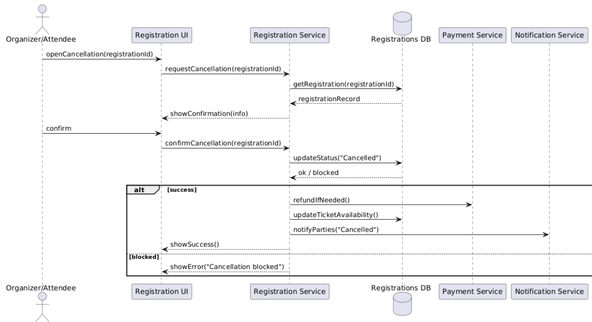
Figure 4.124 cancel registration sequence diagram
