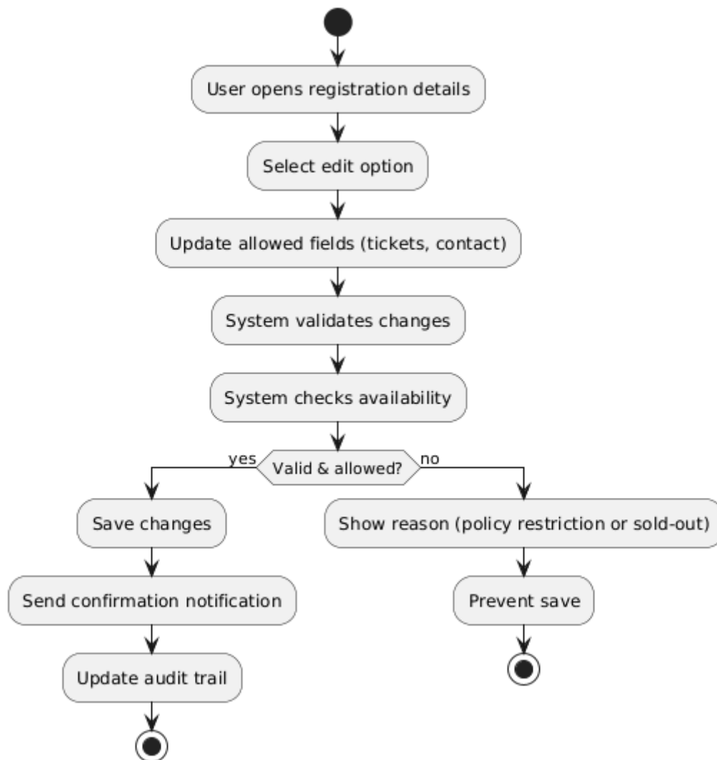
Figure 4.18 edit registration activity diagram
