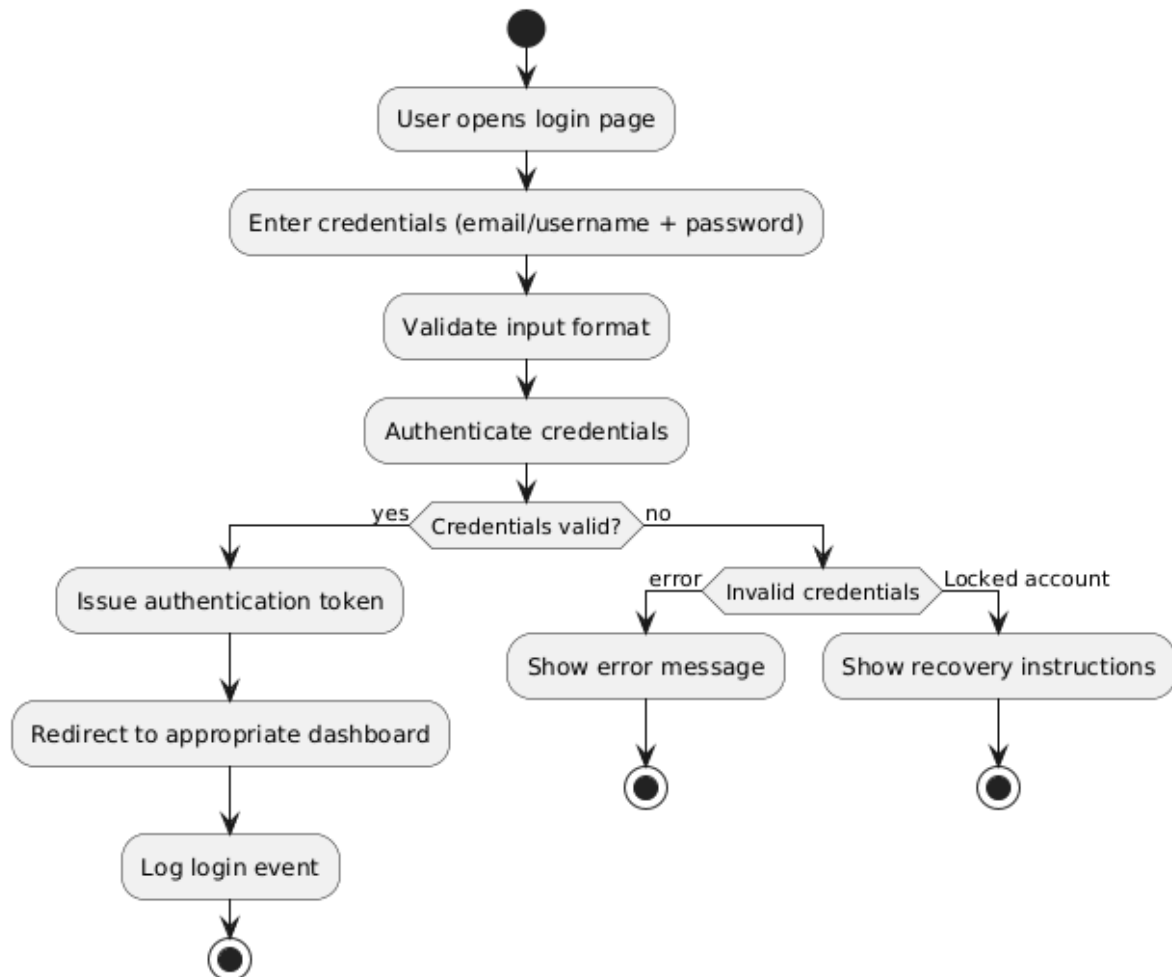
Figure 4.1 login activity diagram
