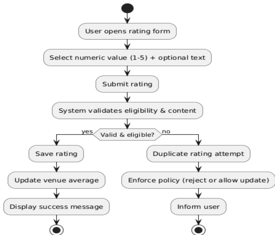
Figure 4.21 add venue rating activity diagram
