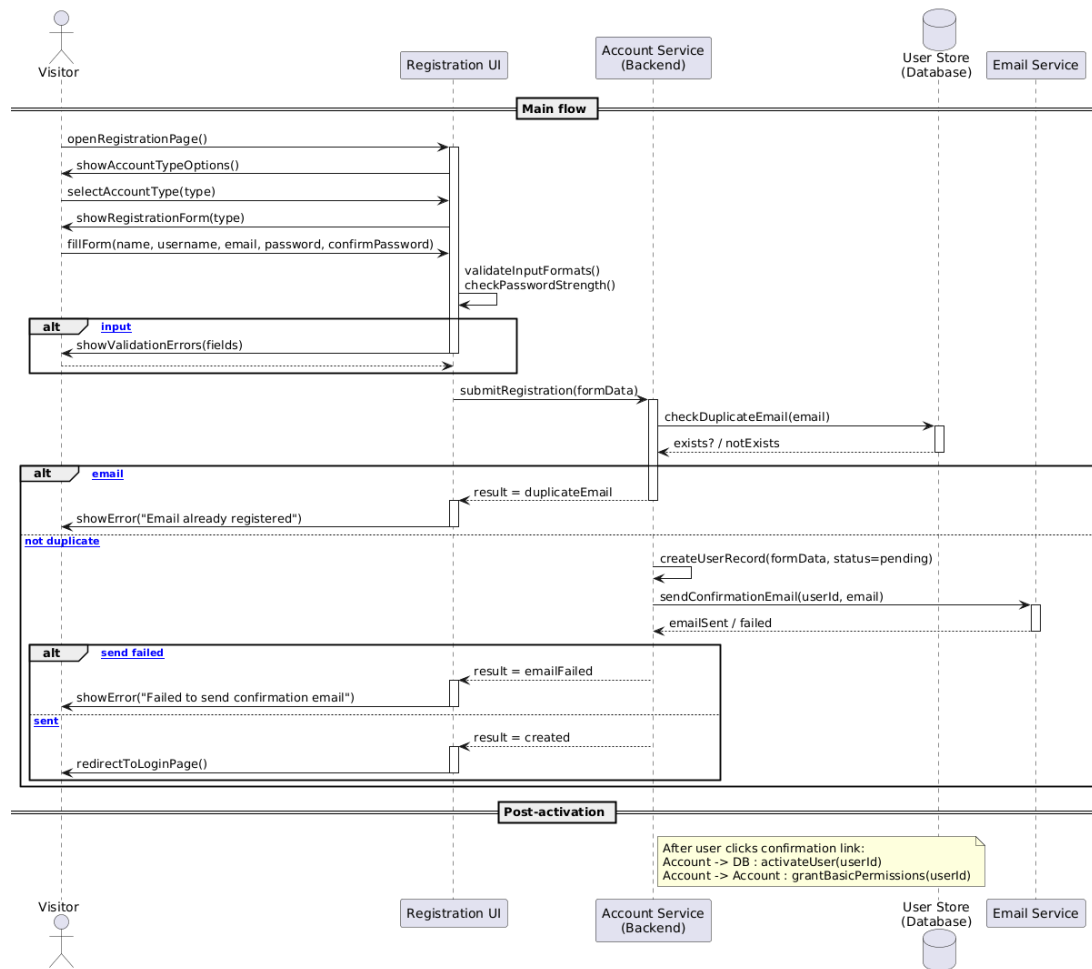
Figure 4.69 register (User Registration) sequence diagram
