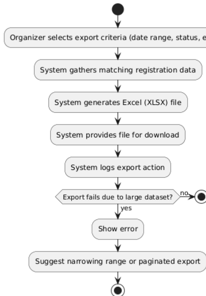
Figure 4.58 explore registration as excel file activity diagram
