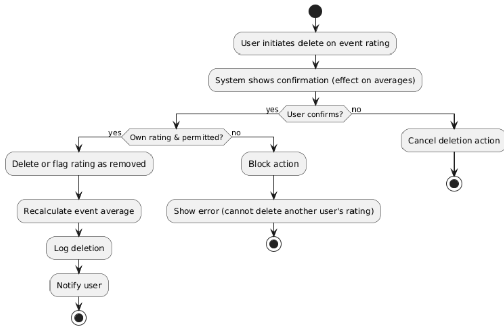
Figure 4.27 delete event rating activity diagram
