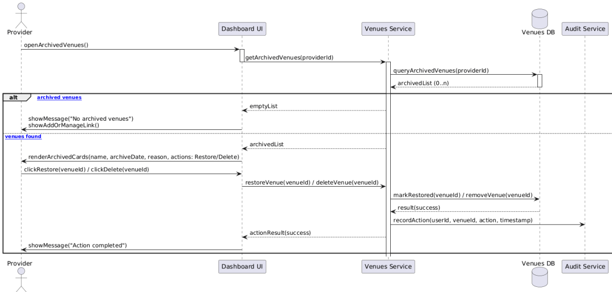
Figure 4.104 brows archived venues sequence diagram
