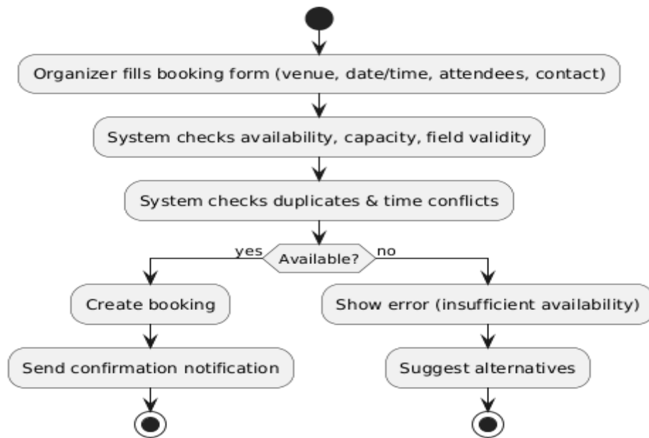
Figure 4.60 add booking (organizer) activity diagram
