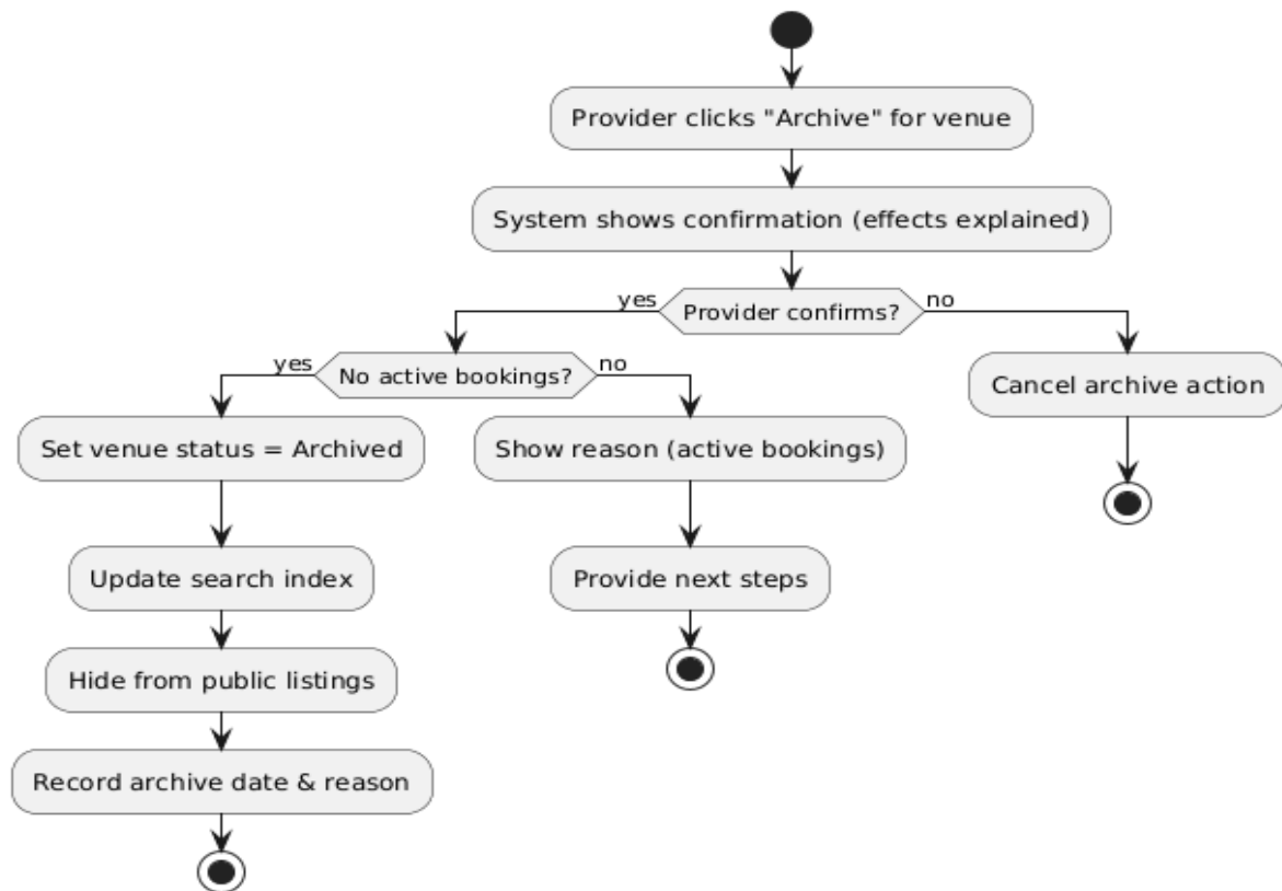
Figure 4.41 archive venue activity diagram
