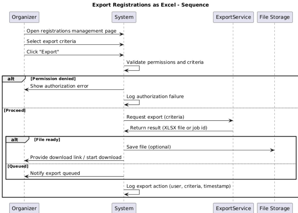
Figure 4.130 export registration as excel file sequence diagram
