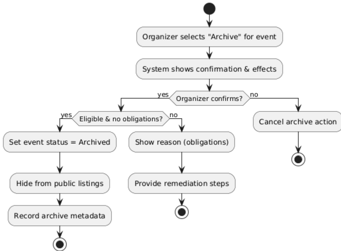
Figure 4.52 archive event activity diagram
