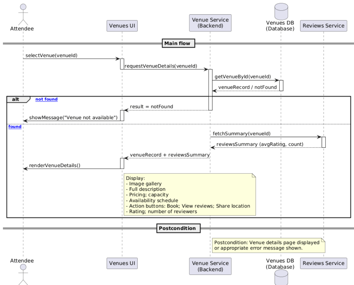
Figure 4.72 view venues details sequence diagram
