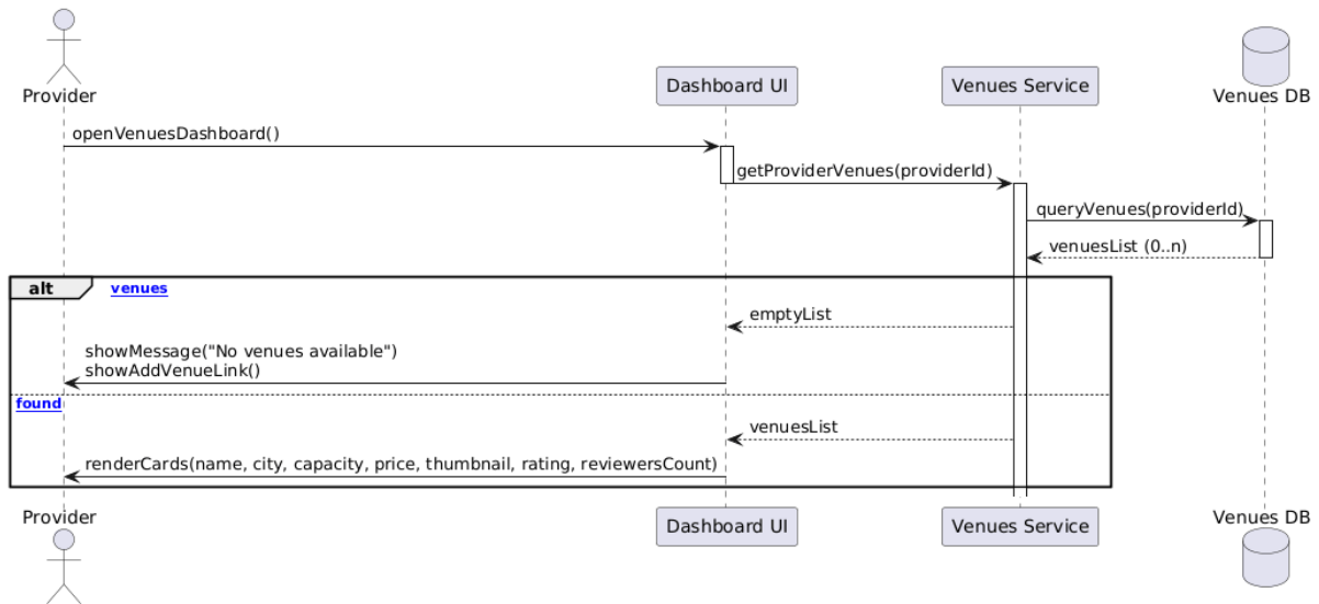
Figure 4.103 browse venues (provider) sequence diagram
