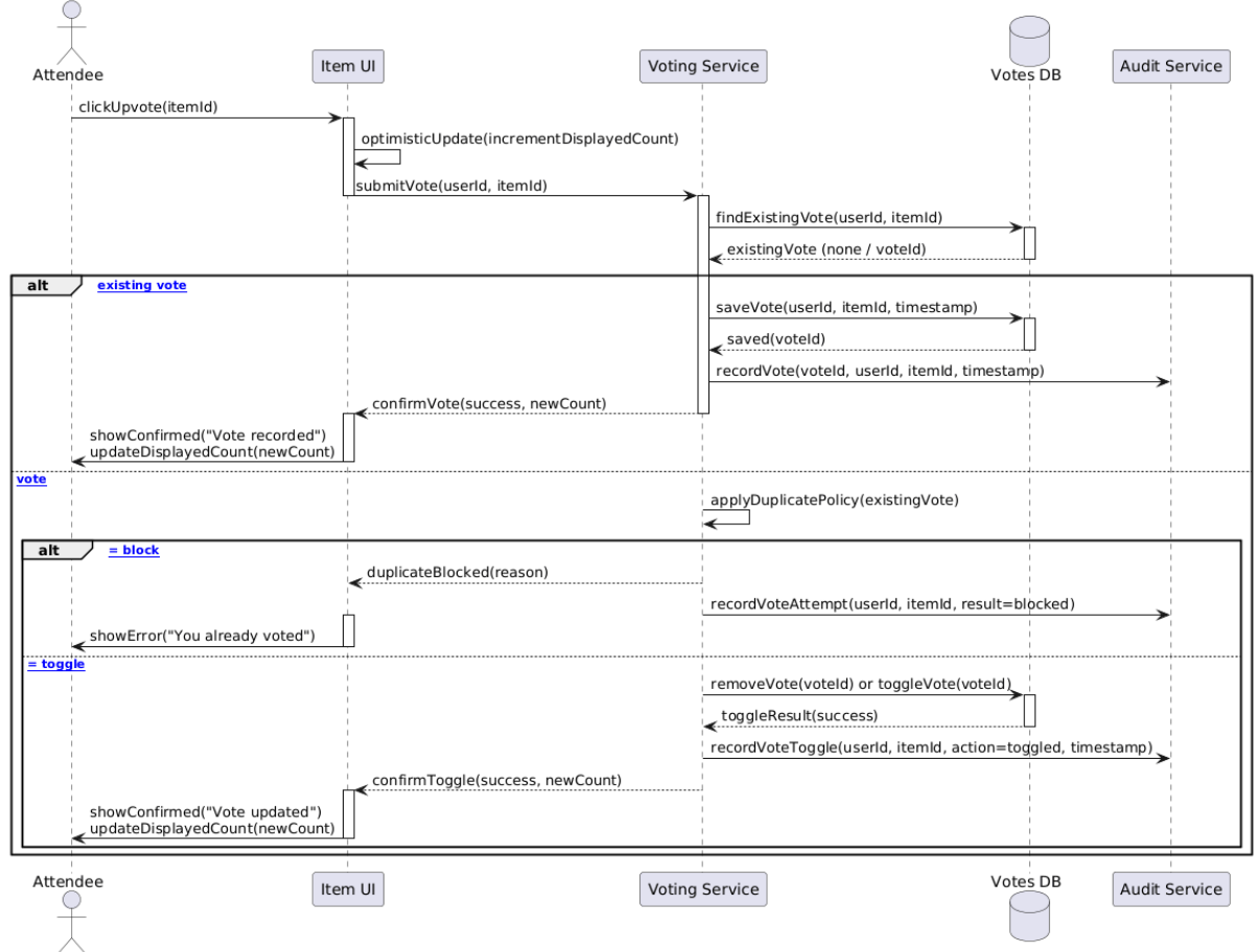
Figure 4.99 upvote sequence diagram
