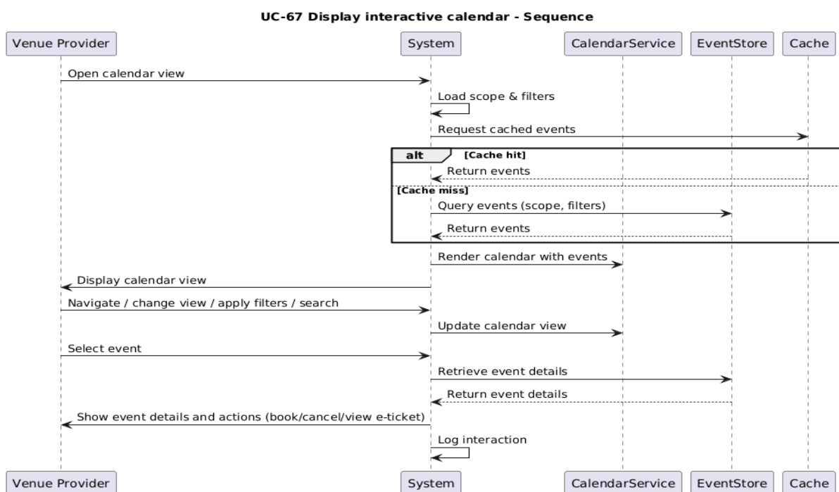
Figure 4.134 display interactive calendar sequence diagram
