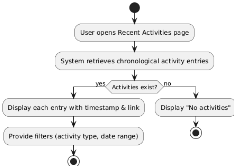
Figure 4.34 view recent activities activity diagram
