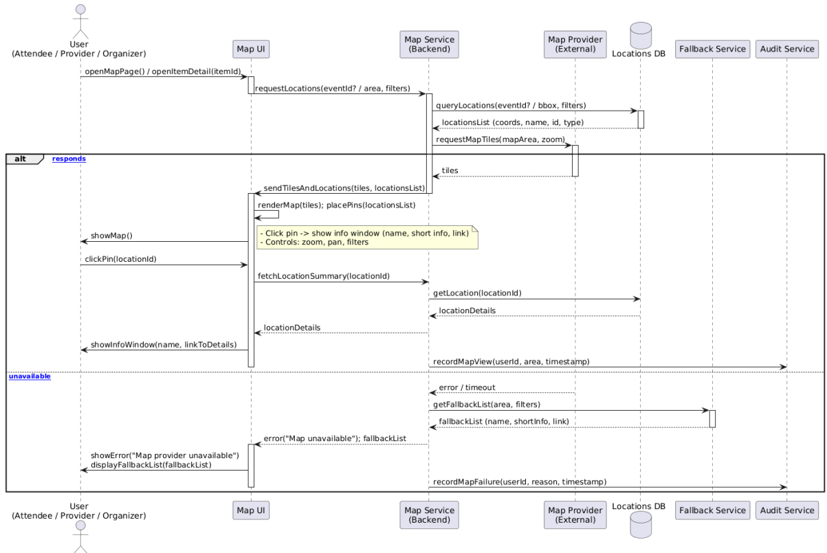
Figure 4.102 display map of event and venue locations sequence diagram
