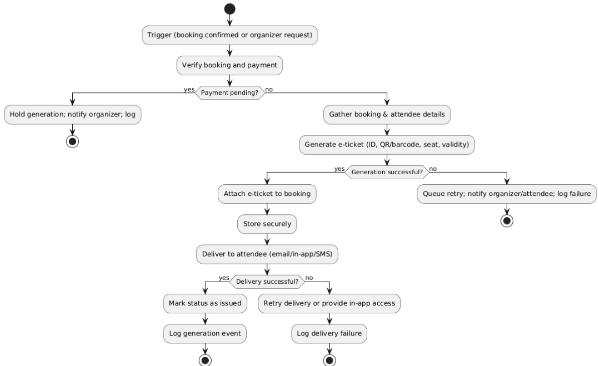
Figure 4.65 create e-ticket activity diagram
