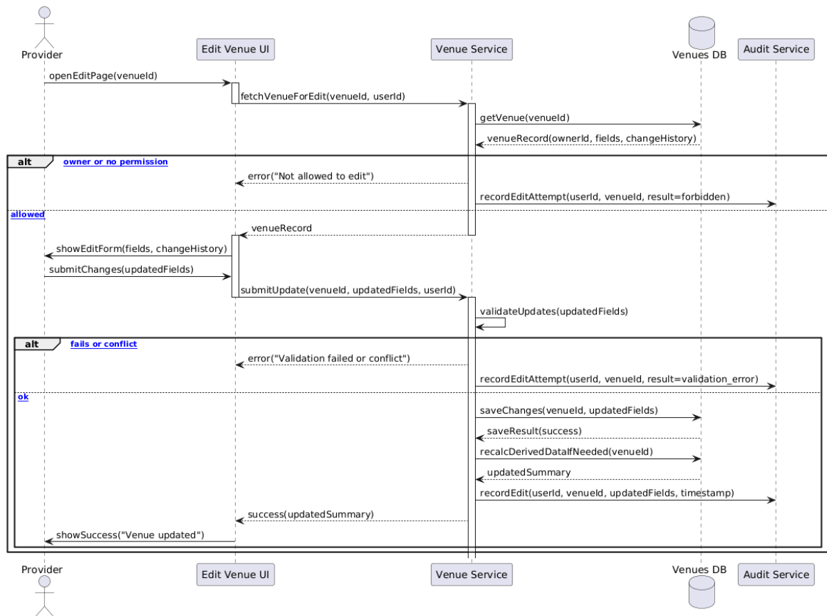
Figure 4.106 edit venue sequence diagram
