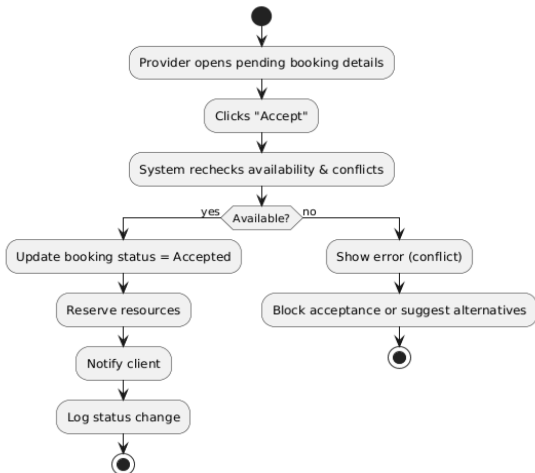
Figure 4.44 accept booking activity diagram
