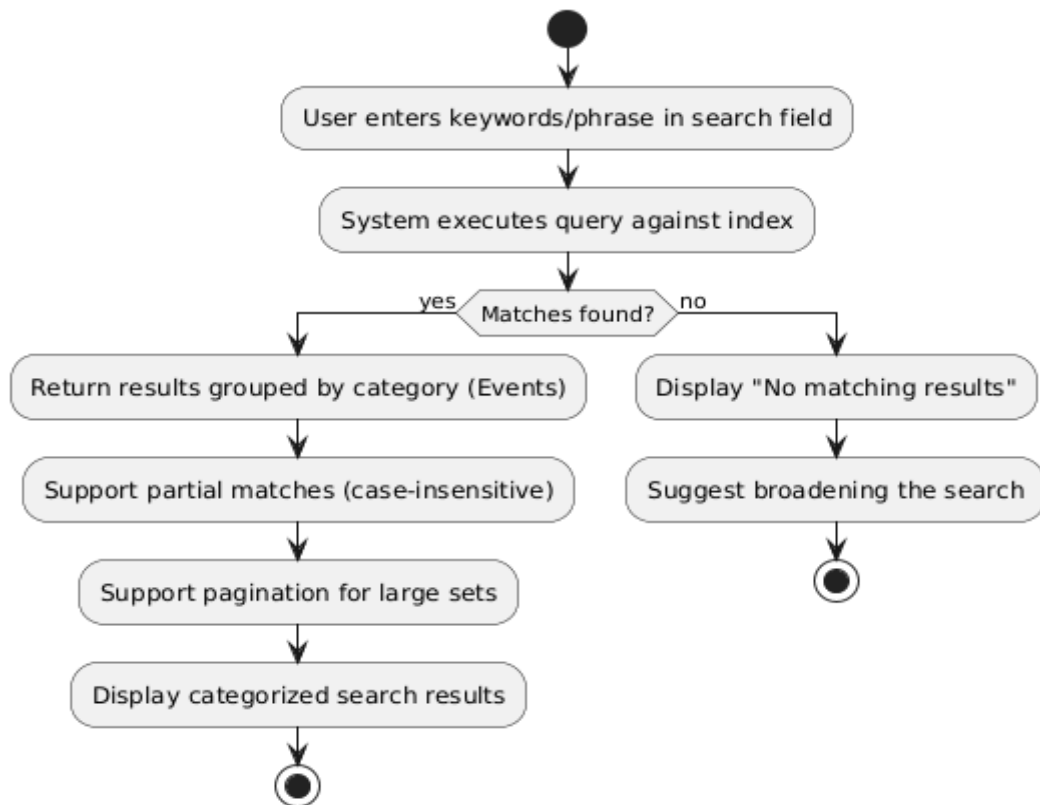
Figure 4.13 unified search for events activity diagram
