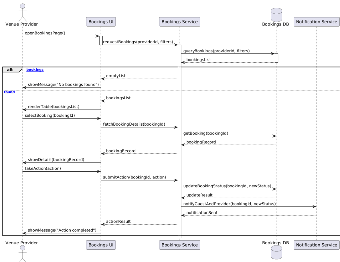
Figure 4.110 browse bookings sequence diagram
