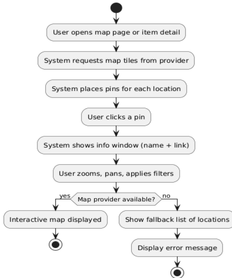
Figure 4.35 display map of event and venue locations activity diagram
