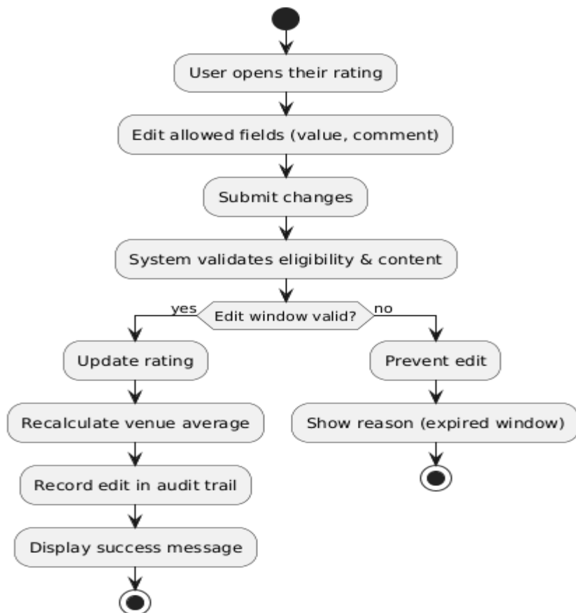
Figure 4.22 edit venue rating activity diagram
