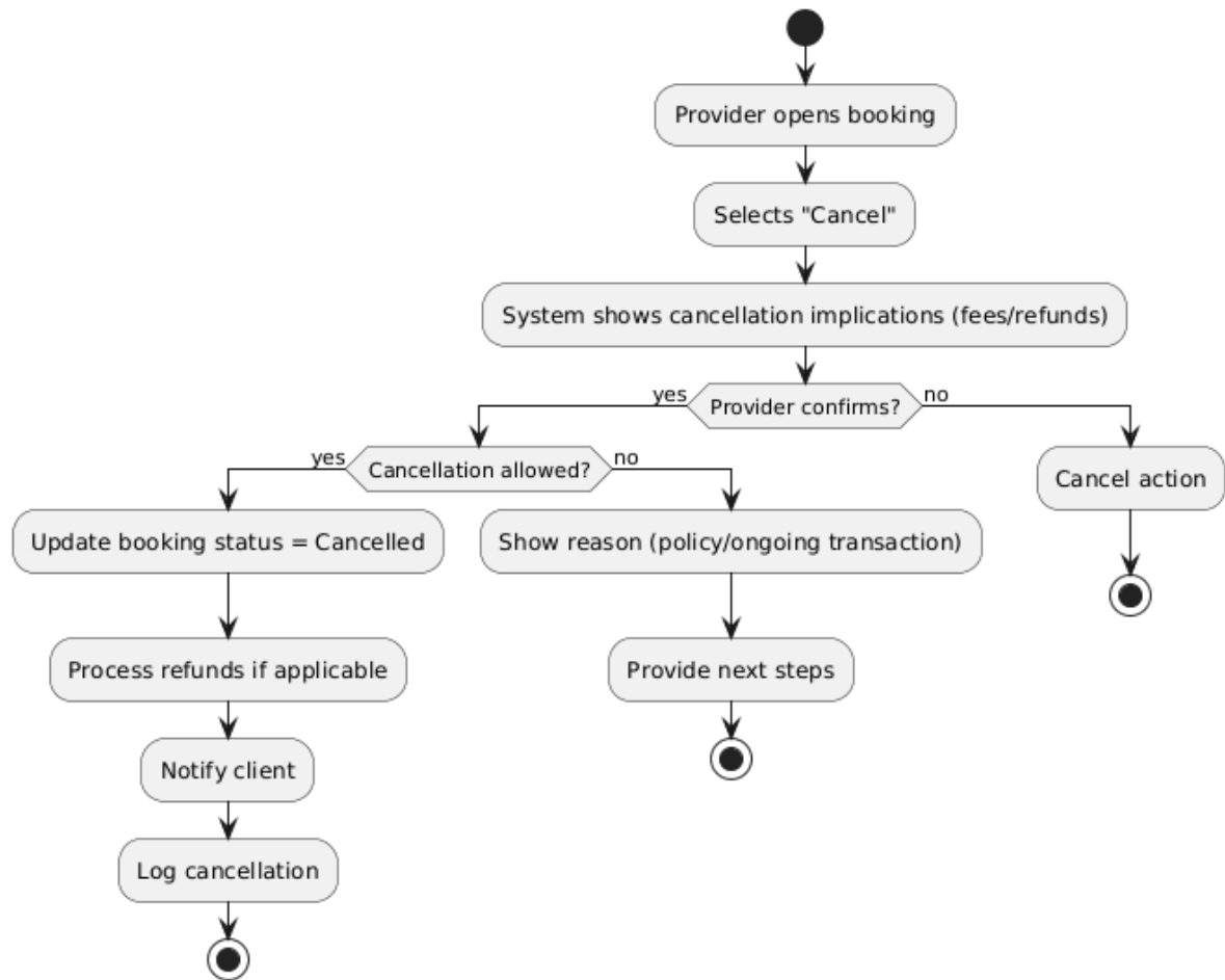
Figure 4.46 cancel booking activity diagram
