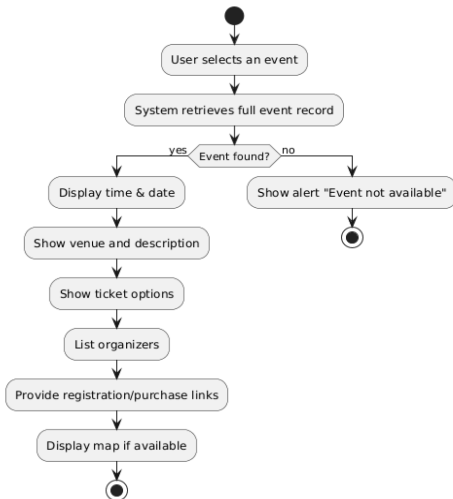
Figure 4.11 view events details activity diagram
