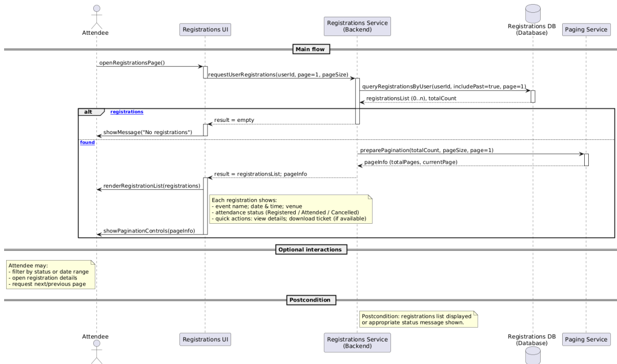
Figure 4.83 view registration sequence diagram
