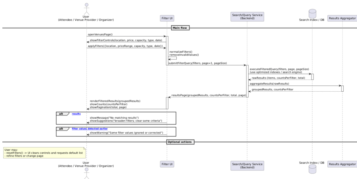
Figure 4.81 filter venues by specific criteria sequence diagram
