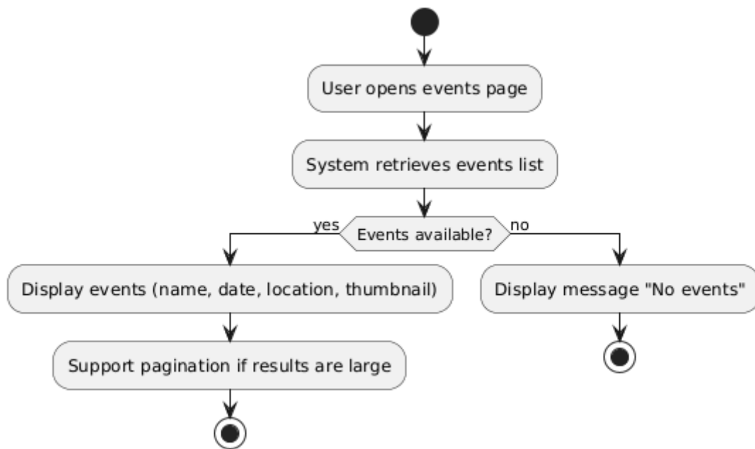
Figure 4.10 view events activity diagram
