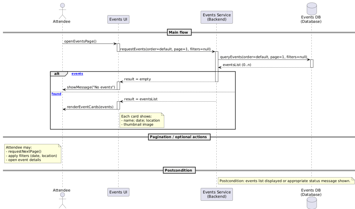
Figure 4.77 view events sequence diagram
