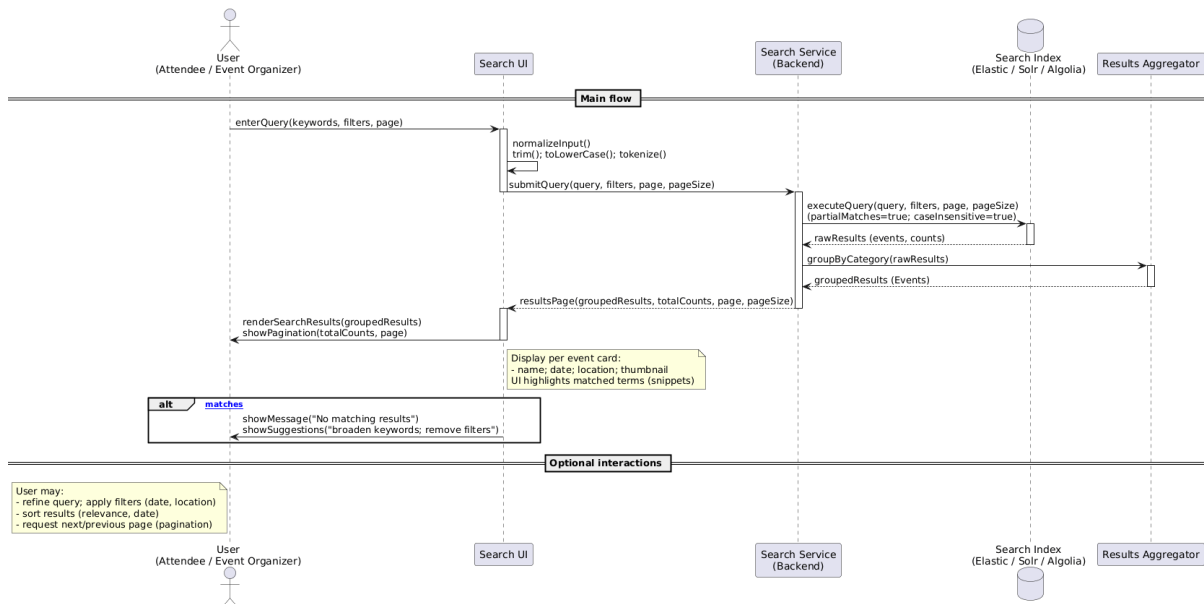
Figure 4.80 unified search for events sequence diagram
