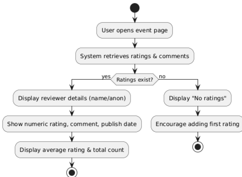
Figure 4.24 view event ratings activity diagram
