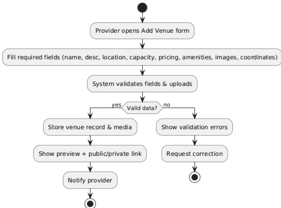
Figure 4.38 add venue activity diagram.
