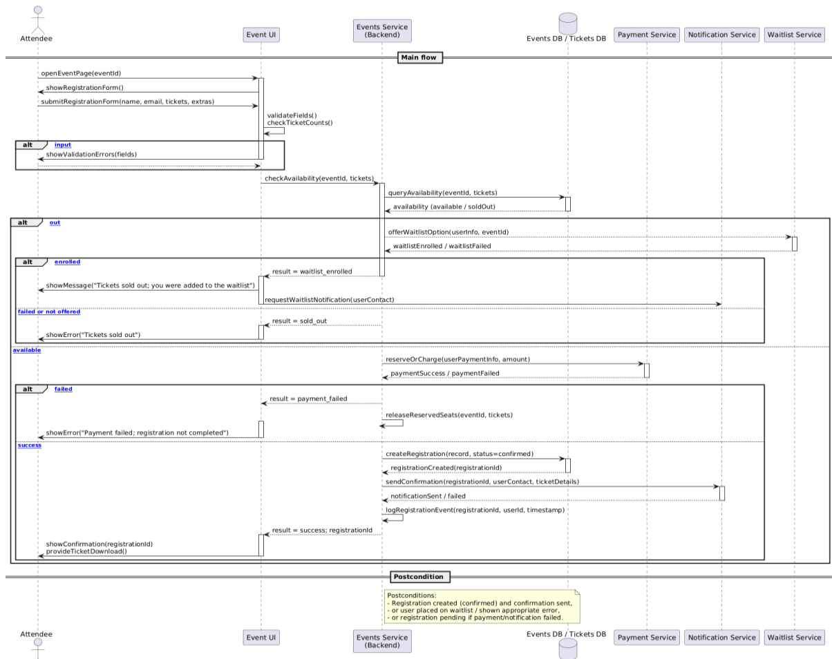
Figure 4.84 add registration sequence diagram
