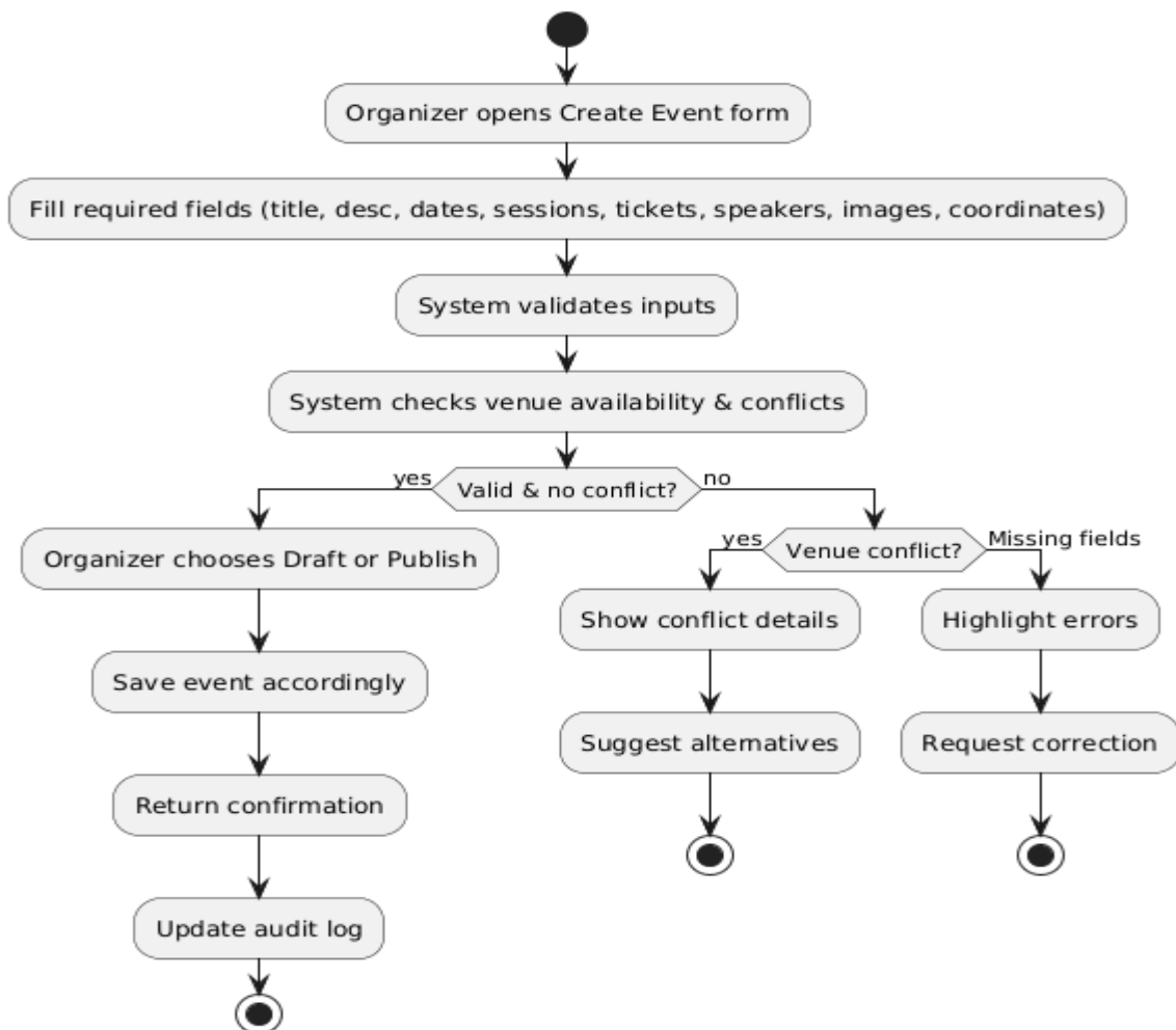
Figure 4.49 create event activity diagram
