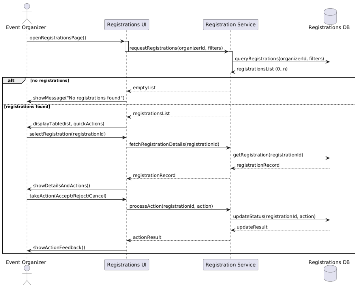
Figure 4.121 browse registrations sequence diagram
