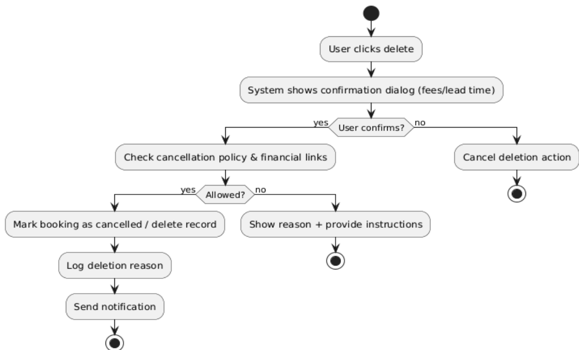
Figure 4.9 delete booking activity diagram
