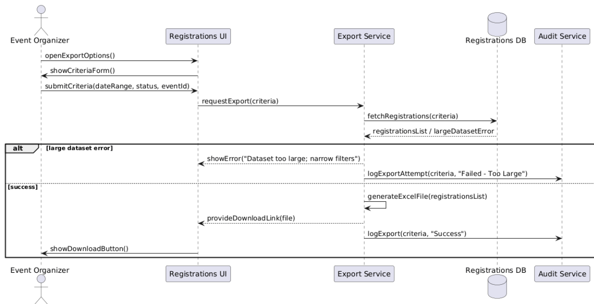
Figure 4.125 explore registration as excel file sequence diagram
