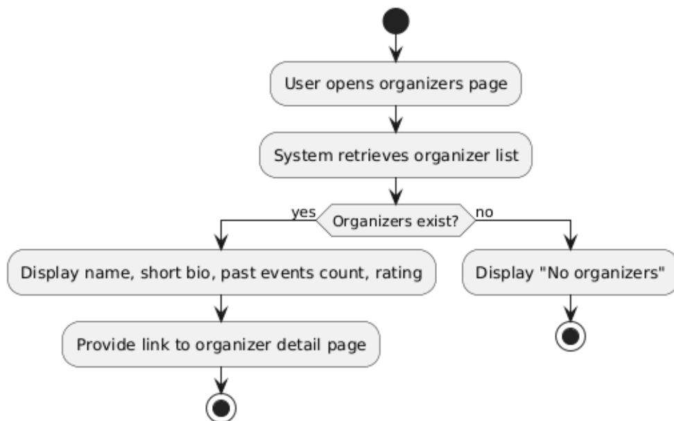
Figure 4.28 view organizers activity diagram
