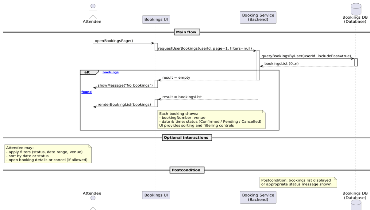
Figure 4.73 view bookings sequence diagram
