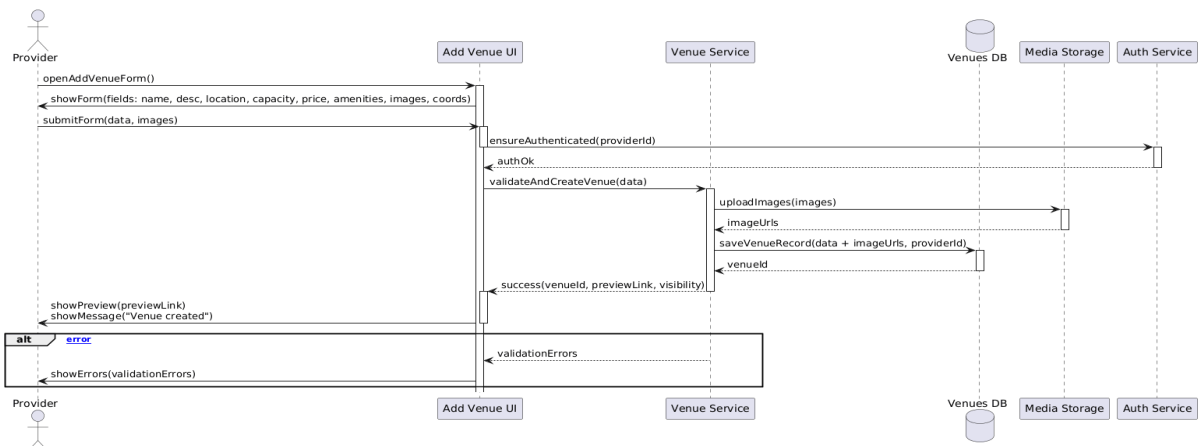
Figure 4.105 add venue sequence diagram
