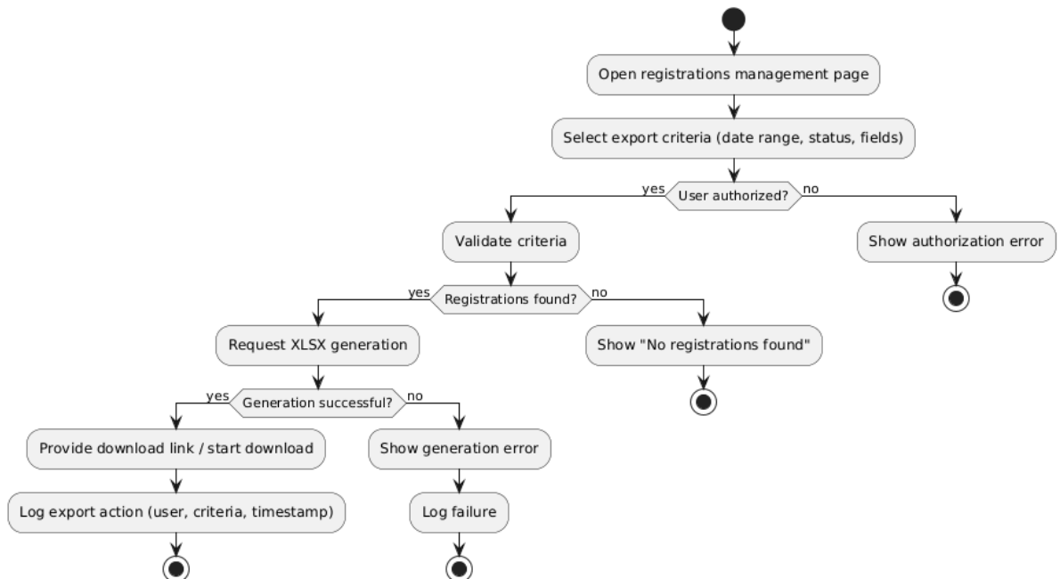
Figure 4.63 export registration as excel file activity diagram
