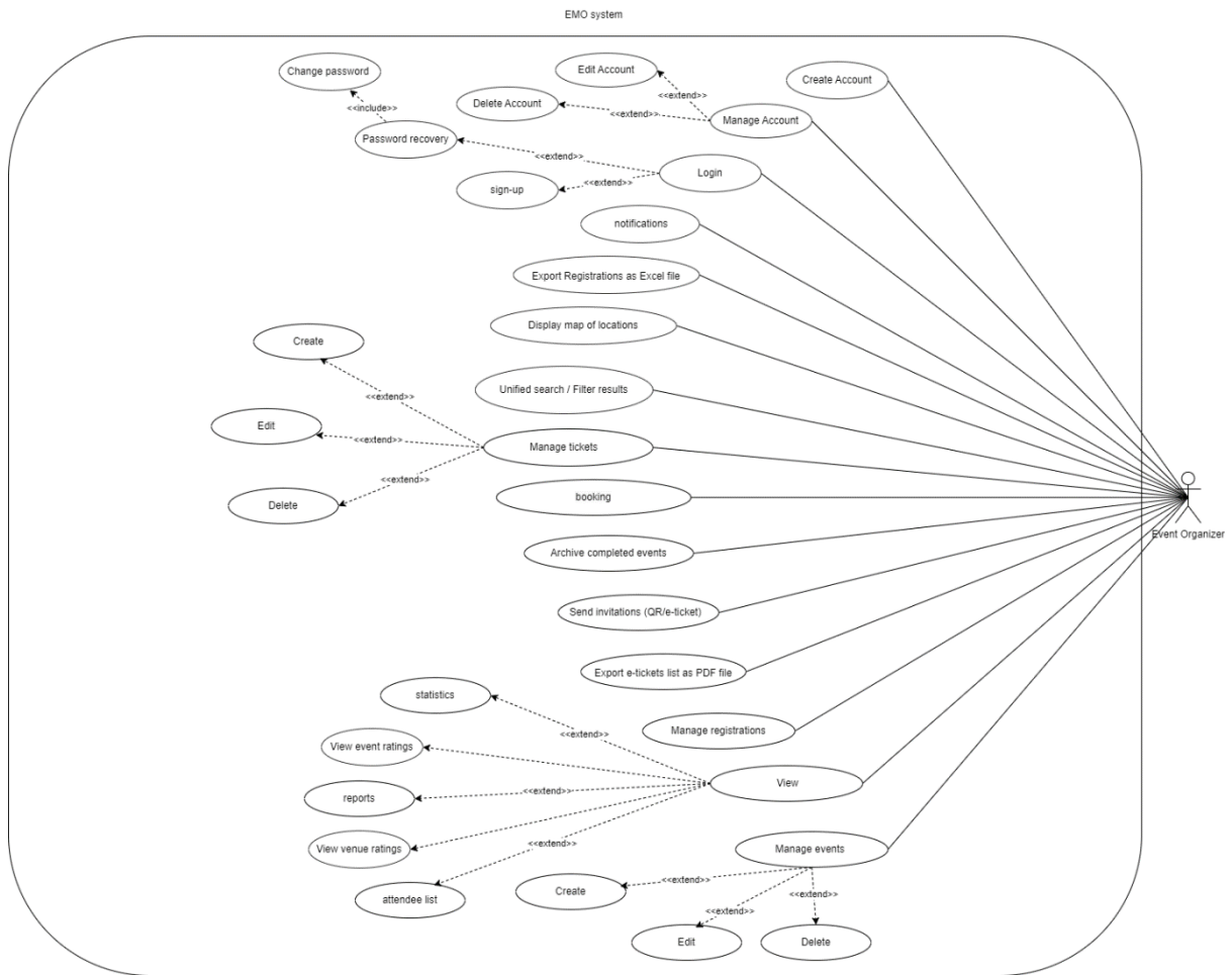
Figure 4.4 event organizer use case diagram
