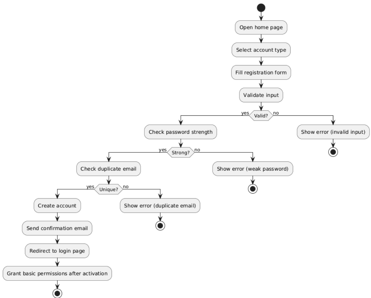
Figure 4.2 register (User Registration) activity diagram
