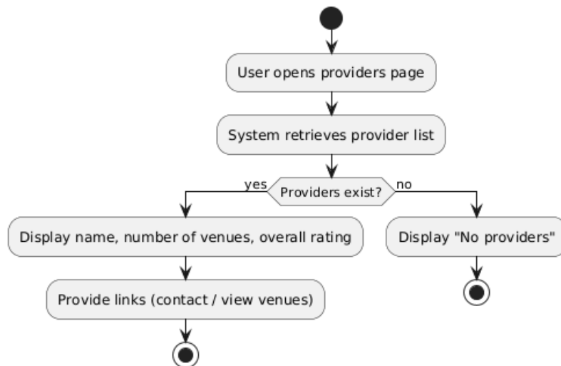
Figure 4.29 view providers activity diagram
