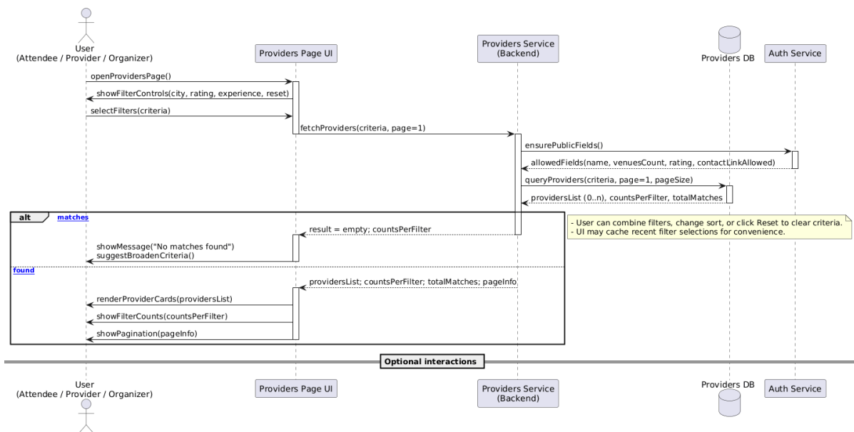
Figure 4.97 filter providers by specific criteria sequence diagram
