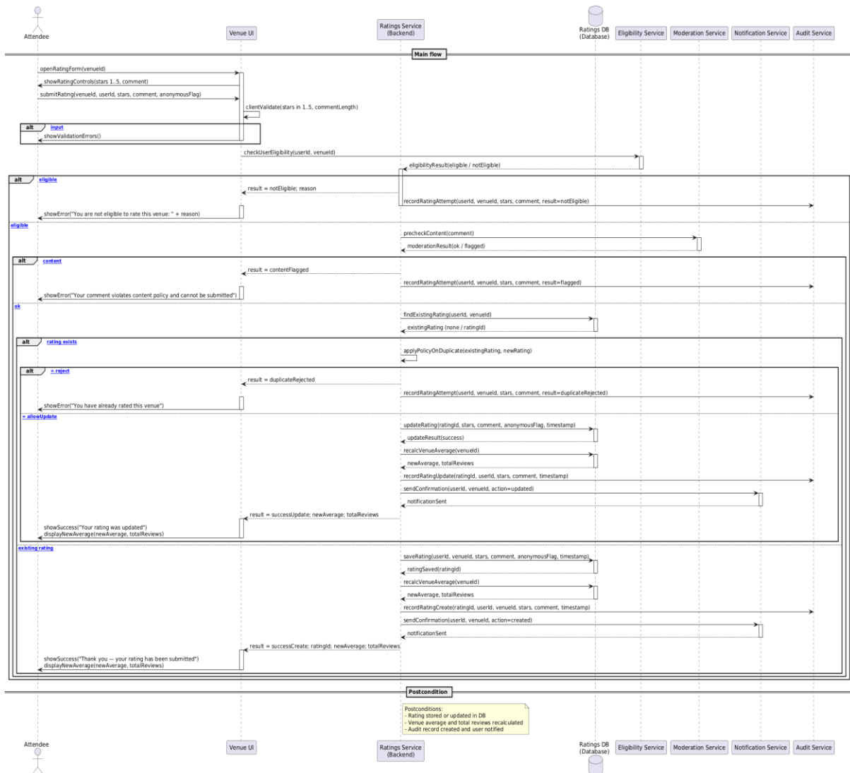
Figure 4.88 add venue rating sequence diagram
