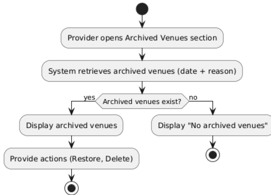
Figure 4.37 brows archived venues activity diagram
