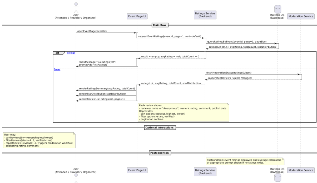
Figure 4.91 view event ratings sequence diagram
