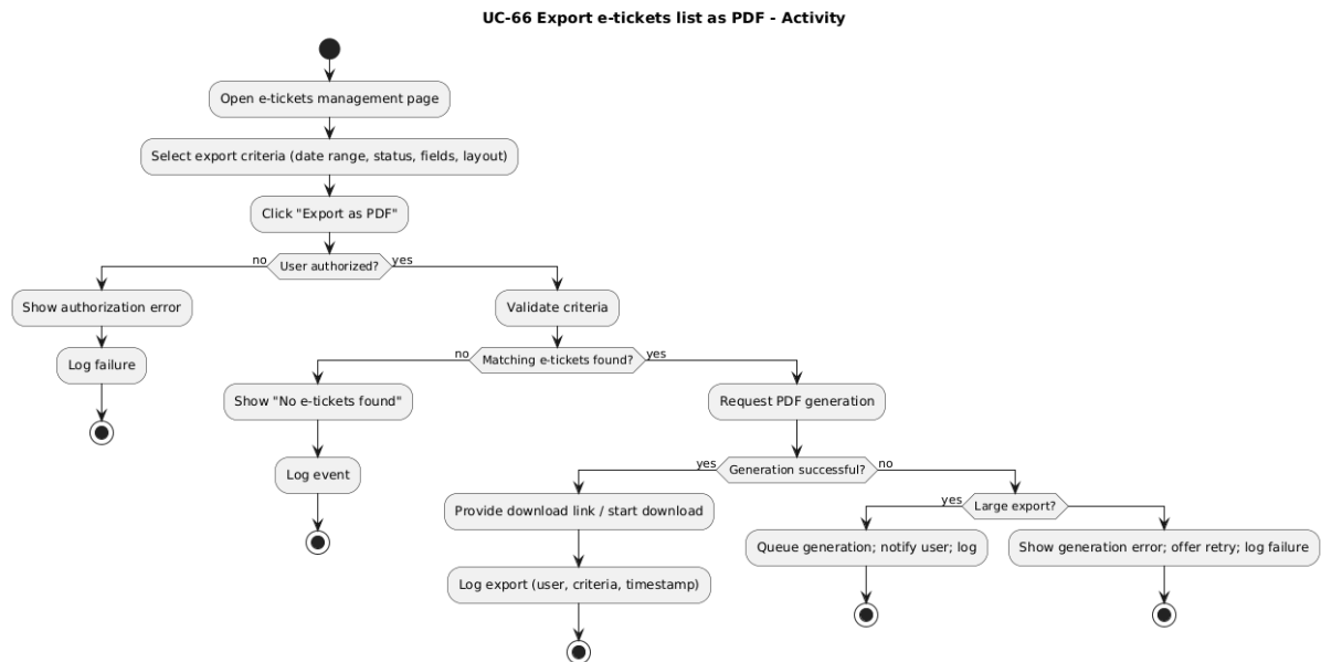
Figure 4.66 export e-tickets list as pdf activity diagram
