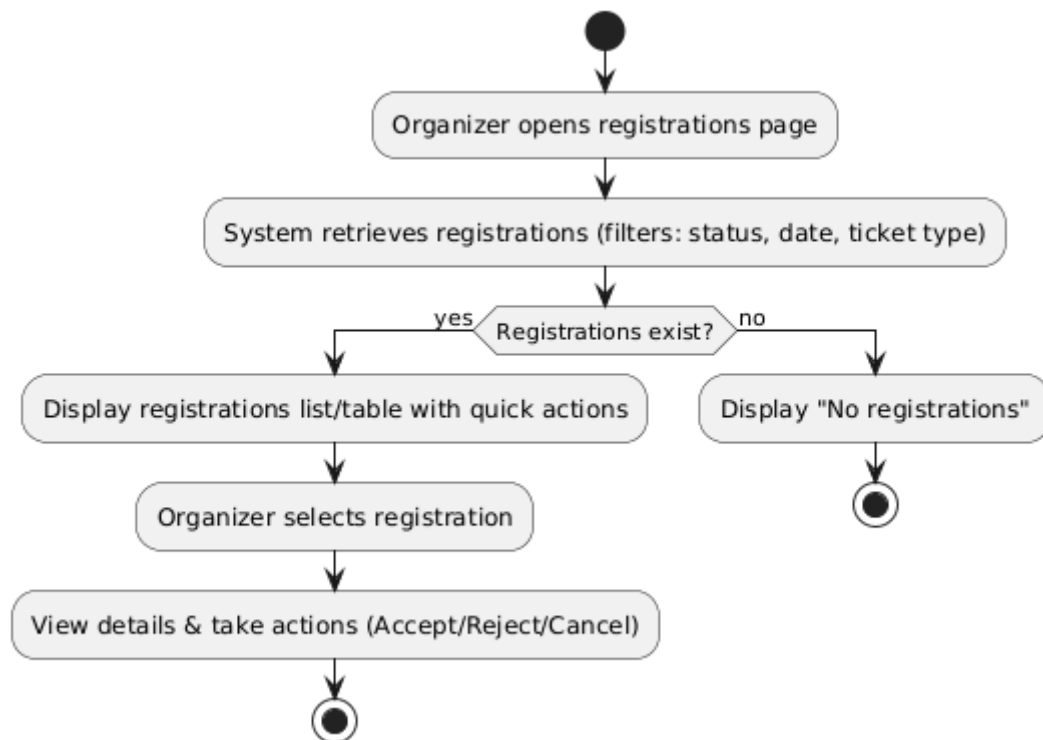
Figure 4.54 browse registrations activity diagram
