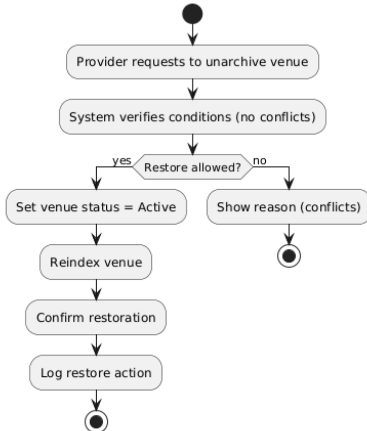
Figure 4.42 unarchive venue activity diagram
