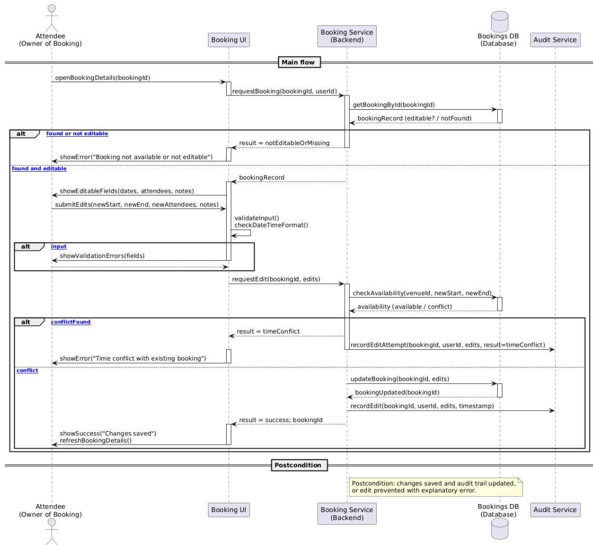
Figure 4.75 edit booking sequence diagram
