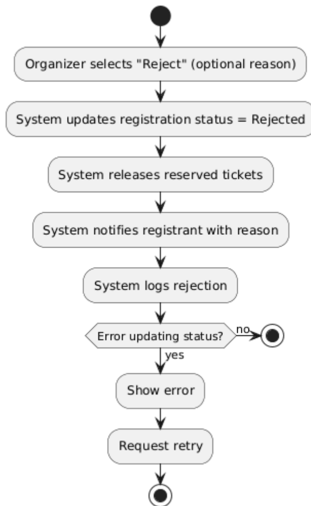
Figure 4.56 reject registration activity diagram
