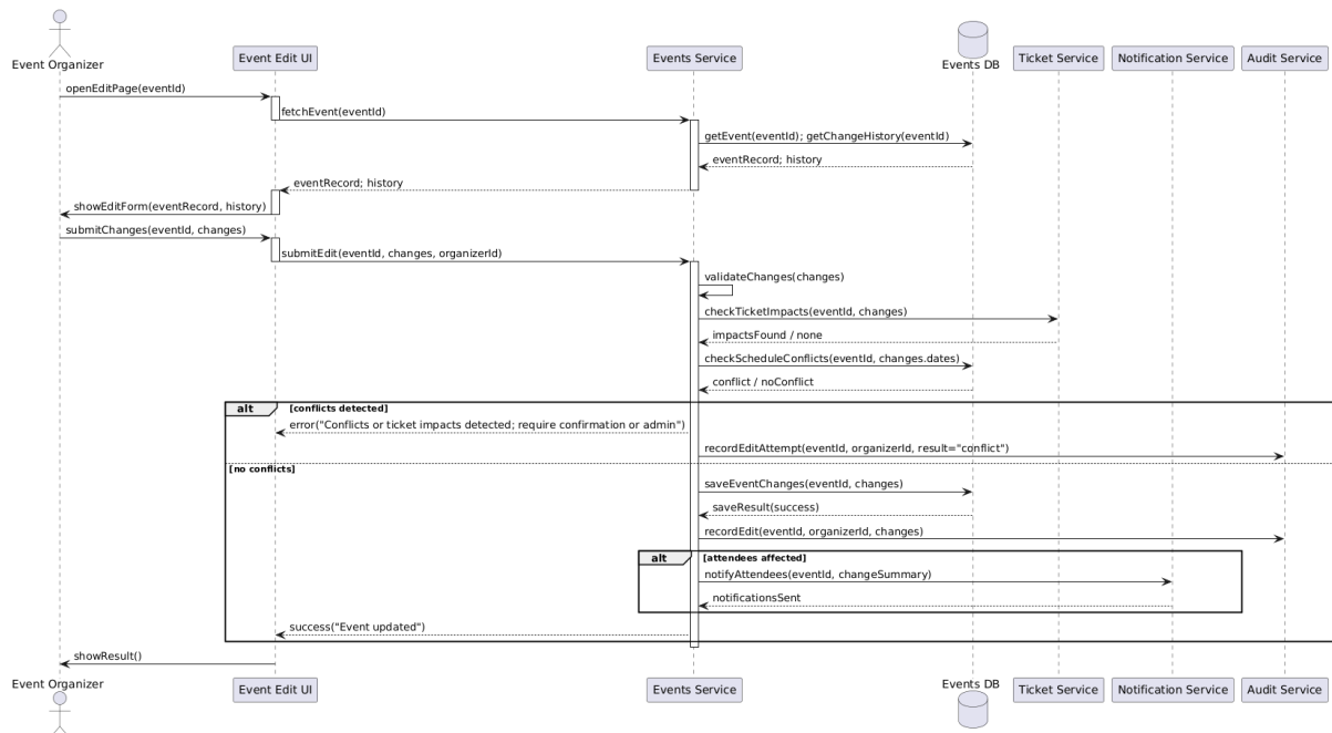
Figure 4.117 edit event sequence diagram
