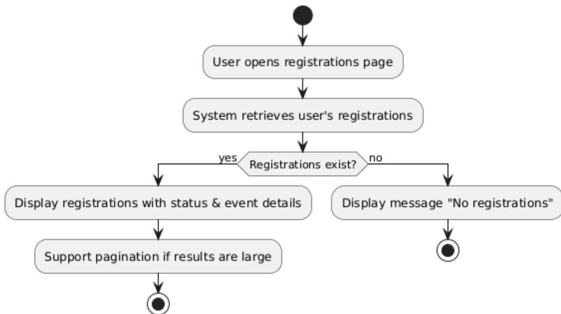
Figure 4.16 view registration activity diagram
