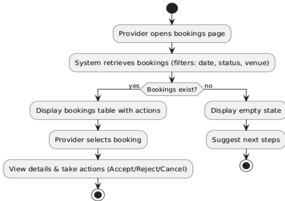
Figure 4.43 browse bookings activity diagram
