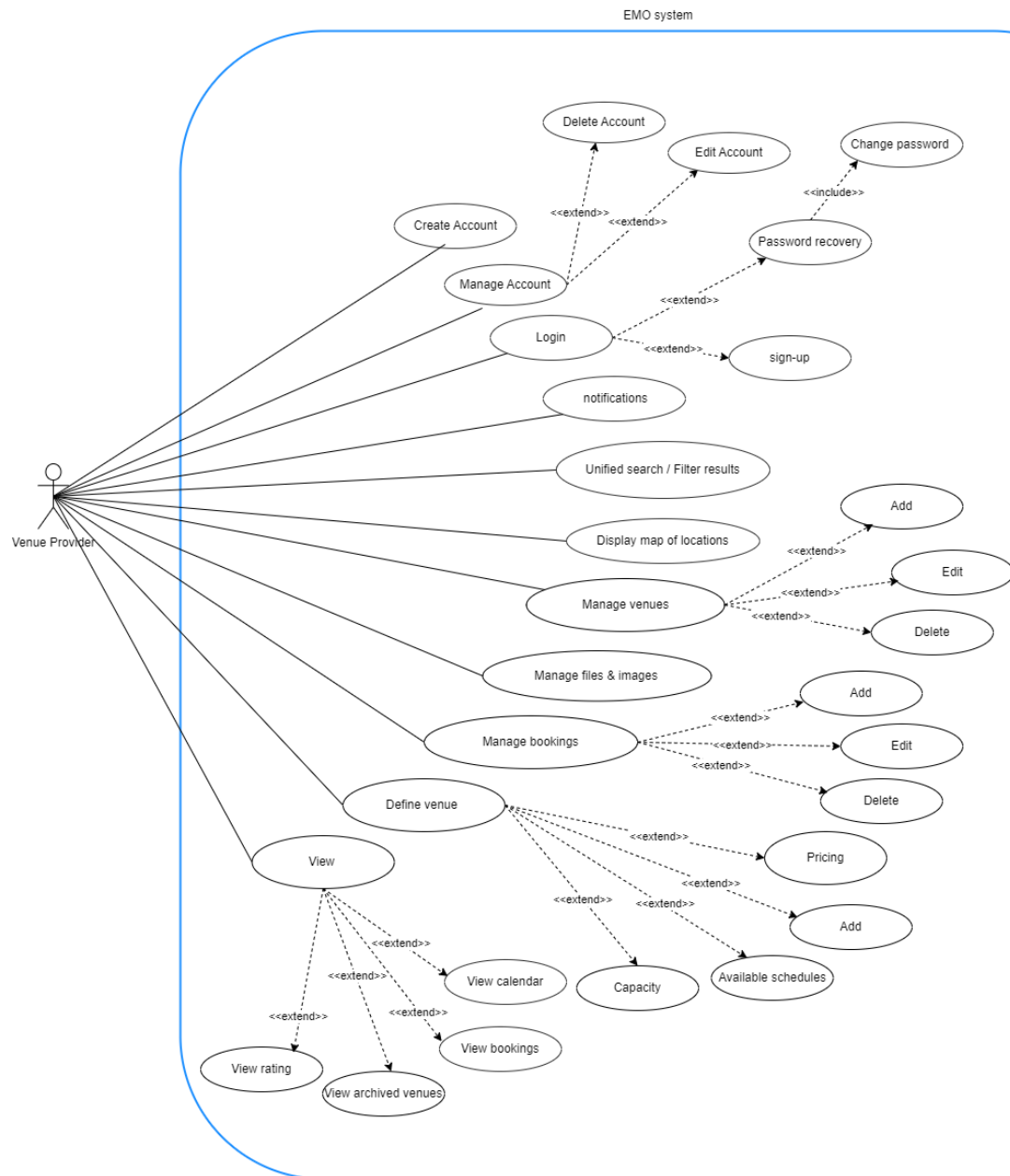
Figure 4.4 venue provider use case diagram
