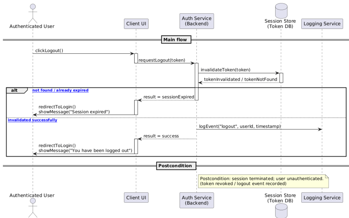
Figure 4.70 Register Logout sequence diagram
