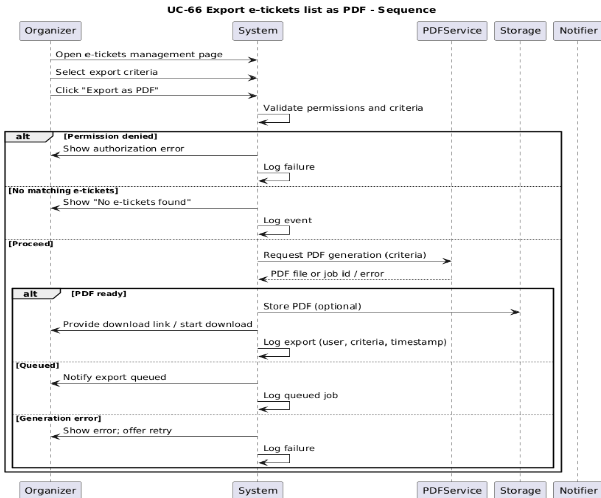
Figure 4.133 export e-ticket list as pdf sequence diagram
