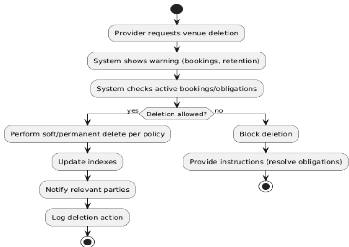
Figure 4.40 delete venue activity diagram
