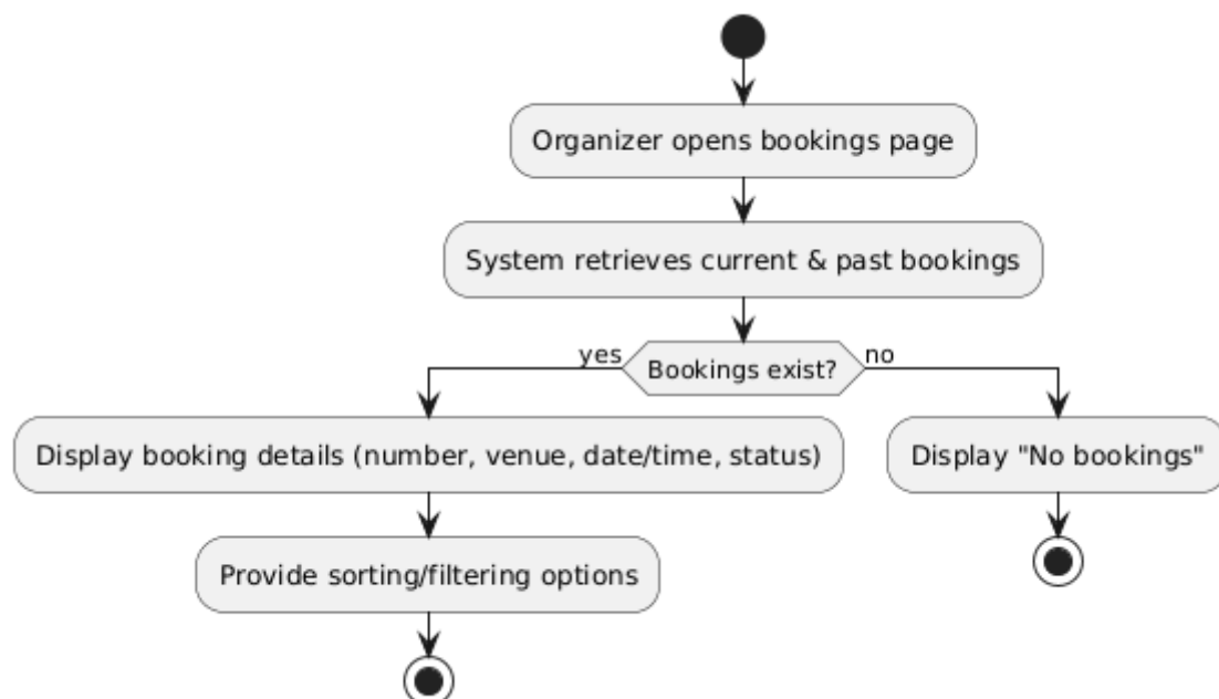
Figure 4.59 view booking (organizer) activity diagram
