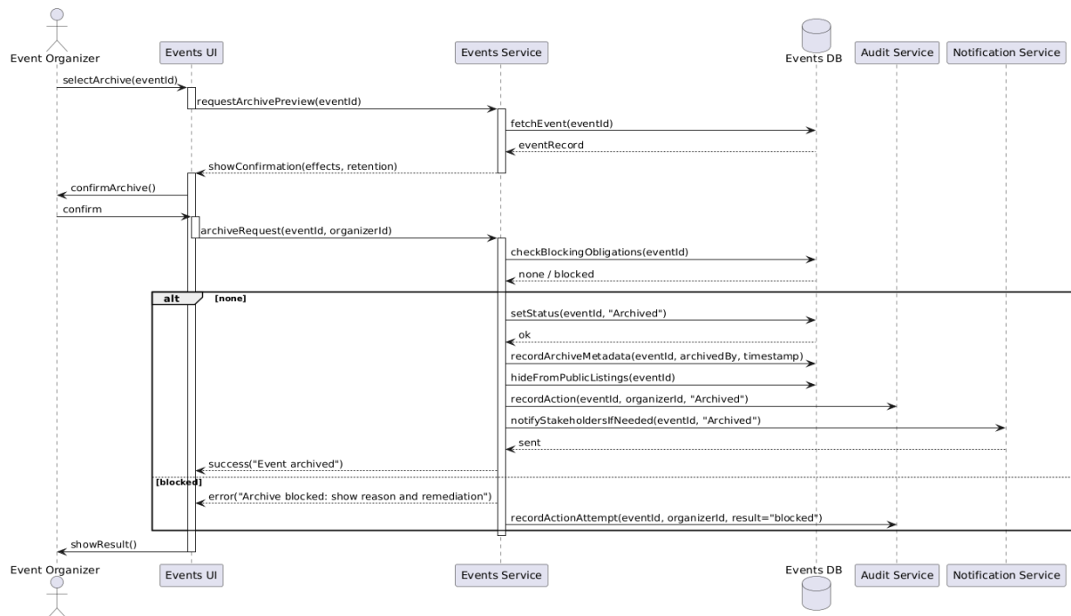
Figure 4.119 archive event sequence diagram
