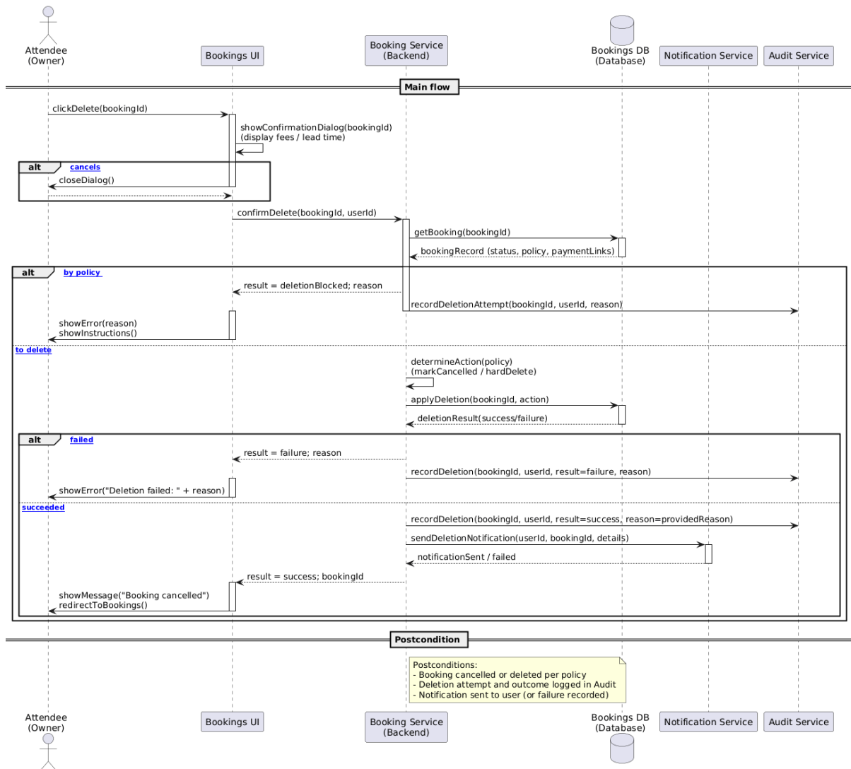
Figure 4.76 delete booking sequence diagram
