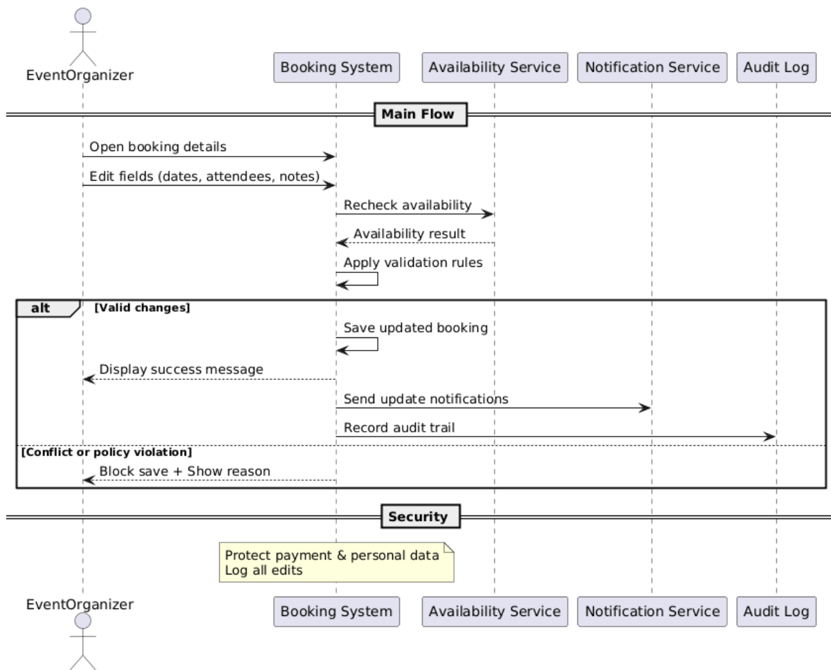
Figure 4.128 edit booking (organizer) sequence diagram
