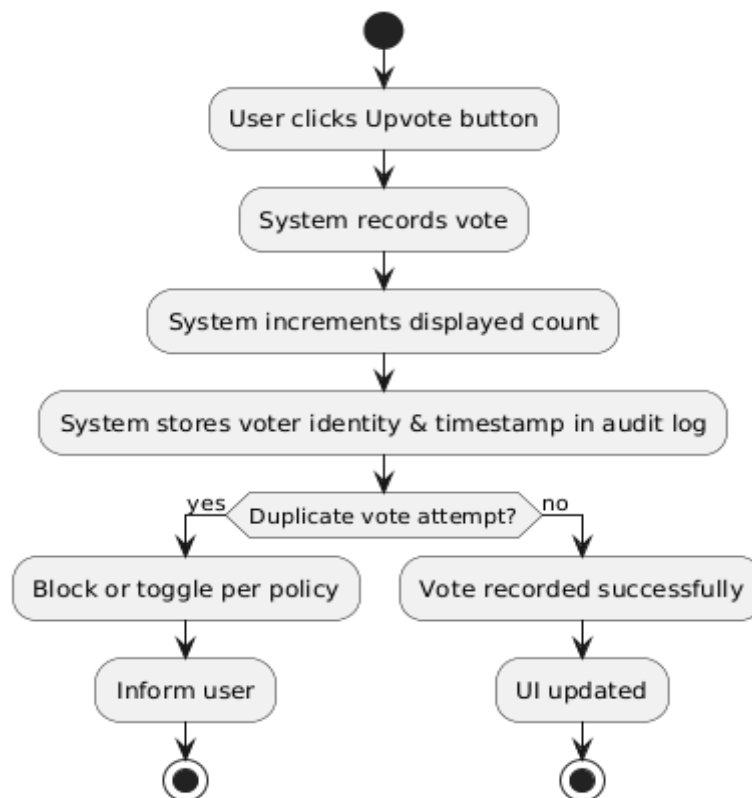
Figure 4.32 upvote activity diagram
