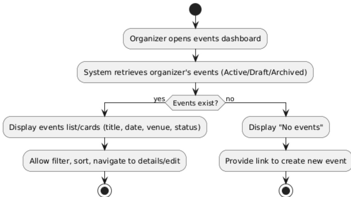
Figure 4.47 browse events (organizer) activity diagram
