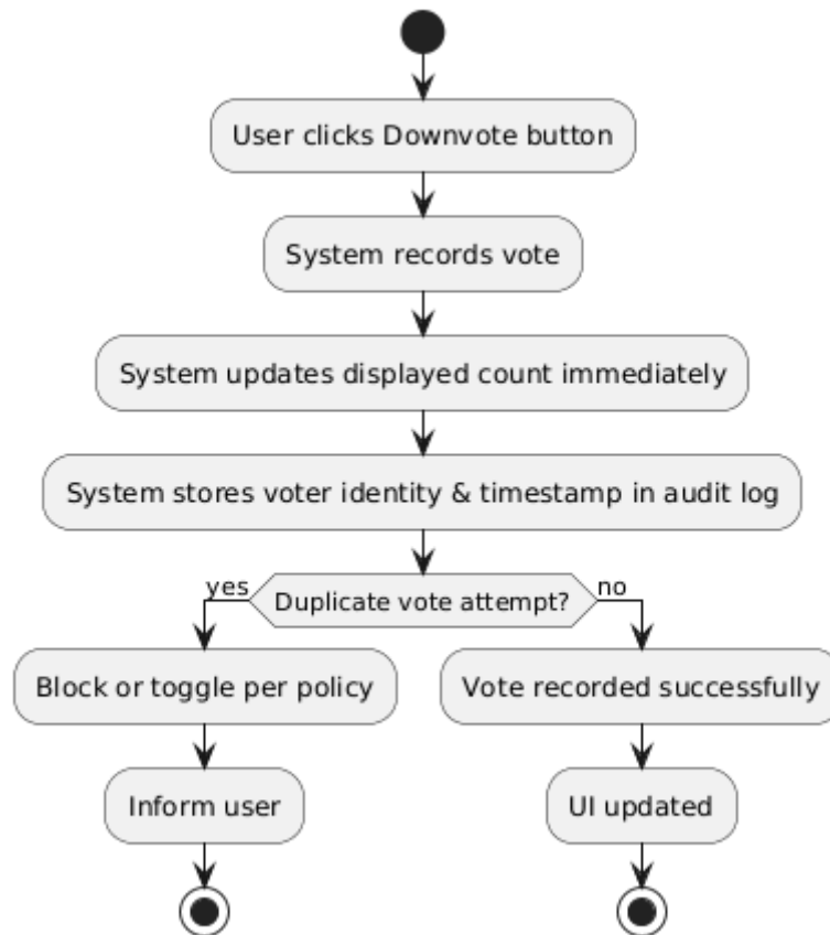
Figure 4.33 downvote activity diagram
