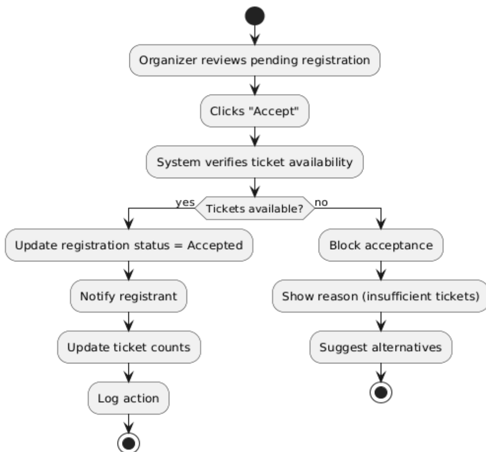
Figure 4.55 accept registration activity diagram
