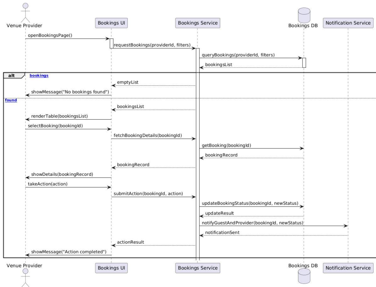
Figure 4.111 accept booking sequence diagram
