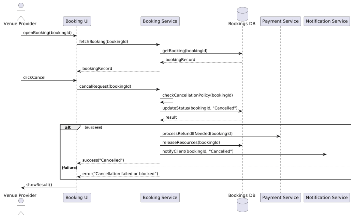
Figure 4.113 cancel booking sequence diagram
