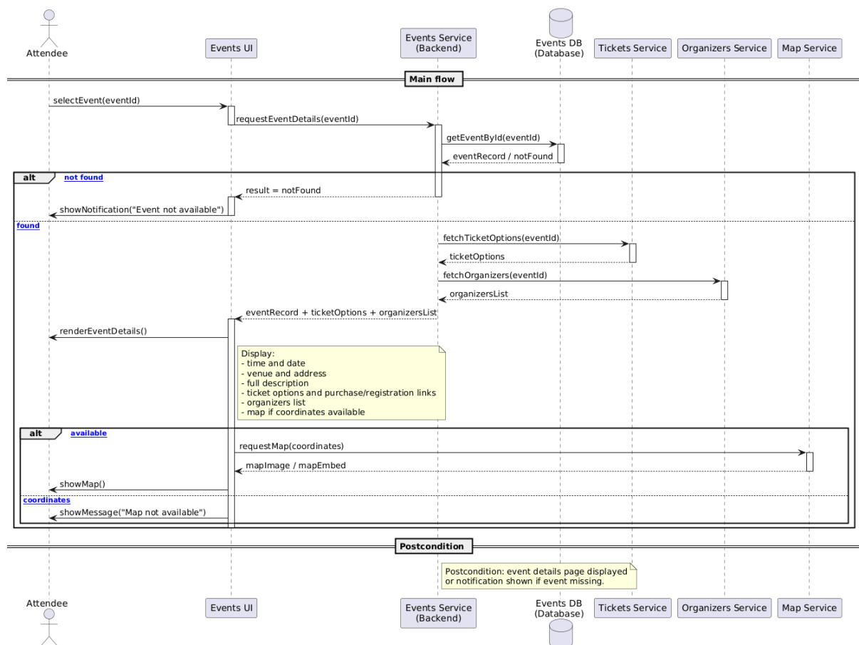
Figure 4.78 view events details sequence diagram
