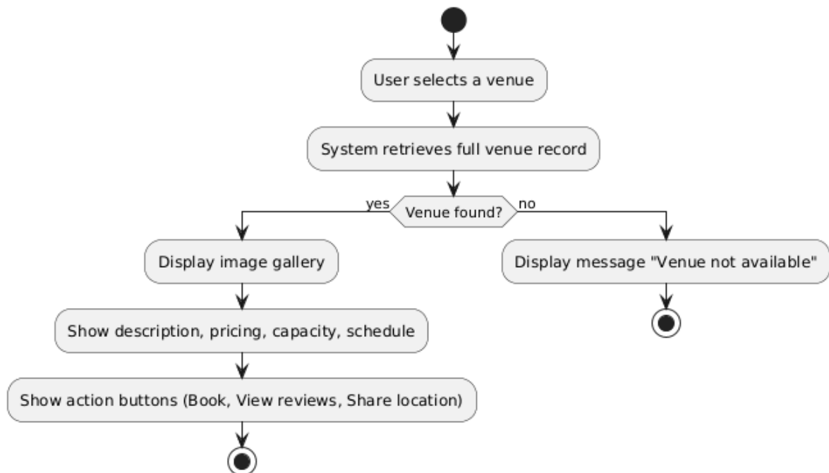
Figure 4.5 view venues details activity diagram
