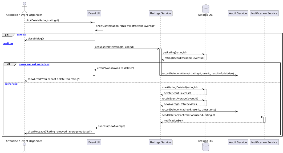
Figure 4.93 edit event rating sequence diagram
