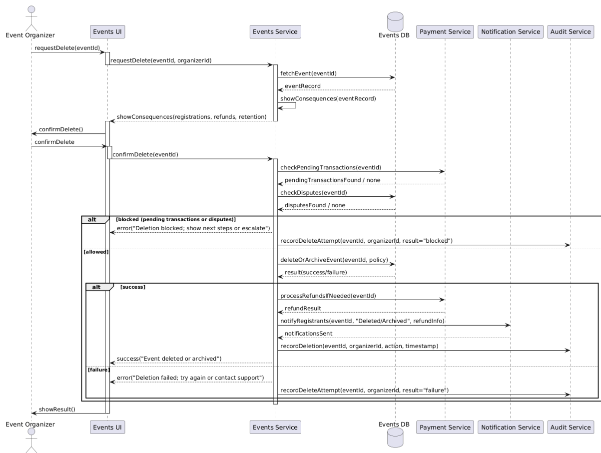
Figure 4.118 delete event sequence diagram
