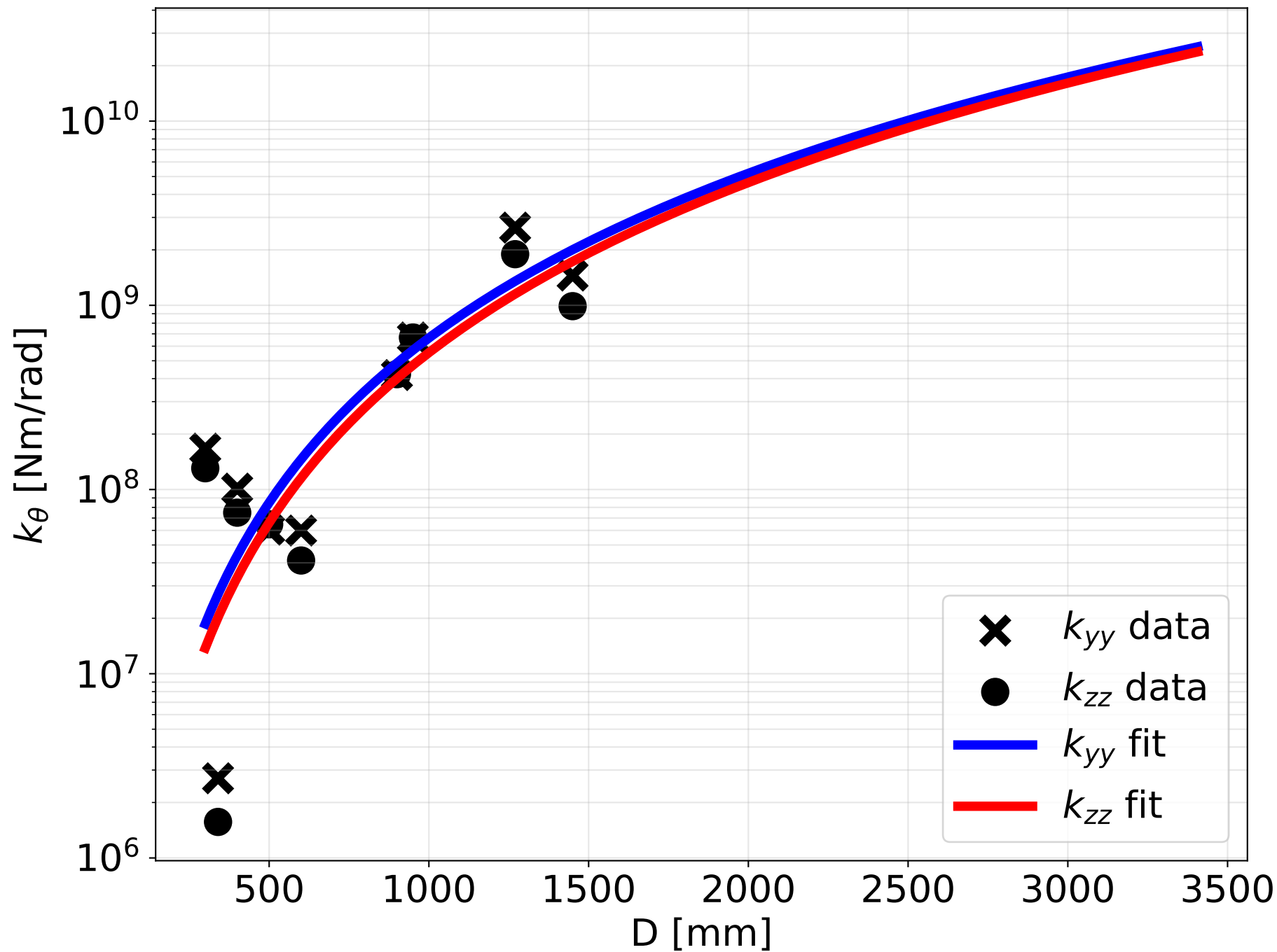
Power-law fit of TRB rotational stiffness
