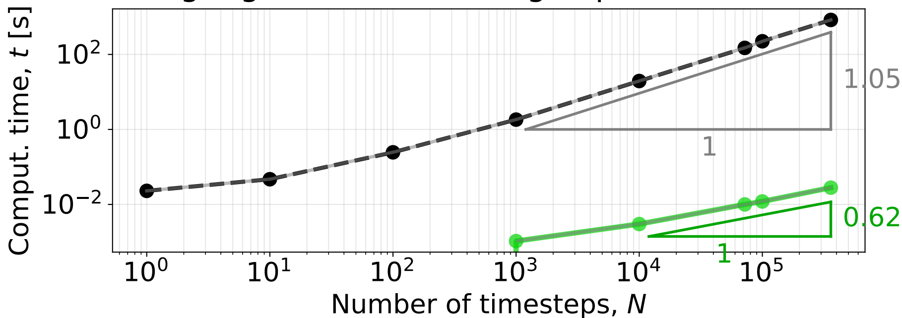
Log-log trend and scaling exponent ( t \sim N^p )
