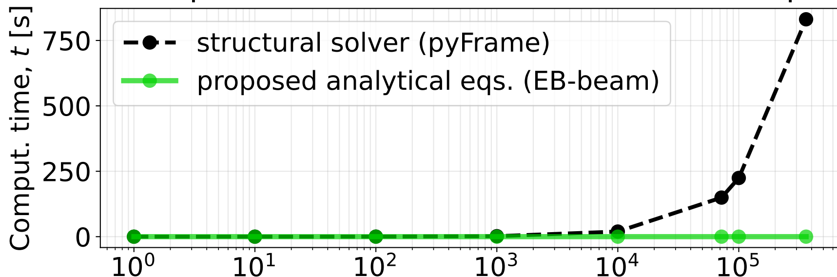
Computational time vs. Number of timesteps
