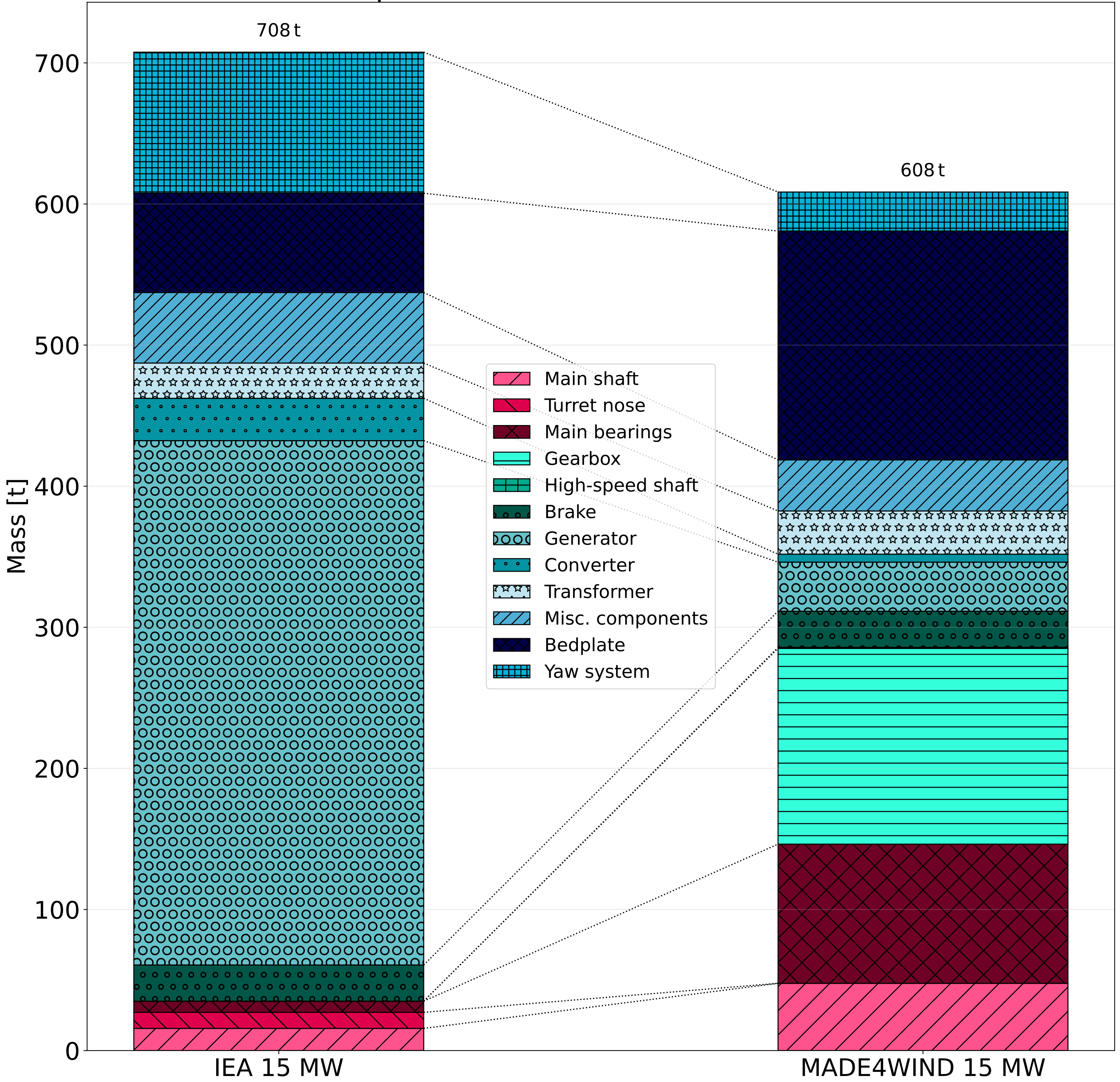
Comparison of nacelle mass distribution
