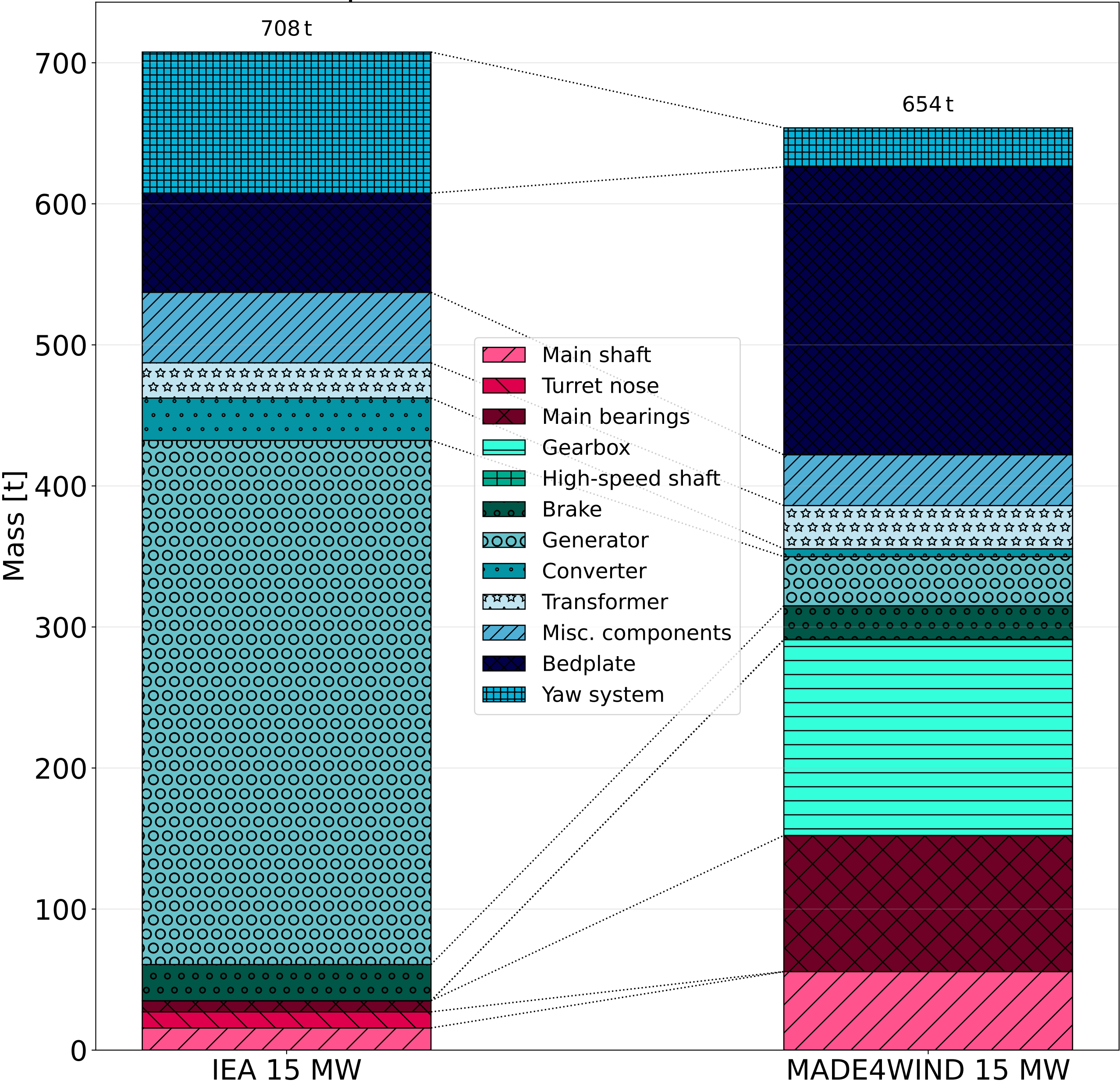
Comparison of nacelle mass distribution
