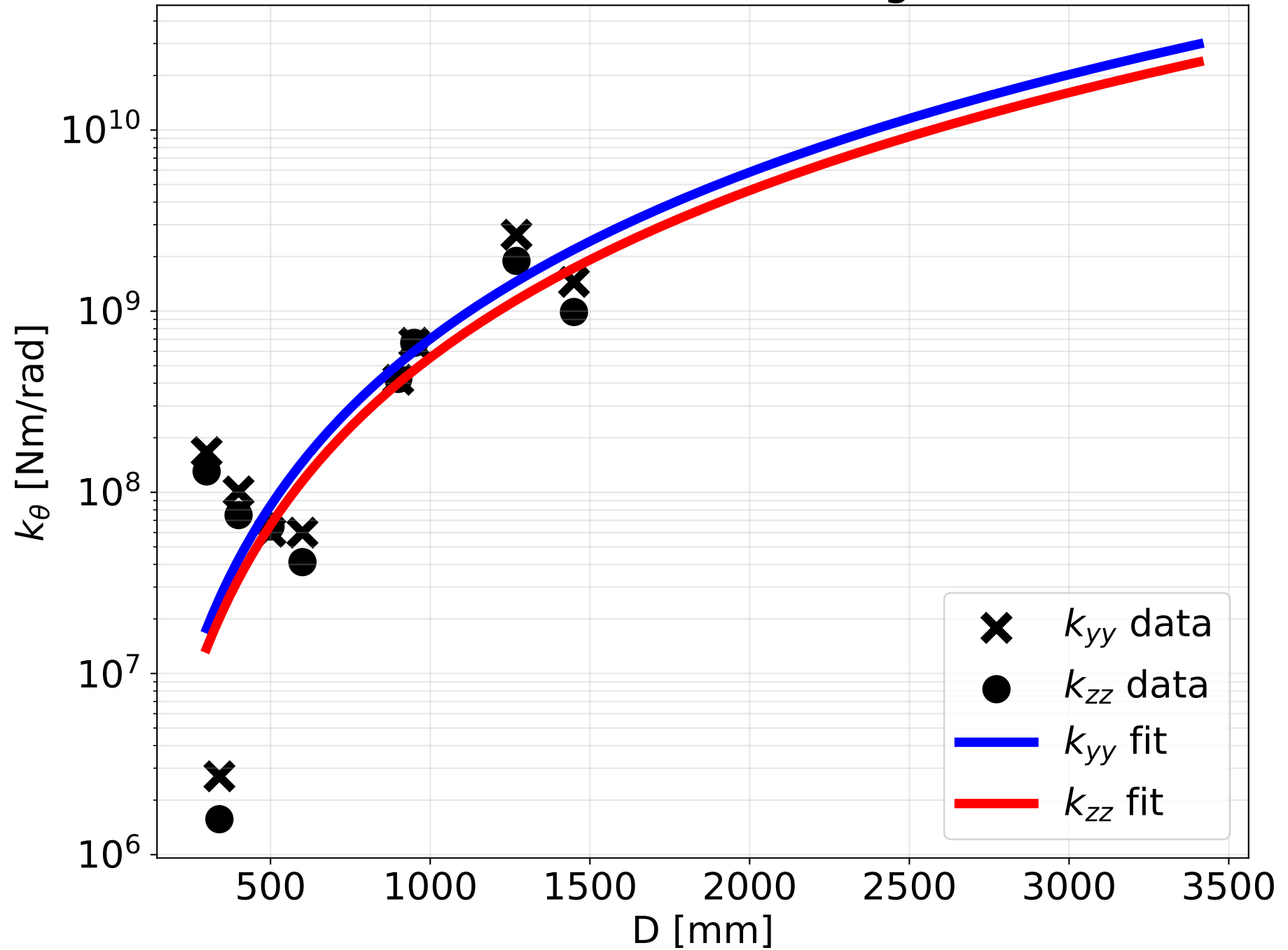
Power-law fit of TRB2 tilting stiffness
