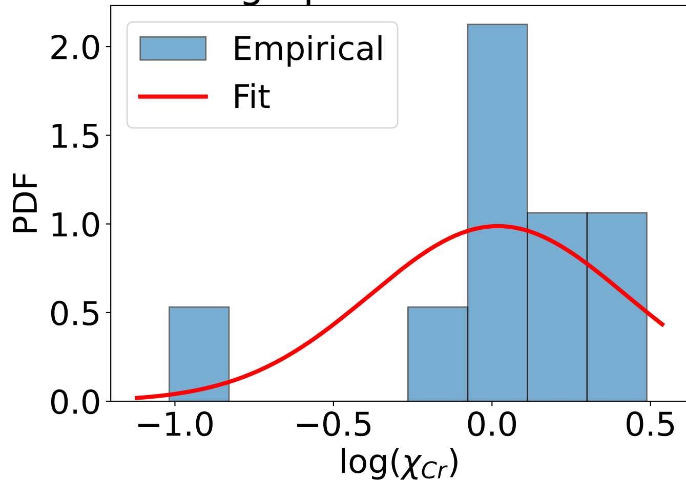
Log-Space Normal fit
