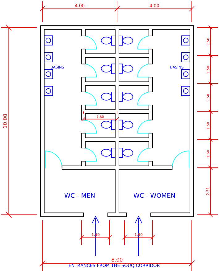
PUBLIC WC 1 (north-west) - 5 + 5 cubicles
