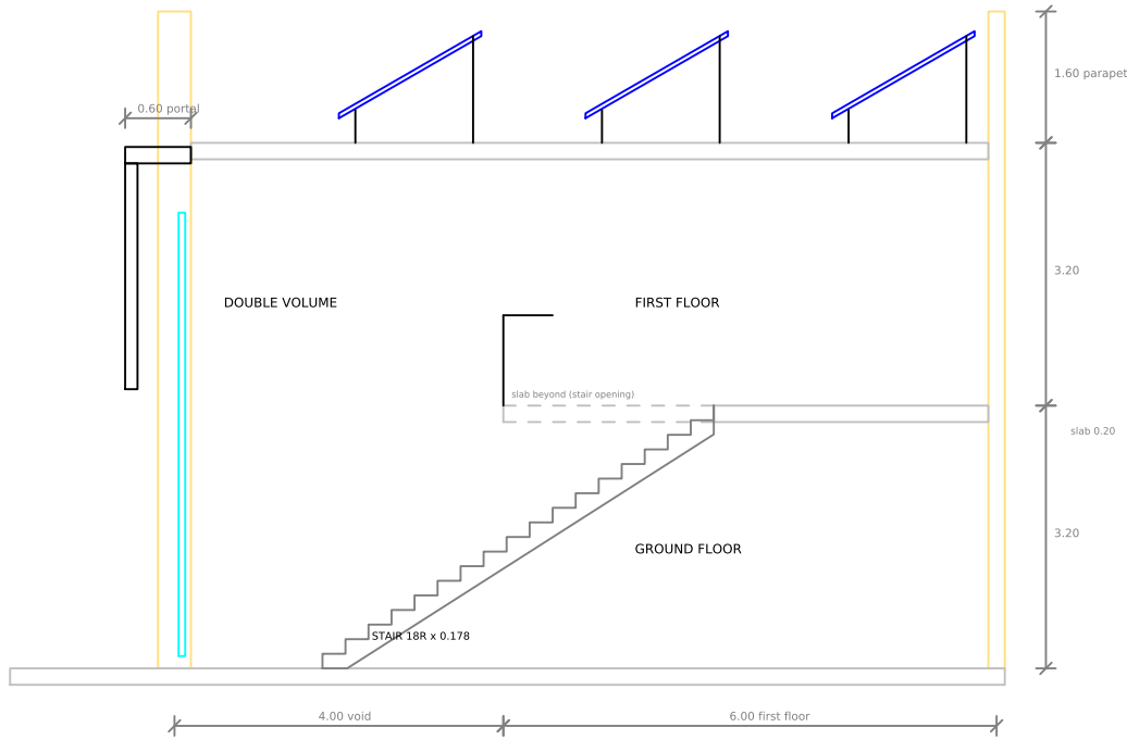
SECTION A-A (through stair)
