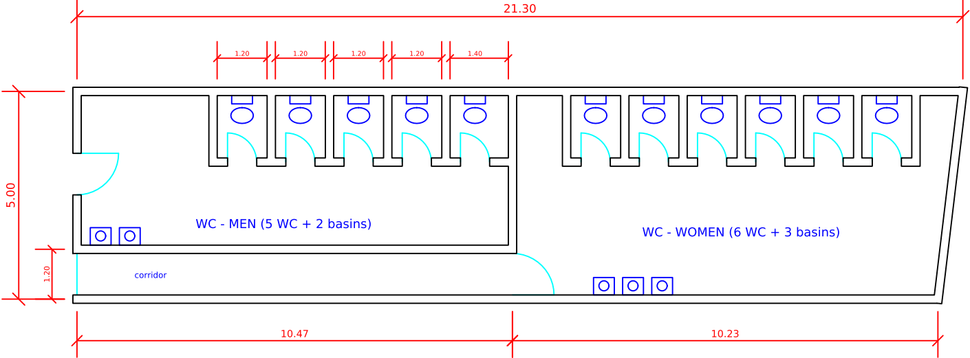
PUBLIC WC 2 (north-east) - men + women side by side
