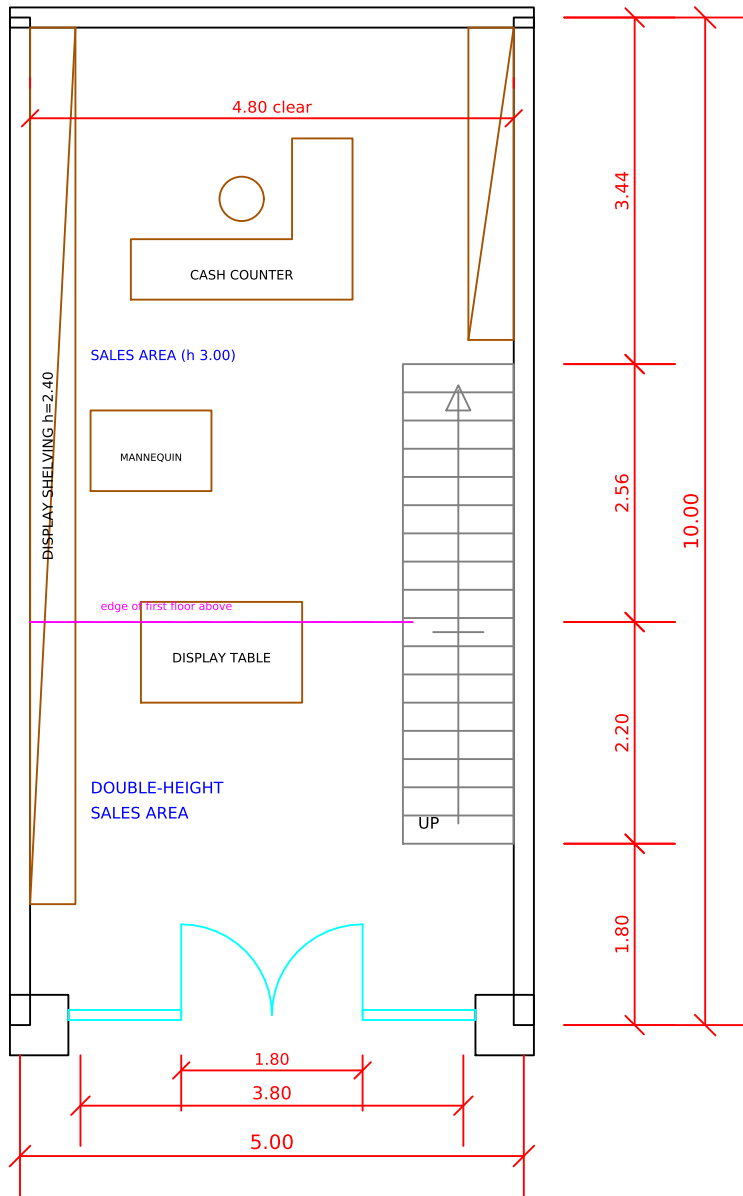
GROUND FLOOR PLAN (+0.00, 48 m2)
