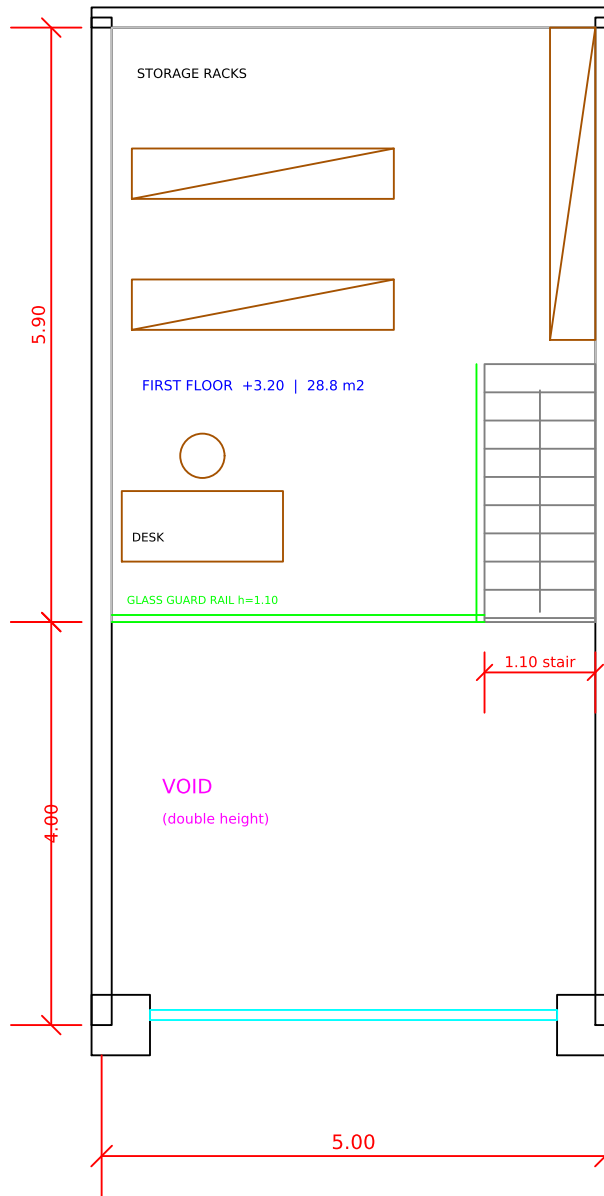
FIRST FLOOR PLAN (+3.20, 28.8 m2)
