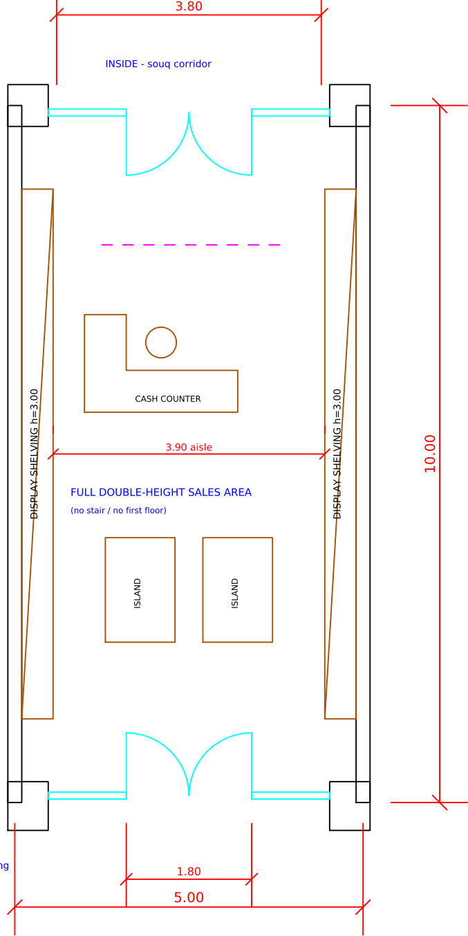
GROUND FLOOR PLAN (48 m2)
