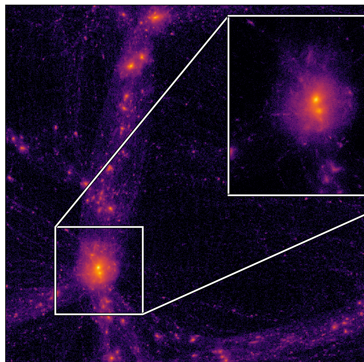
Astrolabe-Small, 10 steps
