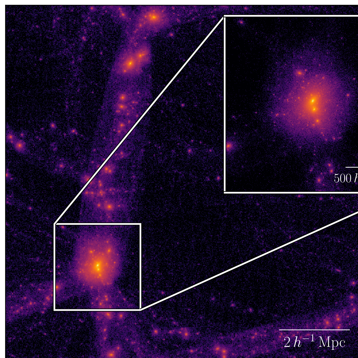
N-Body Simulation
