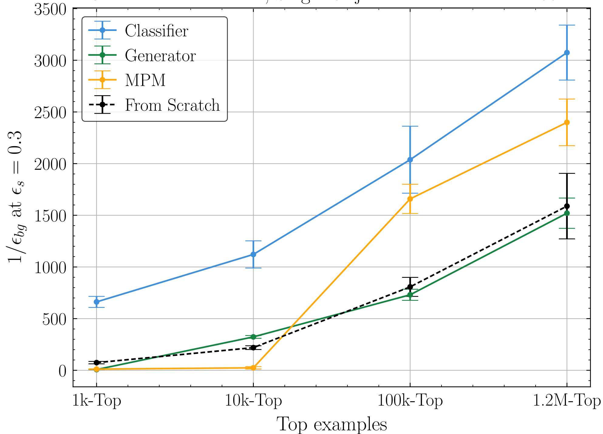
Omnilearned-Medium, Single Objective Pretrained on 100M
