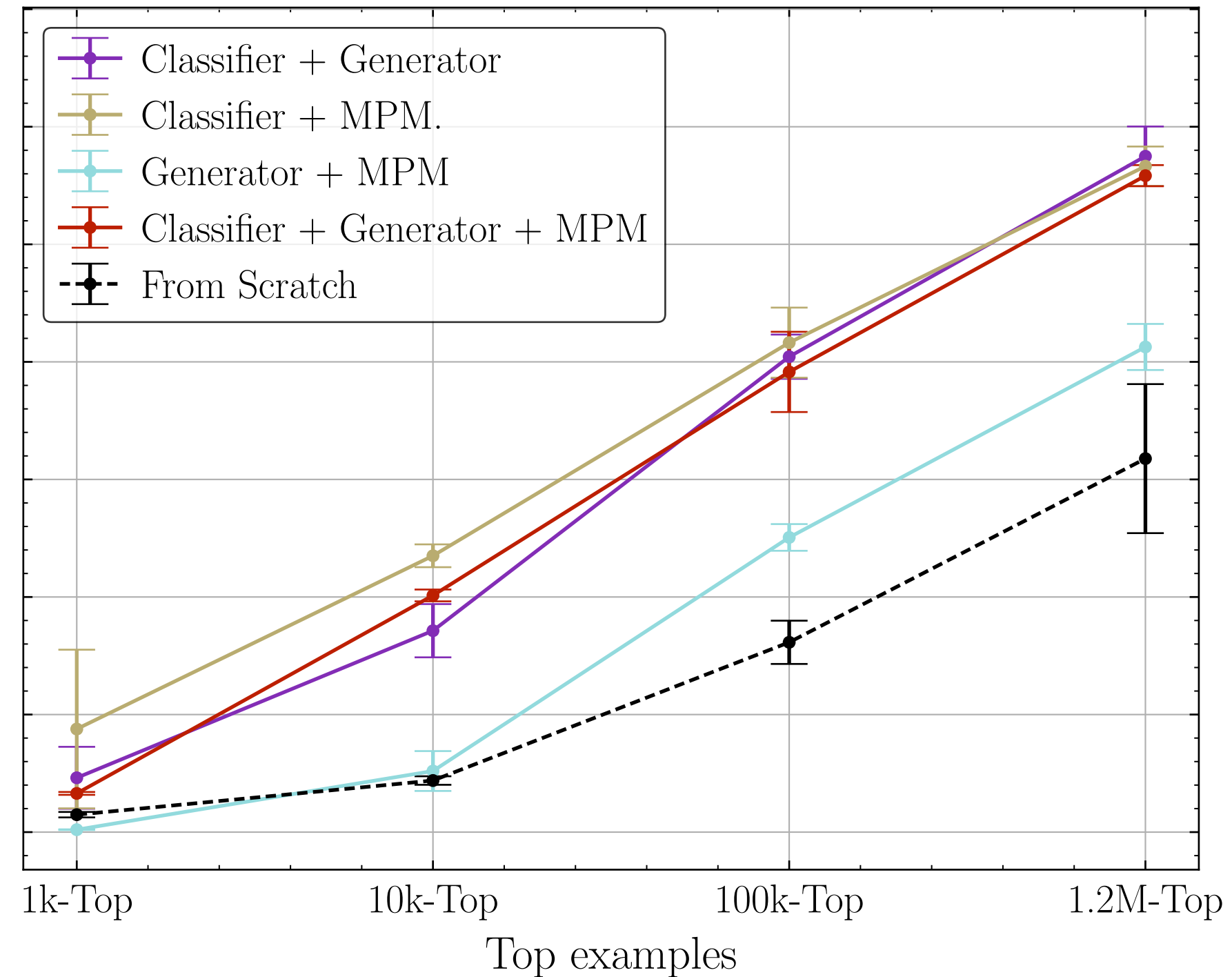
Omnilearned-Medium, Mult-Objective Pretrained on 100M
