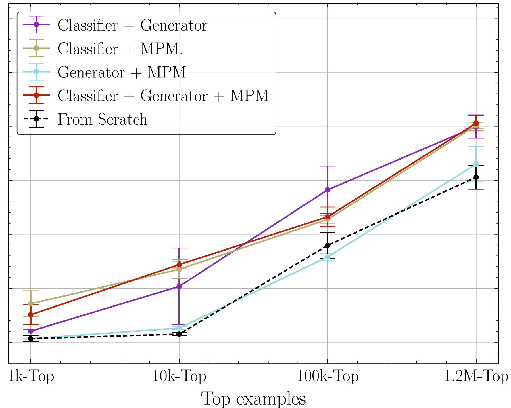
Omnilearned-Micro, Mult-Objective Pretrained on 100M
