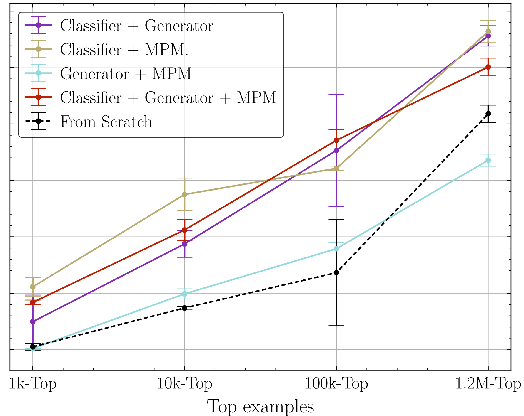
Omnilearned-Small, Mult-Objective Pretrained on 100M
