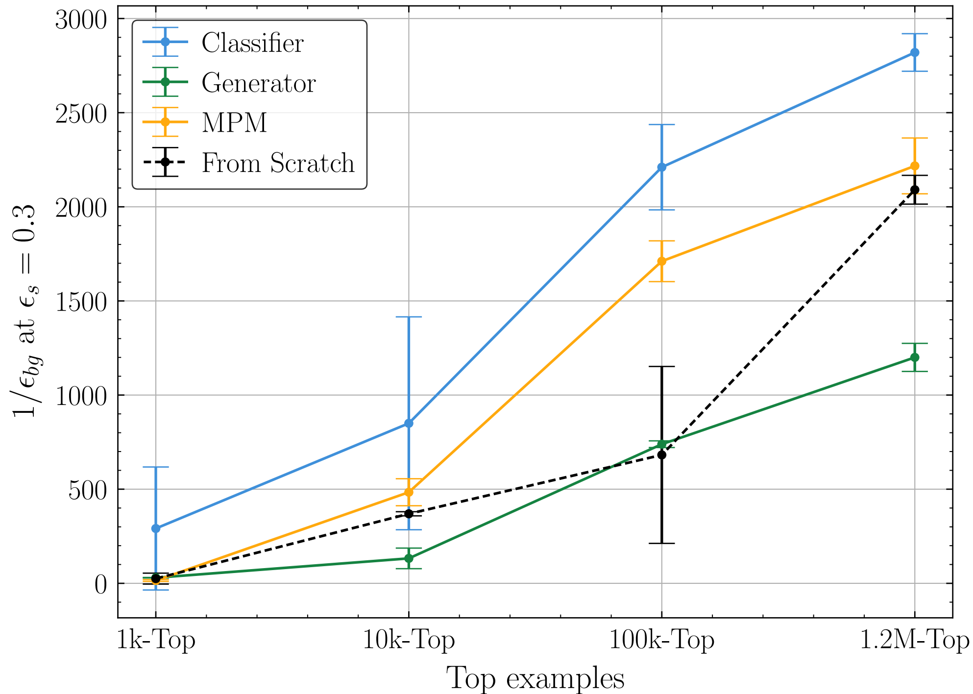
Omnilearned-Small, Single Objective Pretrained on 100M
