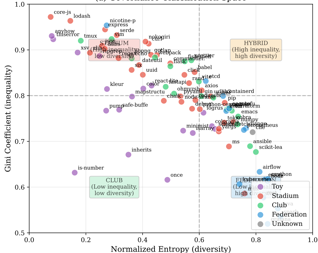
(a) Governance Classification Space
