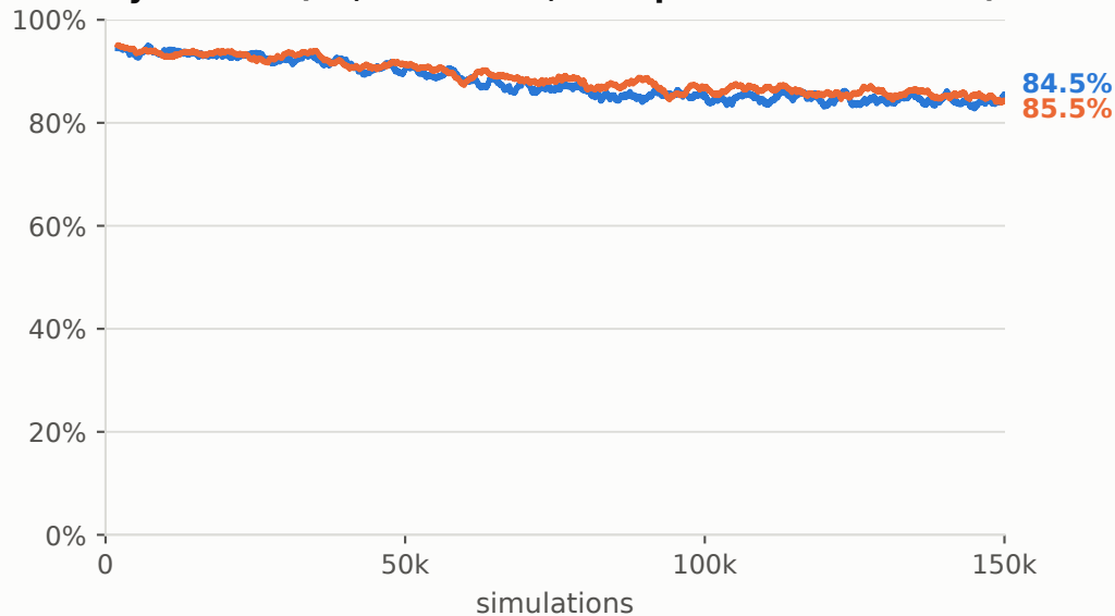
Pyrenees (84,431 of 150,000 episodes concurrent)
