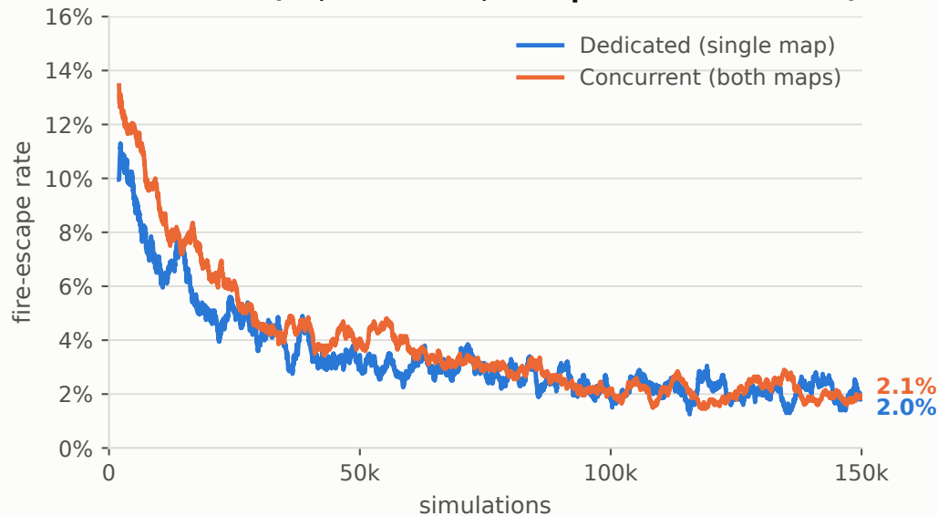
Palisades (65,569 of 150,000 episodes concurrent)
