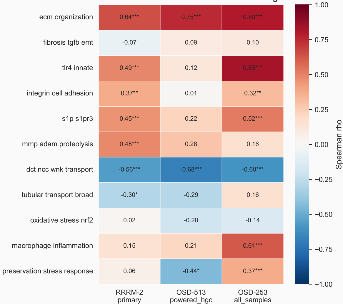
Mechanism scores associated with remodeling axis
