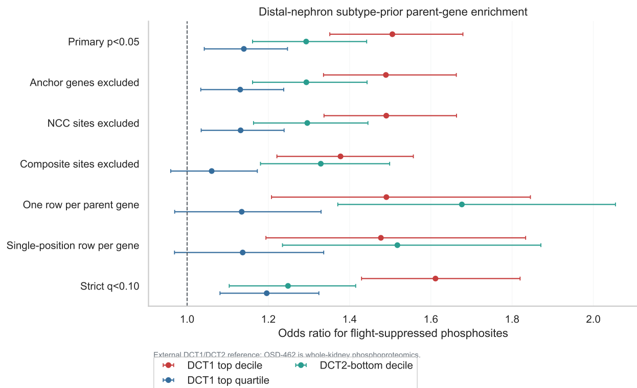
Figure S1: Distal-nephron subtype-prior parent-gene enrichment. DCT1 top-decile, DCT2-bottom-decile, and DCT1 top-quartile reference bins are tested across primary and sensitivity definitions. The safest claim is enrichment in distal-nephron subtype-prior extremes rather than DCT1 exclusivity.
