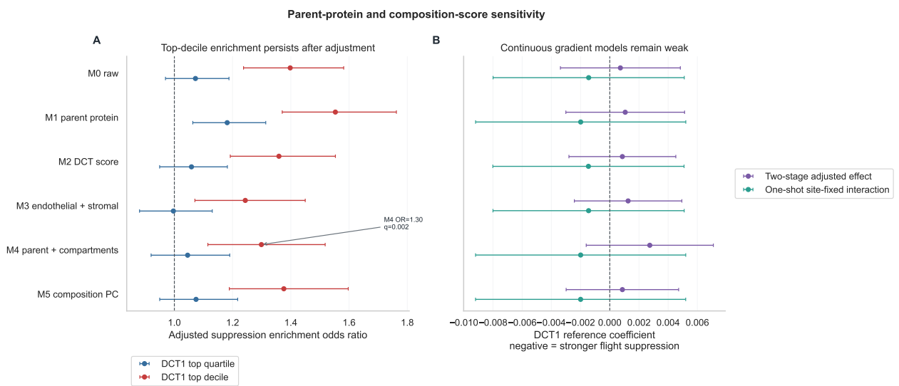
Figure S2: Parent-protein and composition-score sensitivity. Panel A shows top-decile and top-quartile enrichment across the adjustment ladder. Panel B shows that continuous DCT1-reference and flight-by-DCT1 interaction models remain weak.
