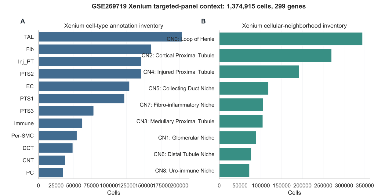
Figure S5: GSE269719 Xenium annotation inventory. The Xenium object provides targeted-panel annotation and cellular-neighborhood context, not whole-transcriptome pathway projection.
