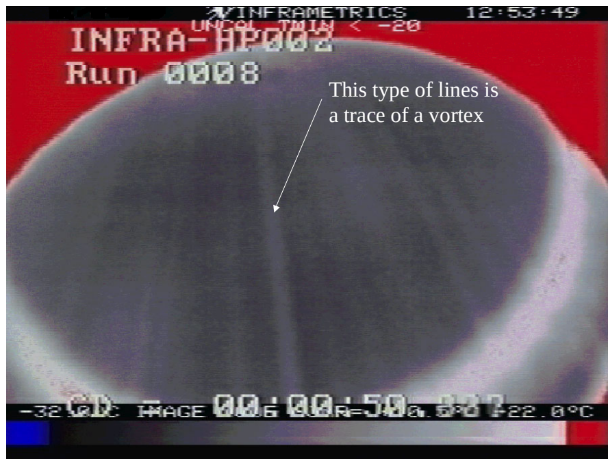
Figure 87. Infrared image: DLR TOP nozzle, vortex origin shortly after nozzle throat, experiment by Stark et al R 123 . (Courtesy of DLR and ASTRIUM)
