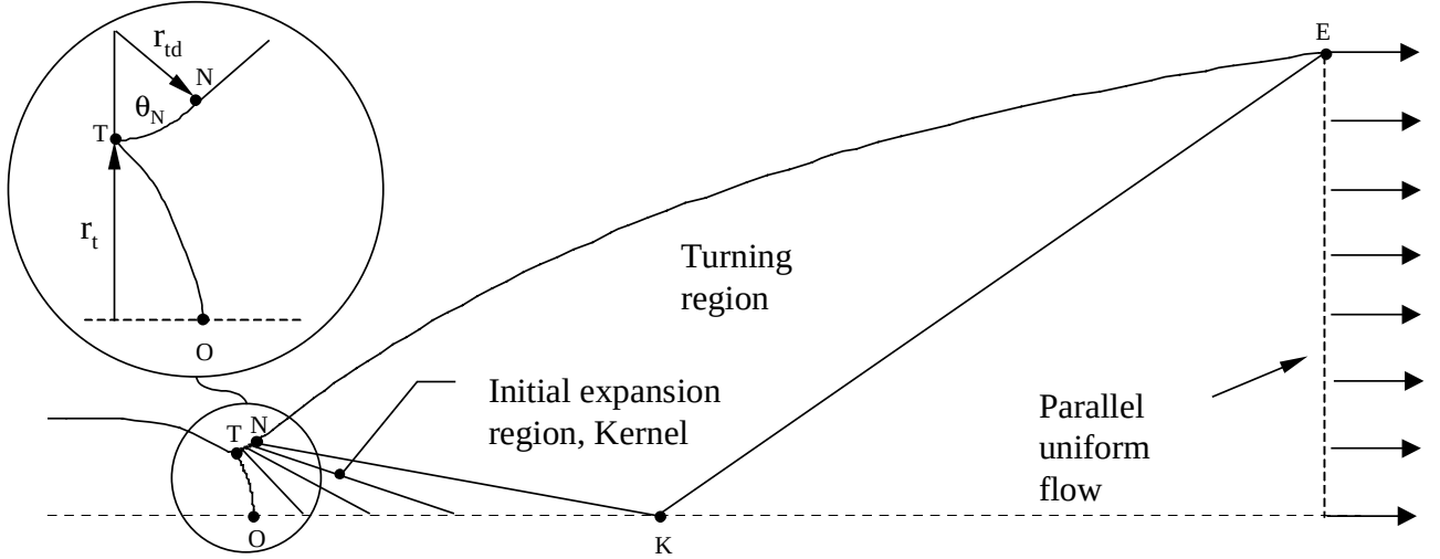
Figure 6. Basic flow structures in an ideal nozzle.
