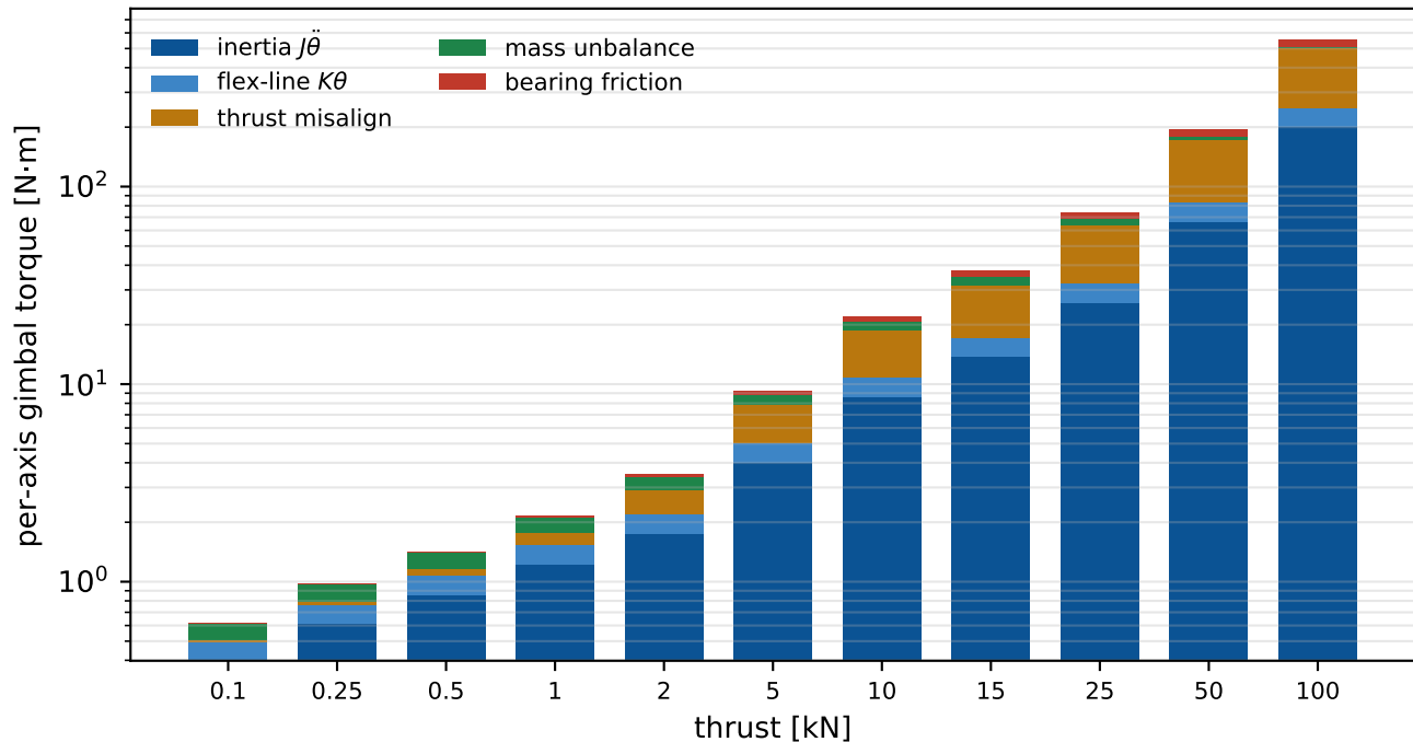
Gimbal torque budget, \pm 5^\circ at 4 Hz, 316L shell, pivot at throat
