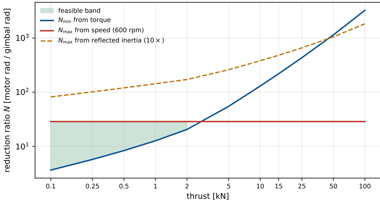
Two NEMA 17 steppers: the feasible band in N closes at \approx 3 kN
