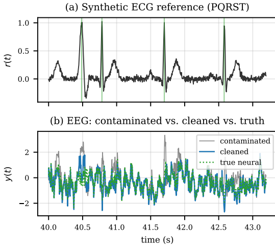
Fig. 2. Time-domain cancellation over three beats (converged, buffered mode). (a) Synthetic ECG reference r(t) with full PQRST morphology; vertical lines mark detected R fiducials t_k . (b) Contaminated EEG y(t) , cleaned output, and ground-truth neural signal s(t) over the same window.
