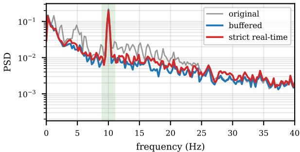
(b) Spectrum: original, buffered, and strict real-time
