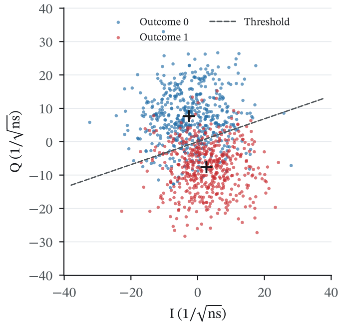
Fridge output at 6.5 GHz · 100 \mu s integration
