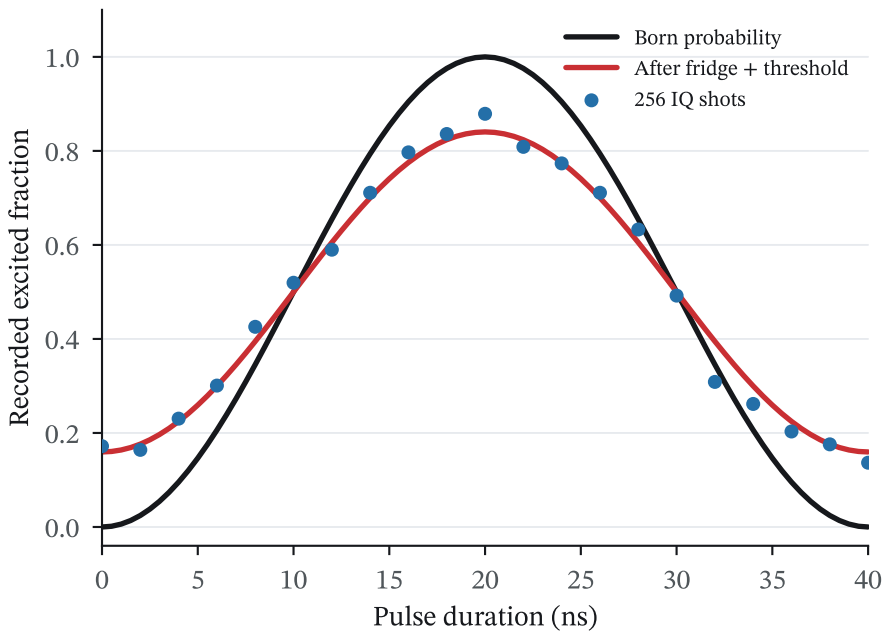
Fridge output at 6.5 GHz · 100 \mu s integration
