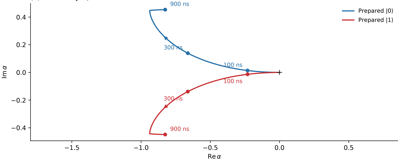
(b) Intracavity IQ in the drive frame
