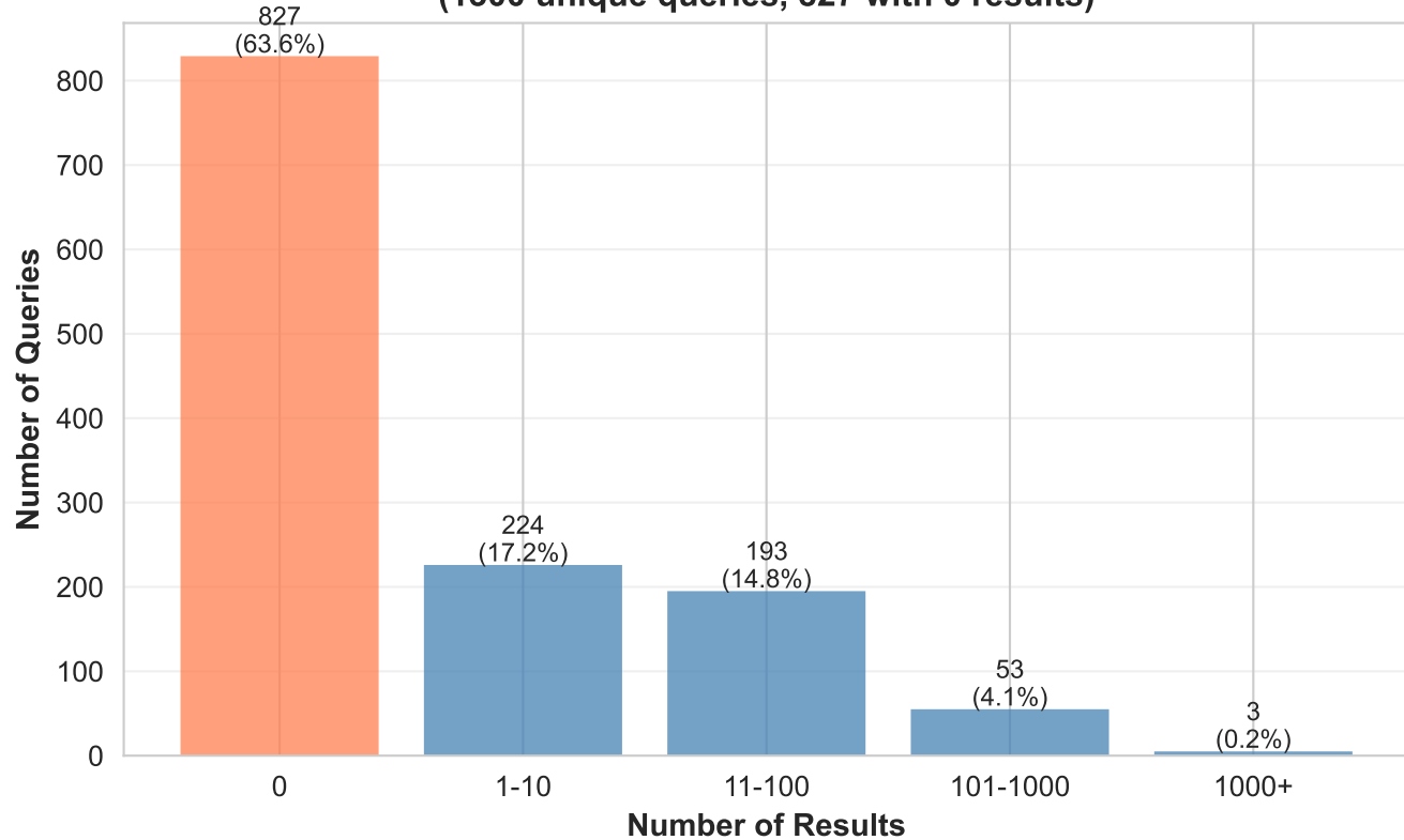
2M Dataset (Deduplicated) (1300 unique queries, 827 with 0 results)
