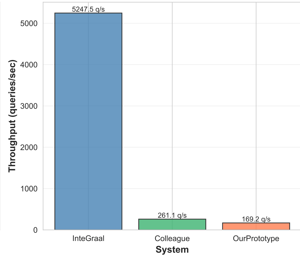
Query Throughput
