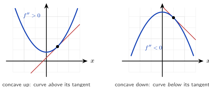
Figure 13.6 The tangent test for concavity. A tangent (scarlet) touches the curve at one point and then
