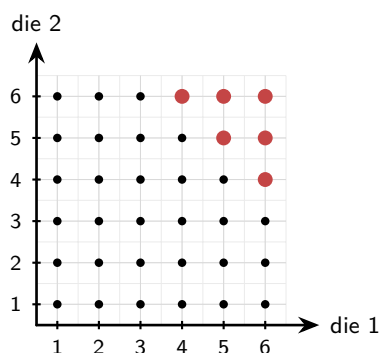
Figure 11.3 The 36 equally likely outcomes of rolling two dice. The six larger scarlet points are the outcomes whose total is at least 10.
