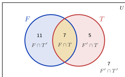
Figure 11.1 The four regions of a two-event Venn diagram, with the class of 30 filled in. Football only is F \cap T' , both is F \cap T , tennis only is F' \cap T , and neither is F' \cap T' , the region outside both circles. The four counts add to 30.
