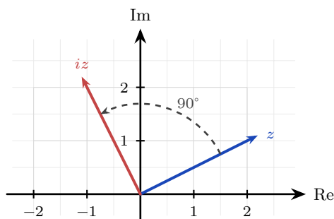
Figure 17.5 Multiplying by i turns a complex number through a quarter-turn anticlockwise about the origin, leaving its modulus unchanged.
