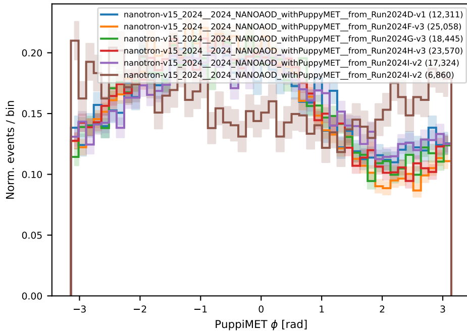
DoubleMuonLowMass5
