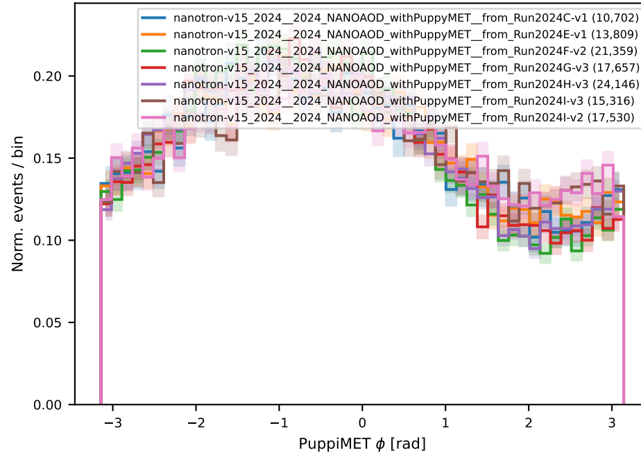
DoubleMuonLowMass2
