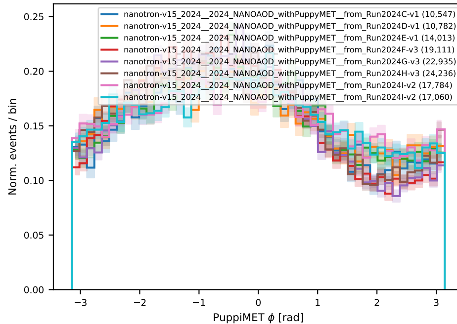
DoubleMuonLowMass6
