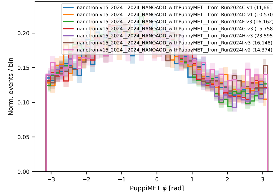
DoubleMuonLowMass3
