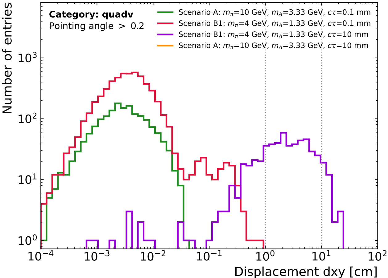
CMS Simulation Preliminary (13.6 TeV, 2024)
