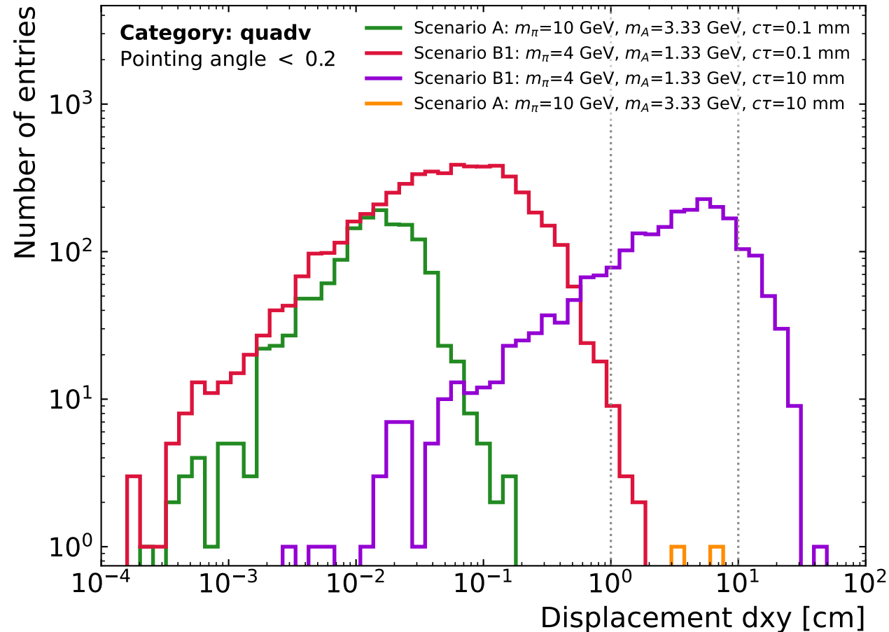
CMS Simulation Preliminary (13.6 TeV, 2024)
