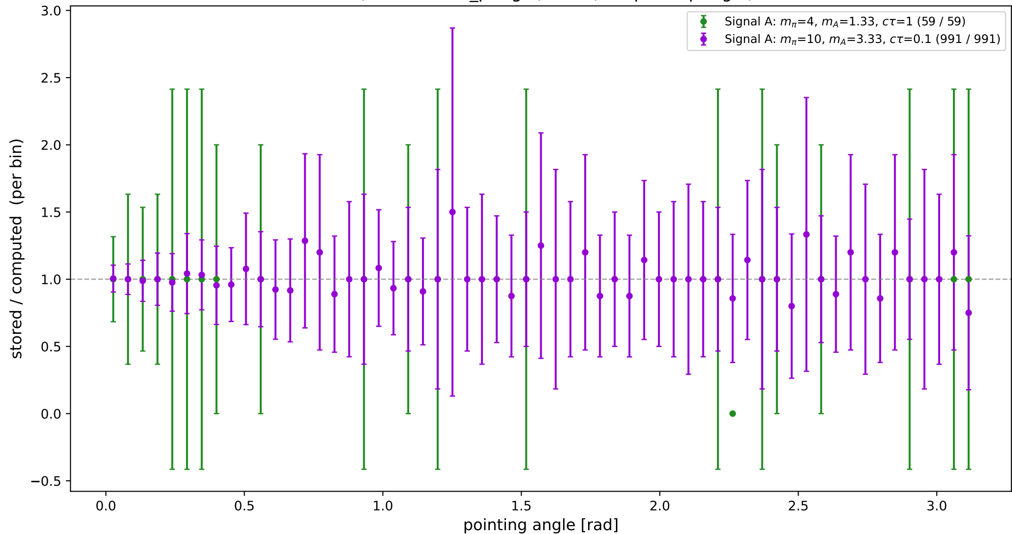
Bin-by-bin ratio of the pointing-angle histograms \text{hist}(\text{fourmuonSV\_pAngle}) / \text{hist}(\text{computed pAngle})
