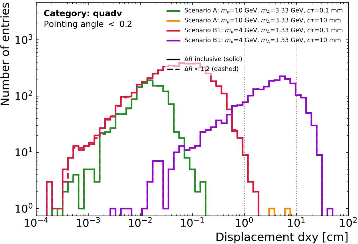
CMS Simulation Preliminary (13.6 TeV, 2024)
