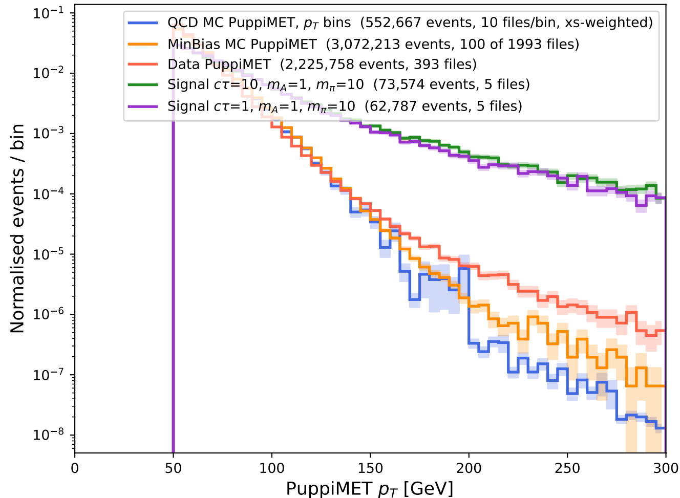
PuppiMET p_T : QCD MC vs Data (v2) [PuppiMET p_T > 50 GeV]
