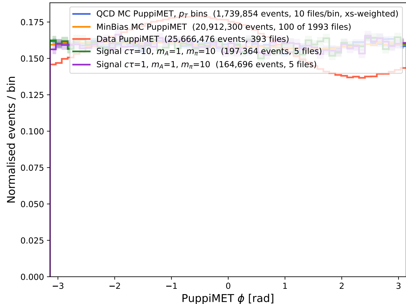
PuppiMET \phi : QCD MC vs Data (v2) [inclusive]
