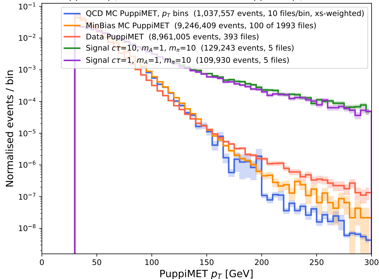
PuppiMET p_T : QCD MC vs Data (v2) [PuppiMET p_T > 30 GeV]
