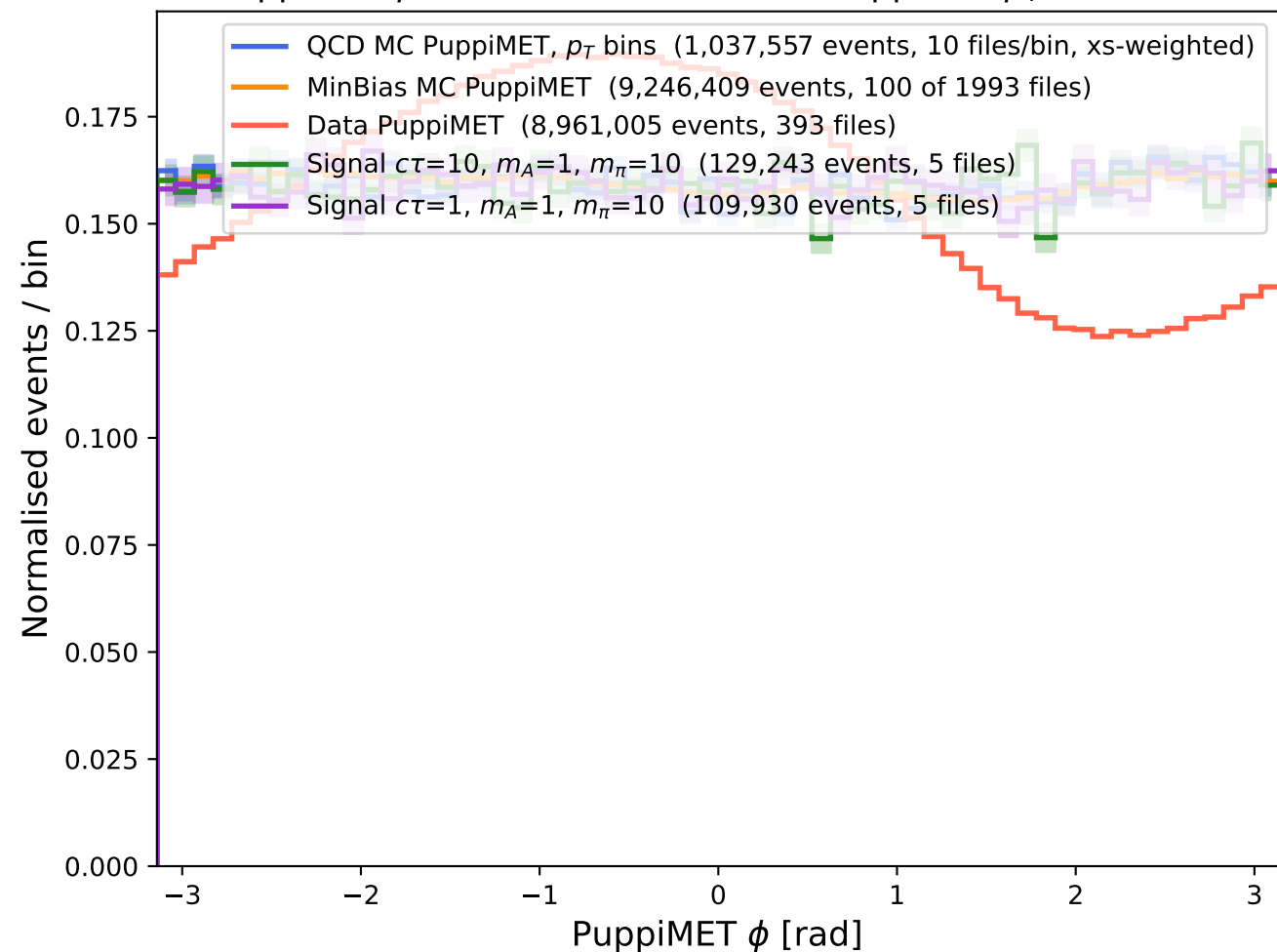
PuppiMET \phi : QCD MC vs Data (v2) [PuppiMET p_T > 30 GeV]
