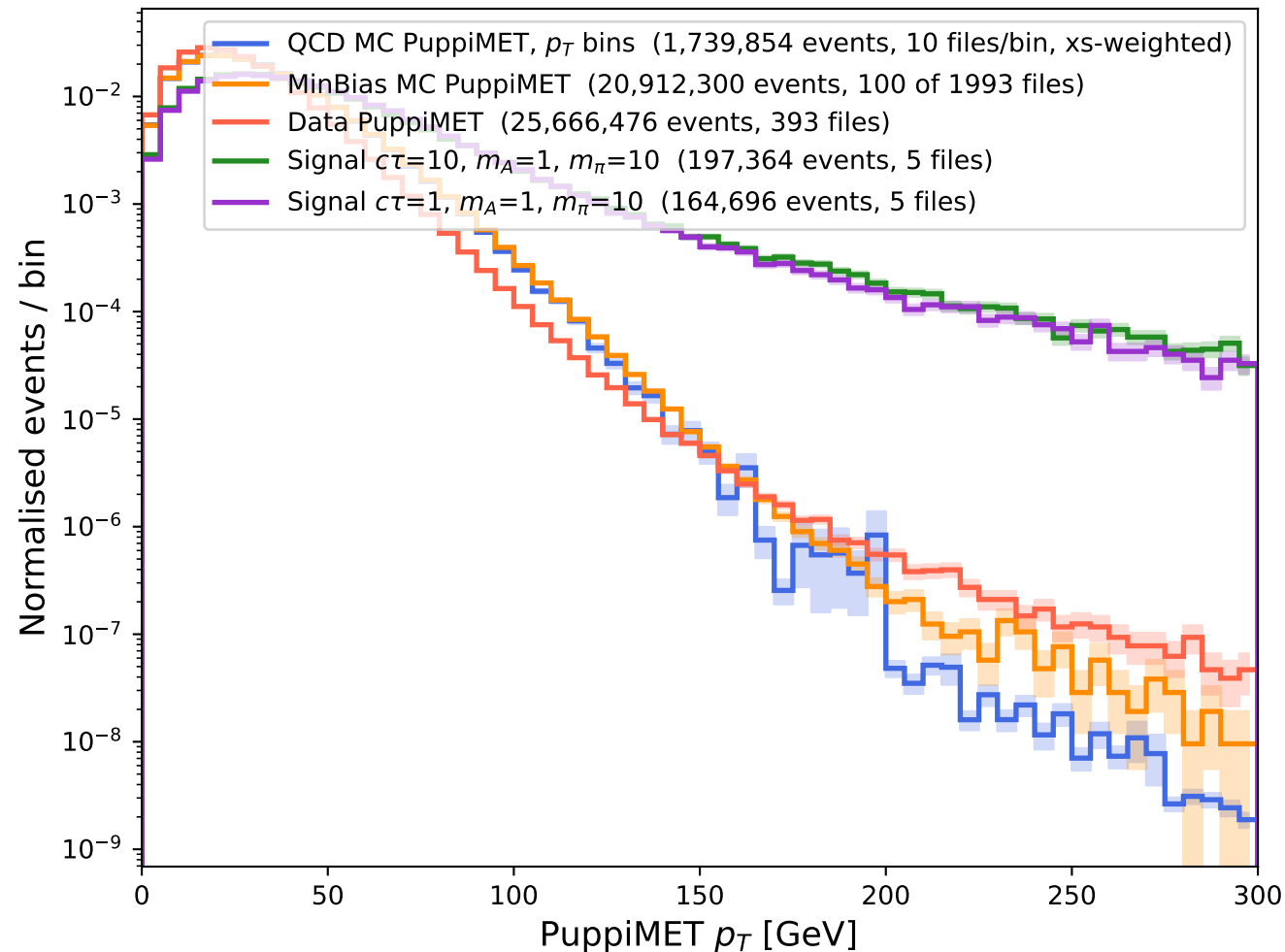
PuppiMET p_T : QCD MC vs Data (v2) [inclusive]
