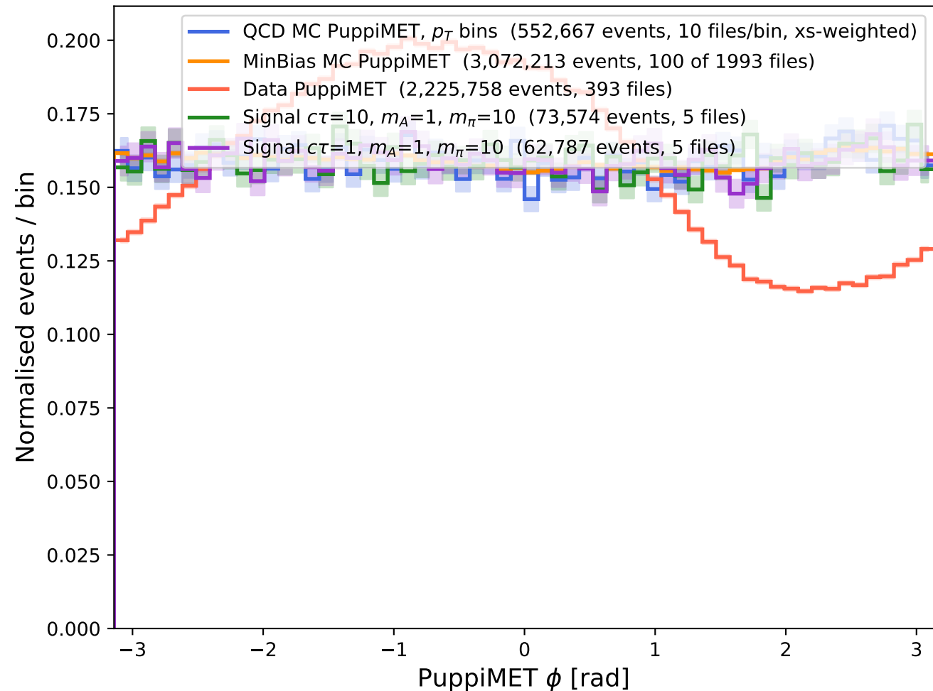
PuppiMET \phi : QCD MC vs Data (v2) [PuppiMET p_T > 50 GeV]
