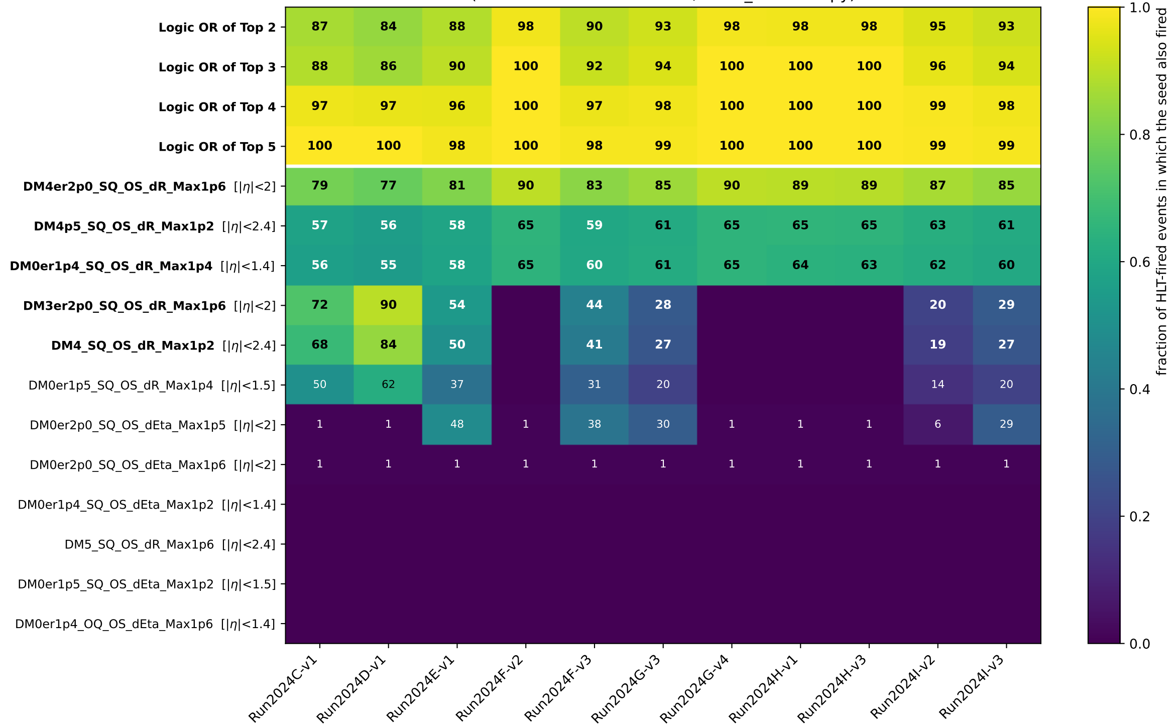
HLT_DoubleMu4_3_LowMass contribution of each L1 seed [%], by era (bold = enabled in modules/muon_selection.py)
