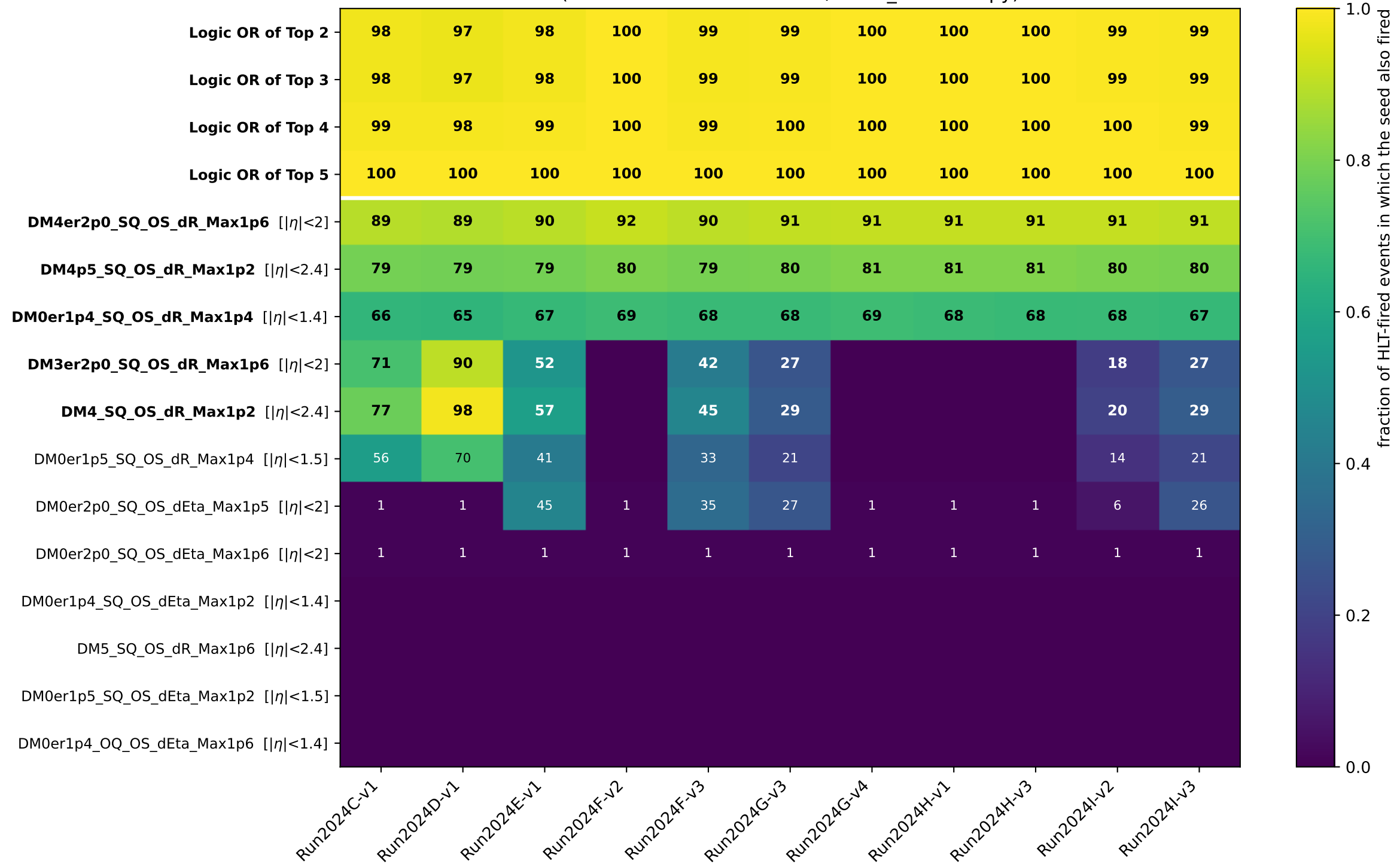
HLT_DoubleMu4_LowMass_Displaced contribution of each L1 seed [%], by era (bold = enabled in modules/muon_selection.py)
