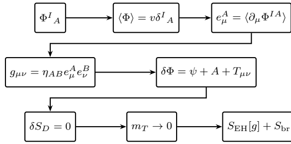
Figure 1.2: The NAMCG derivation spine used in this book. A single scalar phase cannot lock internal indices to local Lorentz frames.
