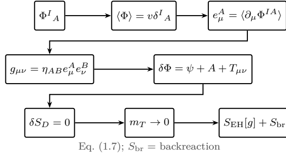
Figure 1.2: The NAMCG derivation spine used in this book. A single scalar phase cannot lock internal indices to local Lorentz frames.
