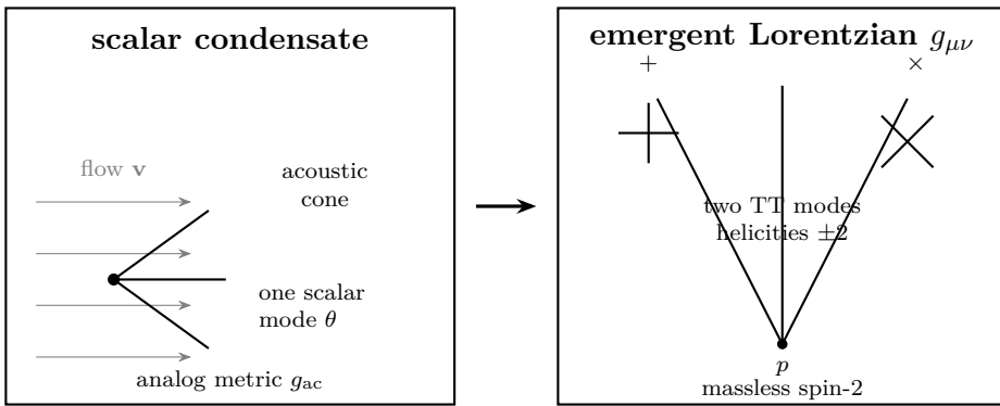
Figure 1.1: A scalar order parameter supplies an acoustic metric. It does not supply the two massless spin-2 polarizations of general relativity.
