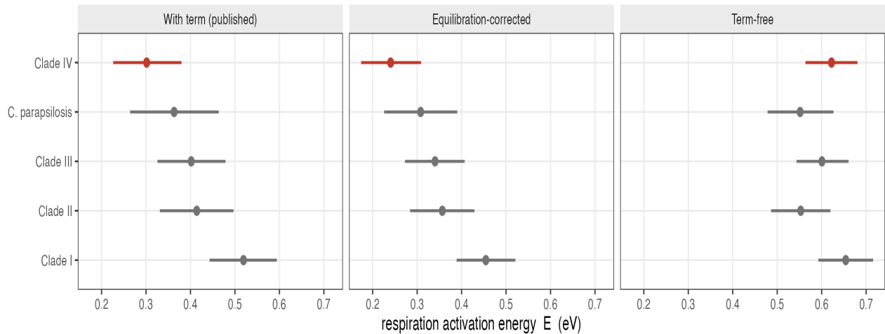
Supplementary Figure 6. The between-clade respiration activation energy under three treatments of the inoculum back-projection. Each panel shows the hierarchical Bayesian Arrhenius activation energy E_R per clade (posterior median; bars, 95% credible interval), refitting the same model under: (left) the published back-projection, N_0 = N_{\text{inoc}} \cdot \exp(r \cdot \Delta t) ; (centre) the equilibration-corrected N_0 , recomputed from the logged internal vial temperature over the onset window; and (right) the term removed entirely, N_0 = N_{\text{inoc}} . The C. auris -versus- C. parapsilosis separation is preserved across all three, but the finer ordering within C. auris is not: Clade IV holds the lowest activation energy under the published and equilibration-corrected treatments and moves to fourth of five when the term is removed. The term-free case is not the physical null (the inoculum grows before the fit window), so it bounds the correction from the opposite side rather than representing the correct value; it is shown to make the dependence explicit. Generated by scripts/18_n0_treatment_panel.R .
