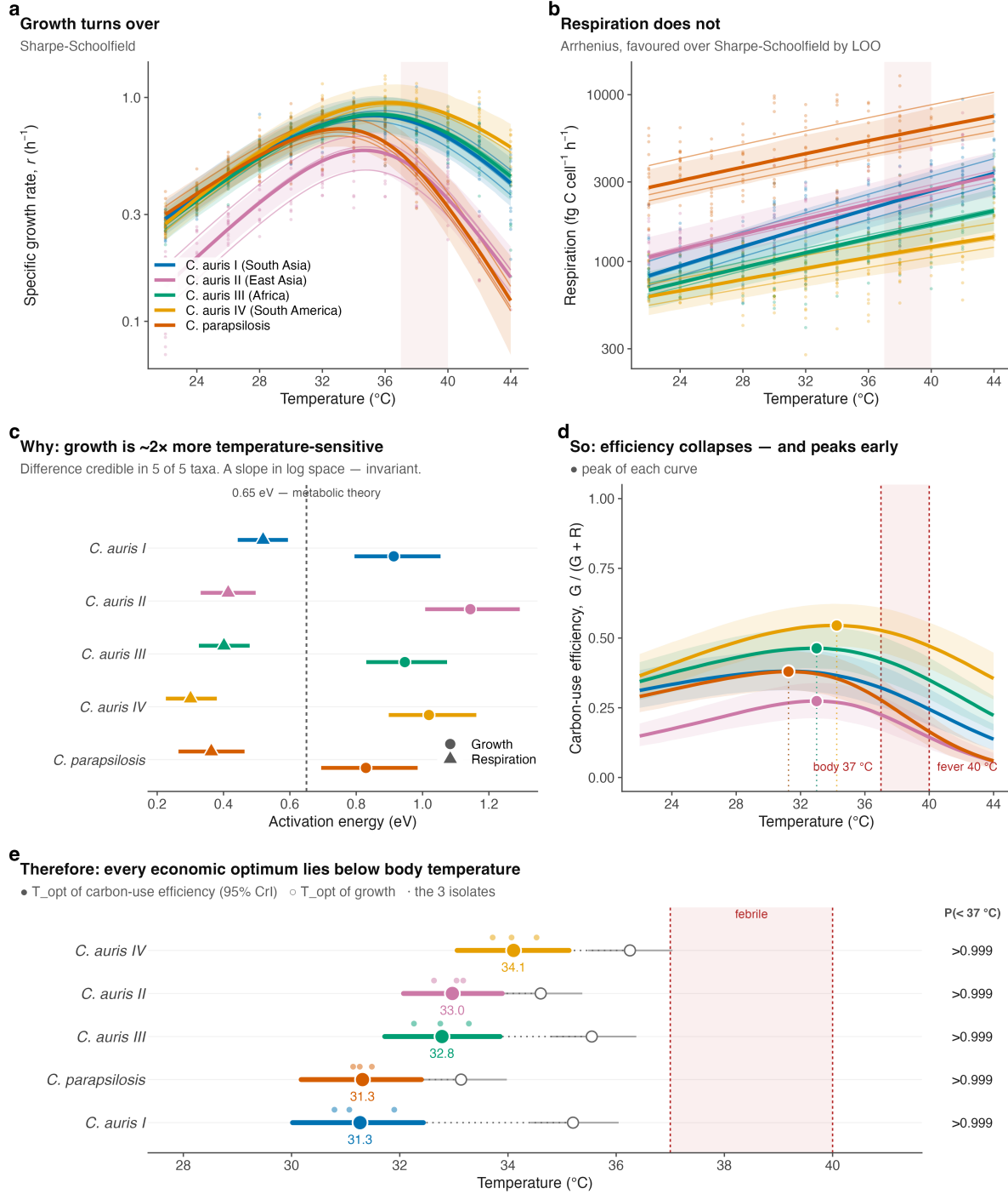
62 Figure 1. Growth and respiration decouple with temperature, placing every carbon-economy 63 optimum below body temperature. (a) Specific growth rate r ( \text{h}^{-1} ) and (b) per-cell respiration carbon 64 flux ( \text{fg C cell}^{-1} \text{h}^{-1} ) versus temperature (points, isolate-level observations; thin lines, per-isolate fits; bold lines, 65 clade-level posterior medians; bands, 95% CrI). Growth turns over; respiration does not (Arrhenius favoured 66 over Sharpe-Schoolfield by leave-one-out cross-validation). (c) Activation energies of growth (circles) and 67 respiration (triangles); dashed line, the 0.65 eV metabolic-theory value. Growth is credibly more temperature- 68 sensitive than respiration in all five taxa. (d) Carbon-use efficiency, \text{CUE} = G/(G+R) , collapses with 69 warming and peaks early; filled points mark each curve's peak. (e) Thermal optimum of CUE (filled points,
