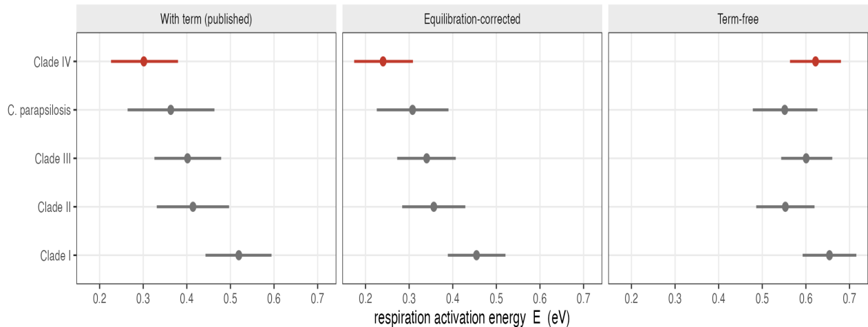
Supplementary Figure 4. The between-clade respiration activation energy under three treatments of the inoculum back-projection. Each panel shows the hierarchical Bayesian Arrhenius activation energy E_R per clade (posterior median; bars, 95% credible interval), refitting the same model under: (left) the published back-projection, N_0 = N_{\text{inoc}} \cdot \exp(r \cdot \Delta t) ; (centre) the equilibration-corrected N_0 , recomputed from the logged internal vial temperature over the onset window; and (right) the term removed entirely, N_0 = N_{\text{inoc}} . The C. auris -versus- C. parapsilosis separation is preserved across all three, but the finer ordering within C. auris is not: Clade IV holds the lowest activation energy under the published and equilibration-corrected treatments and moves to fourth of five when the term is removed. The term-free case is not the physical null (the inoculum grows before the fit window), so it bounds the correction from the opposite side rather than representing the correct value; it is shown to make the dependence explicit. Generated by scripts/18_n0_treatment_panel.R .
