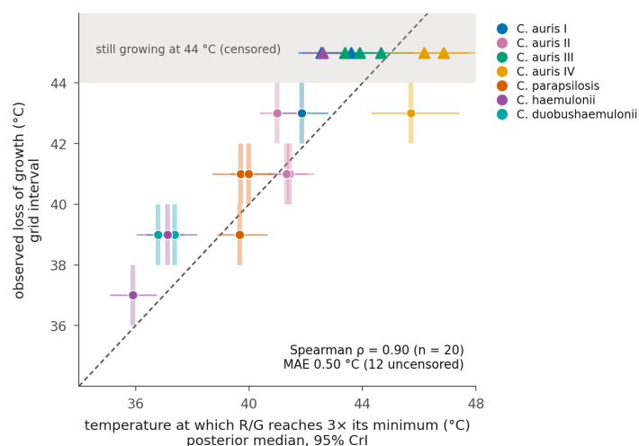
Supplementary Figure 12. The 3 \times crossing of the respiration-to-growth ratio tracks the growth limit isolate by isolate. Each point is one isolate: the temperature at which its respiration per unit growth reaches three times its own minimum (posterior median and 95% CrI from the isolate's own curve in the hierarchical
