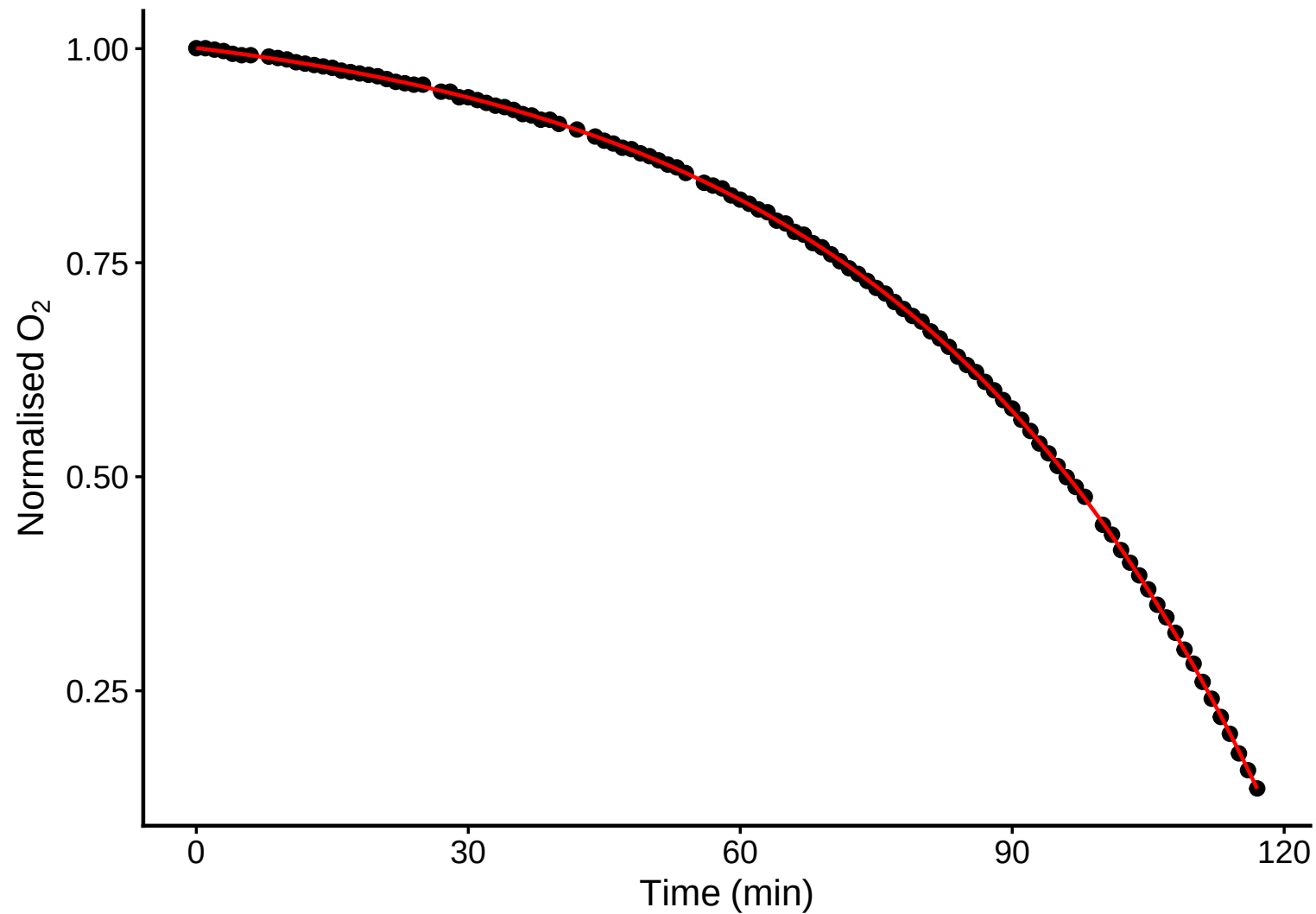
Flavobacterium_A_R3
