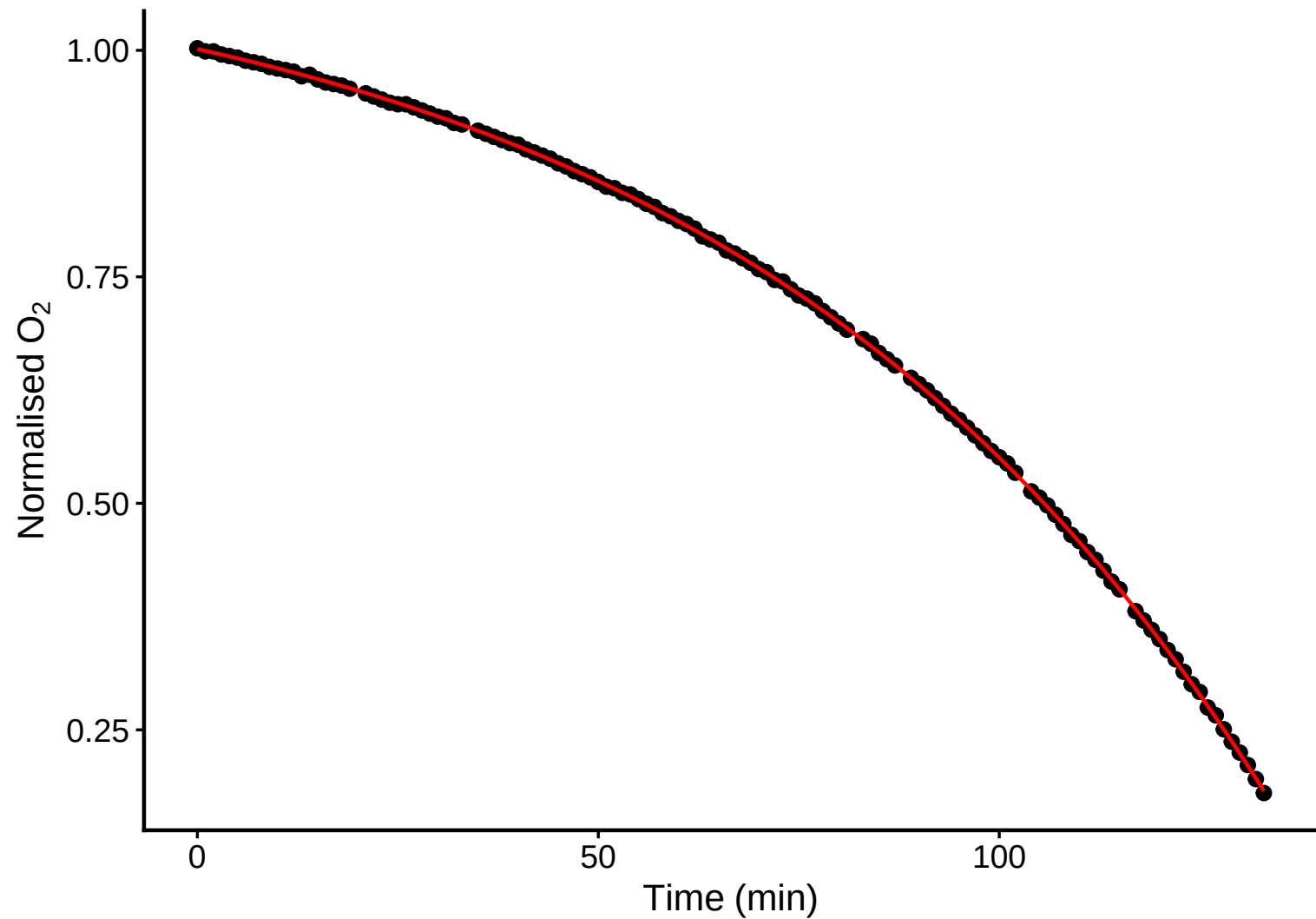
Flavobacterium_B_R2
